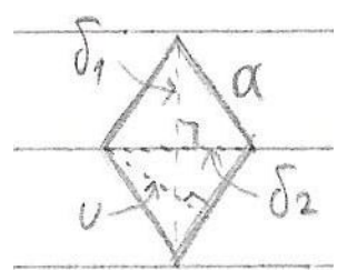
Figure 15: Ρόμβος
