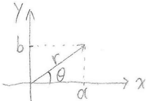
Figure 27: Argand Diagram
