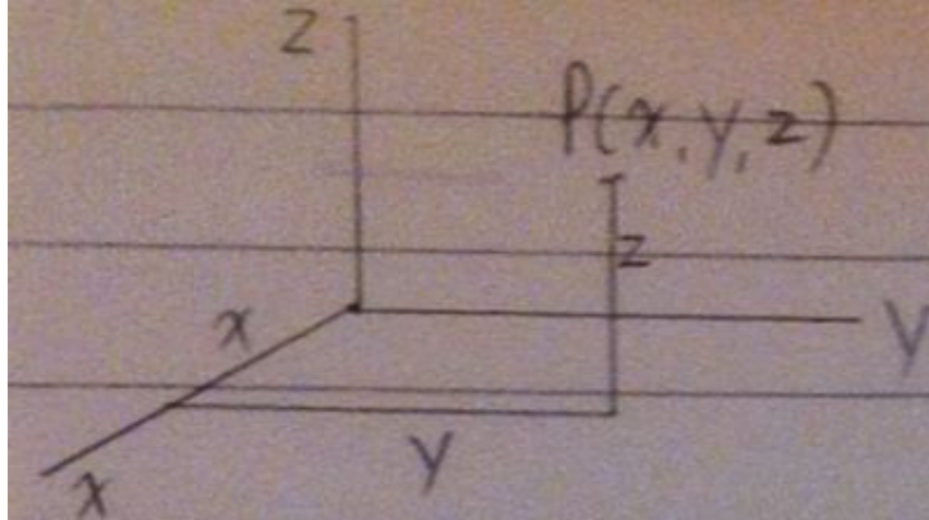
Figure 36: 3-Dimensional Coordinate System
