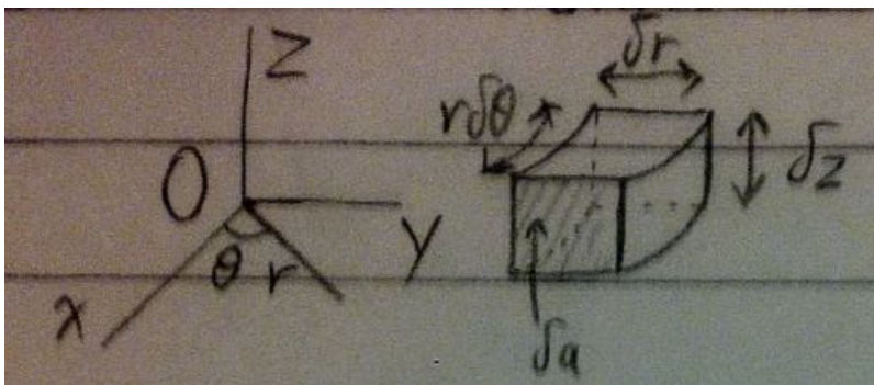
Figure 41: Element of Volume in Cylindrical Coordinates
