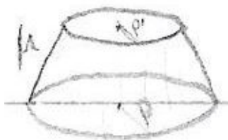
Figure 23: Κόλουρος κώνος
