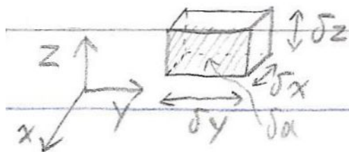
Figure 40: Element of Volume in Cartesian Coordinates
