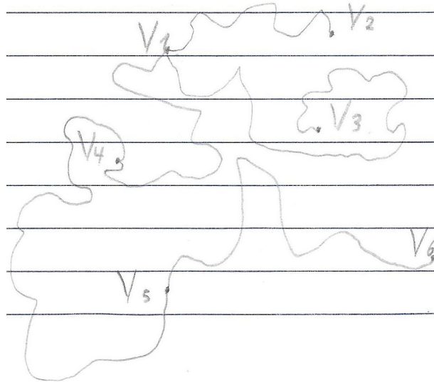
Figure 2: Graph G'
