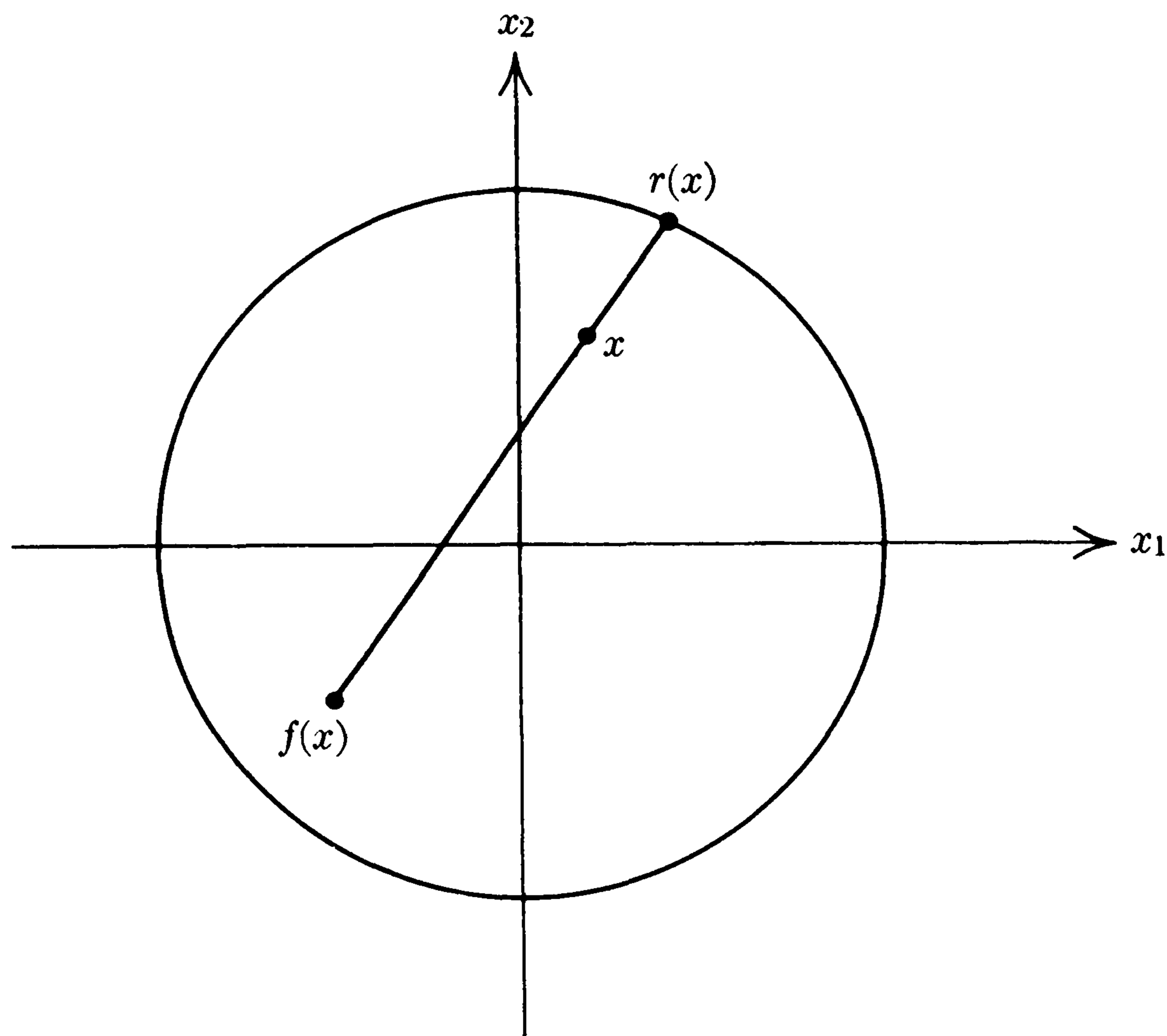
FIGURE 2.5 Proof of the Brouwer Fixed-Point Theorem.
