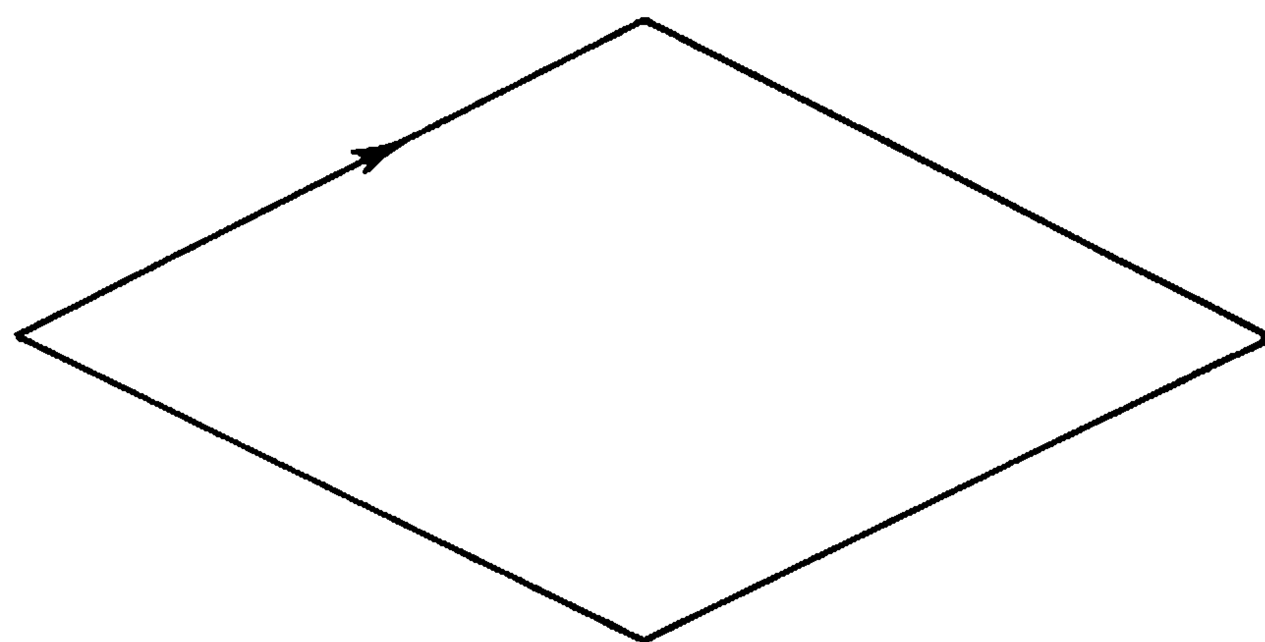
Figure 46. \pi(R^3 - K) = | \mathbf{x} : |
