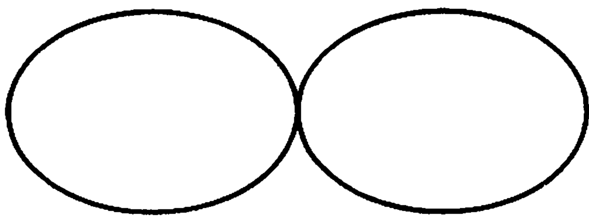
Ellipses with one point in common
