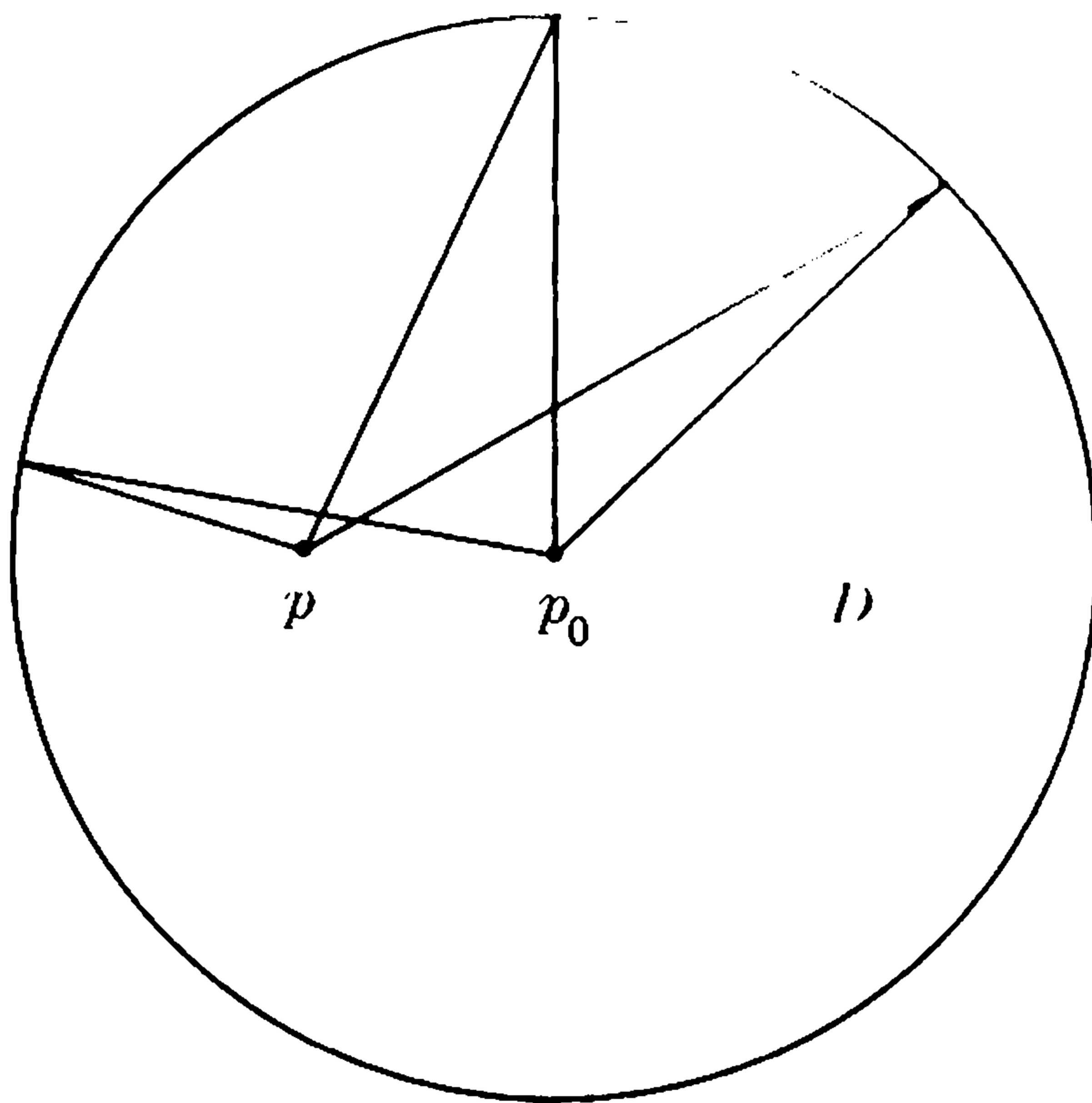
Figure 64. Perpendicular cross section of a cone
