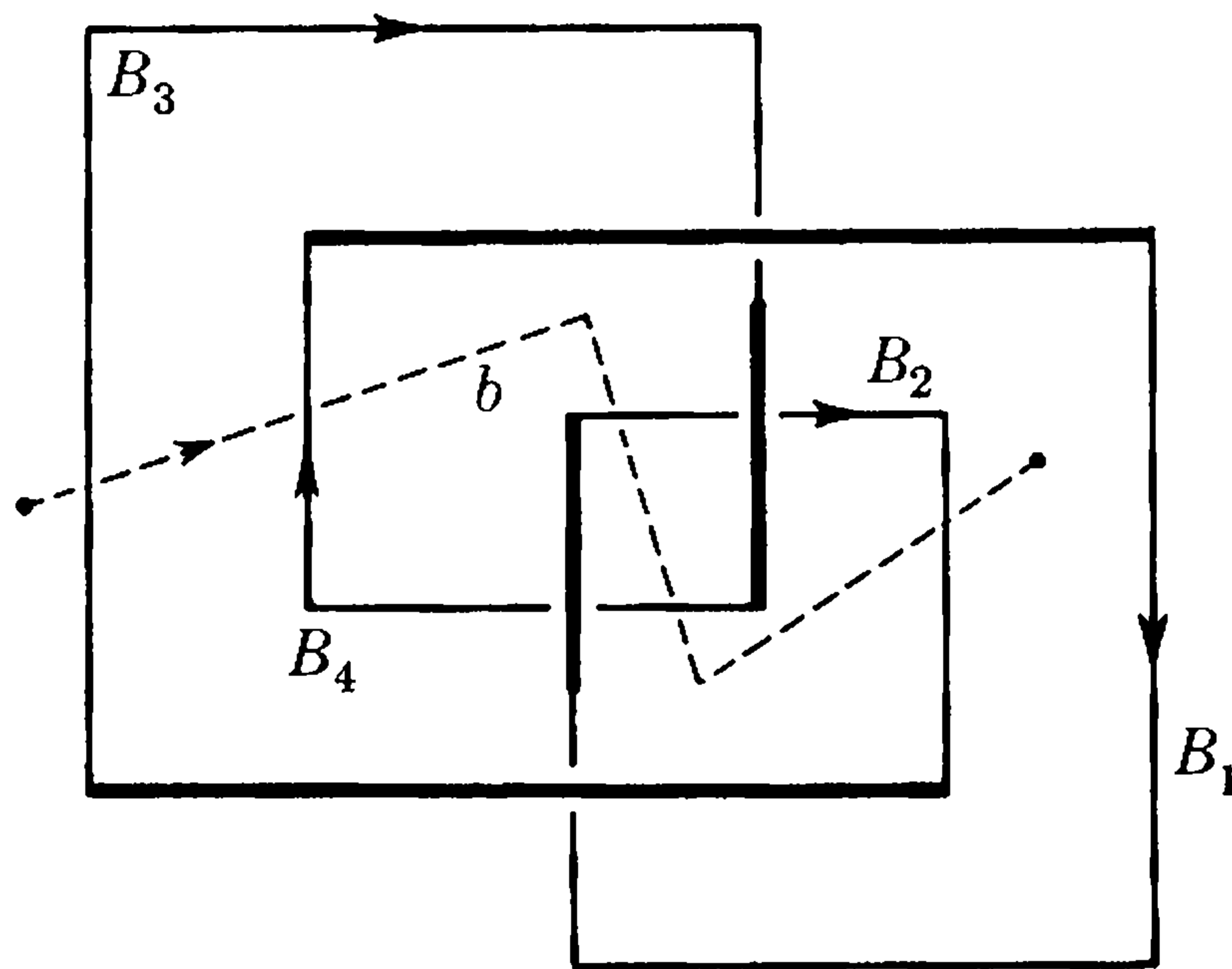
Figure 30 b^b = y_3 y_4 y_2 y_4^{-1} y_2^{-1}
