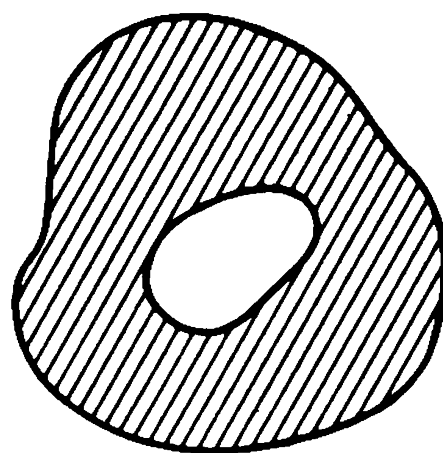
Plane annular region
