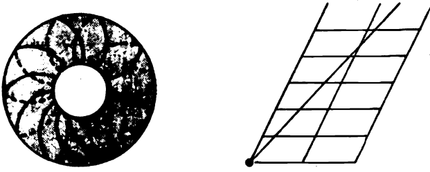
Figure 11. A torus and a part of its universal covering surface. A straight line projects on a spiral.
