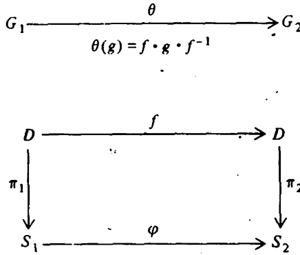
Figure 8. Mappings induced by a homeomorphic \varphi .
