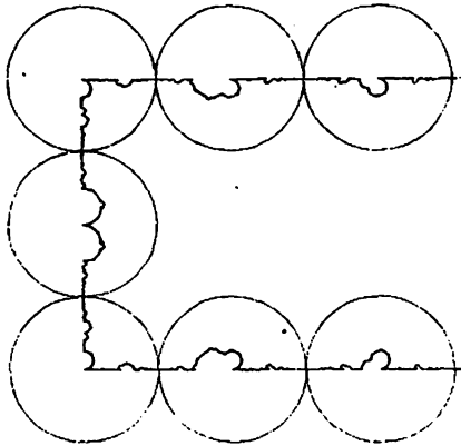
Figure 13. Invariant Jordan domain which is not a quasidisc.
