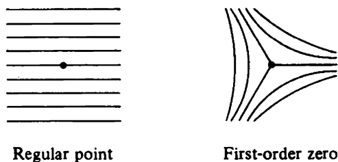
Figure 10. Horizontal trajectories under natural parameters.
