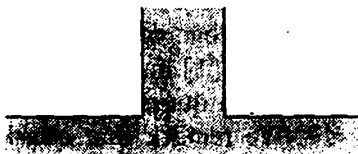
Figure 1. Strebel's chimney.
