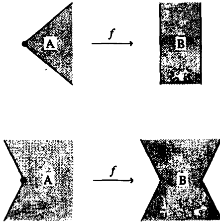
Figure 7. S_f \in \partial T_A(1) closest to the origin.
