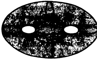
Figure 12. Horizontal trajectories on a surface of genus 2. 4p - 4 = 4 critical points.
