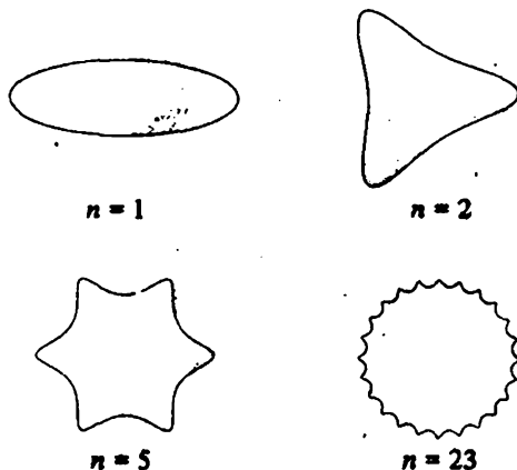
Figure 5. Extremal domains for k = \frac{1}{2} .
