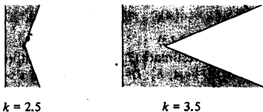
Figure 4. Extremal domains.
