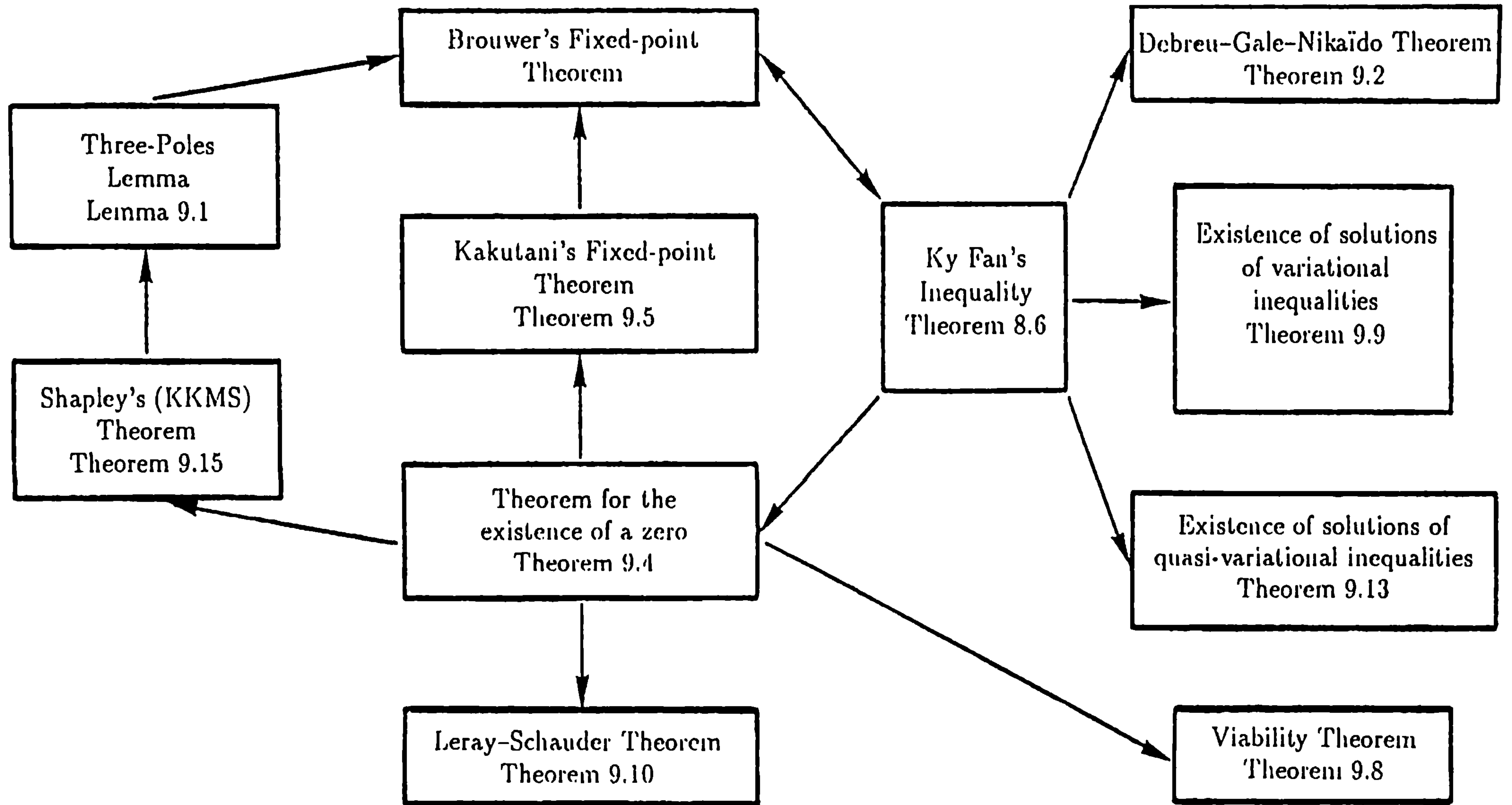
Fig. 9.3 Relationships between the main theorems of nonlinear analysis
