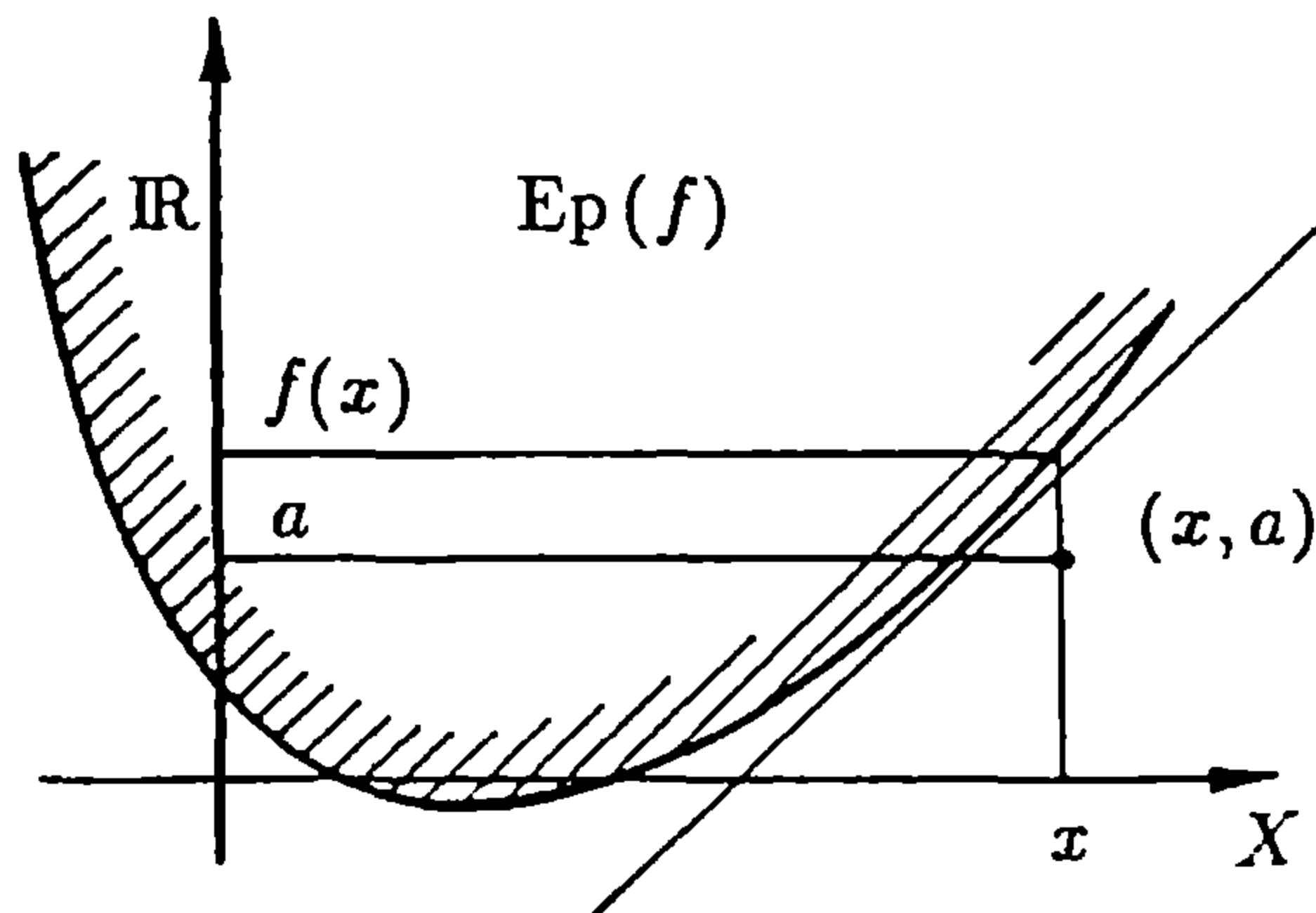
Fig. 3.1. Graph of an affine function minorising f .
