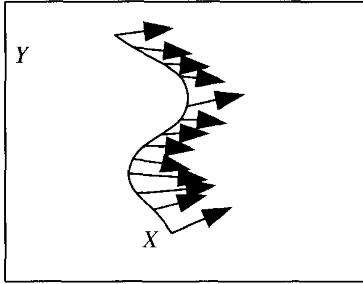
FIGURE 6.9. A normal vector field.
