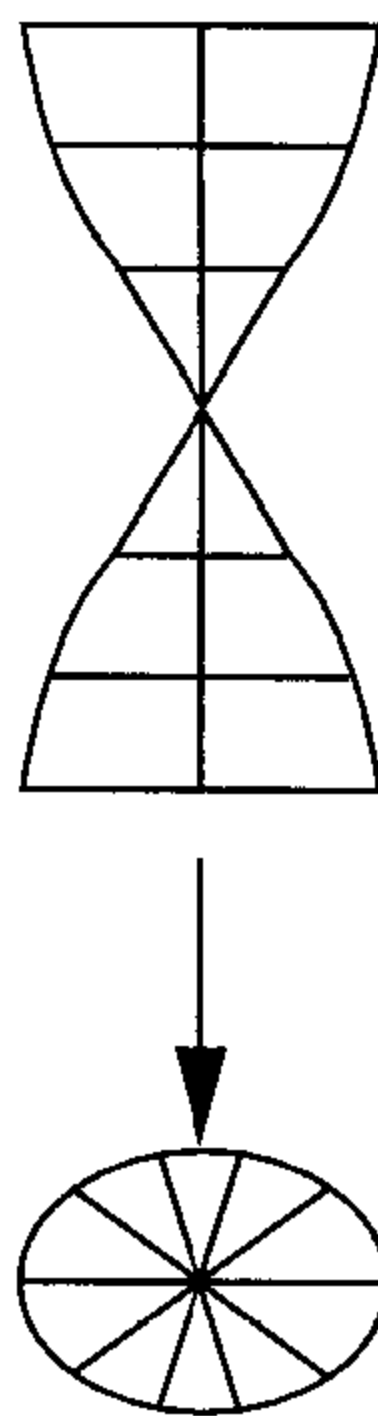
FIGURE 6.8. Blowup of a point in the plane.
