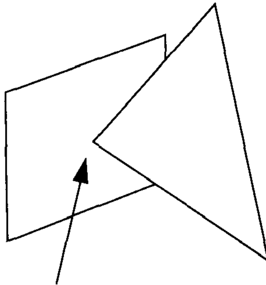
Not Cohen-Macaulay here.
