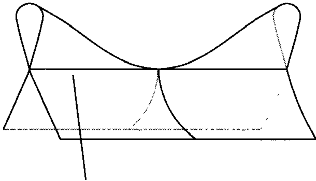
The singular locus is x = y = 0 , a line parametrized by t .
