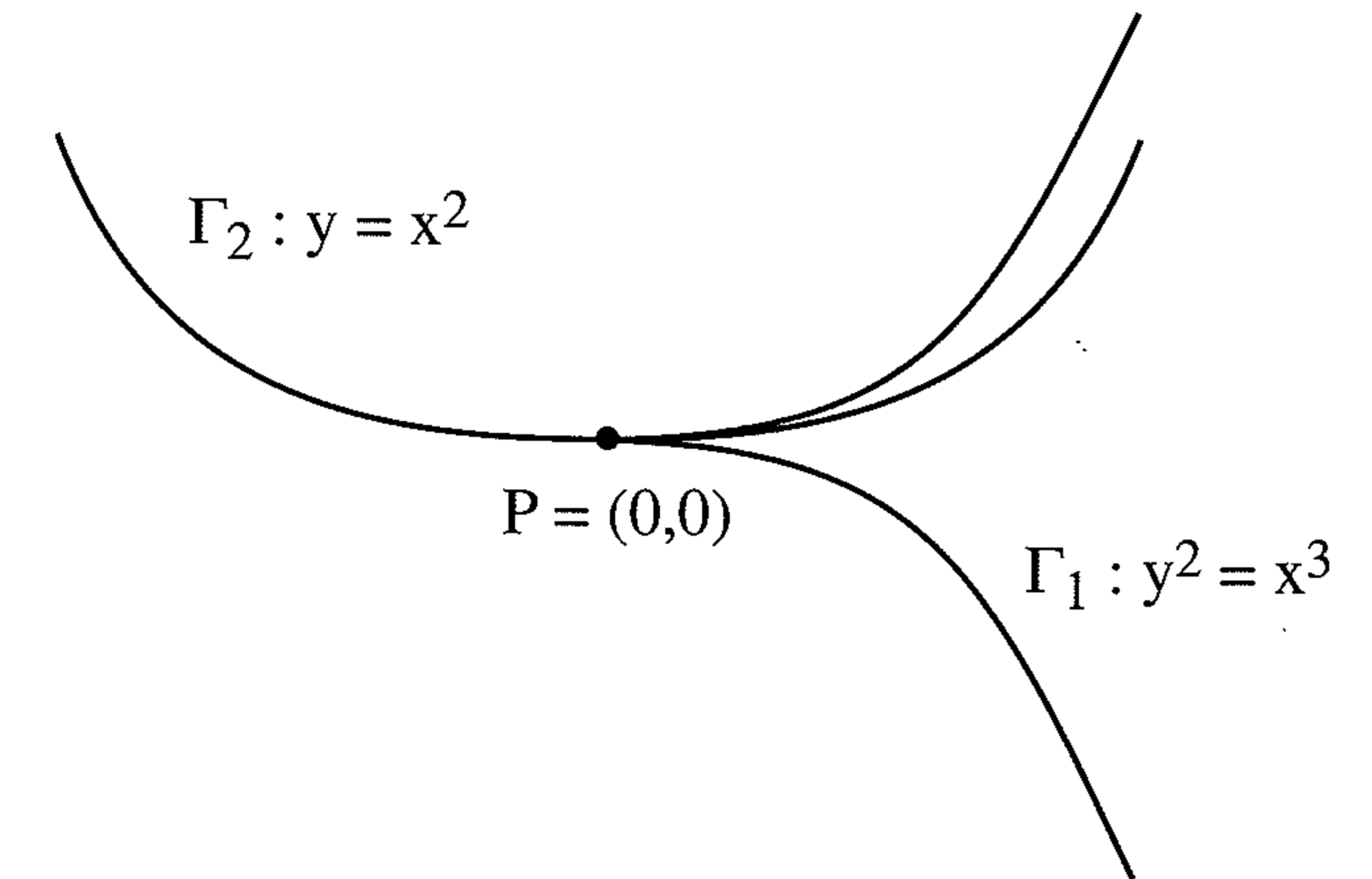
The Curves \Gamma_1 : y^2 = x^3 and \Gamma_2 : y = x^2 Near P = (0,0)
