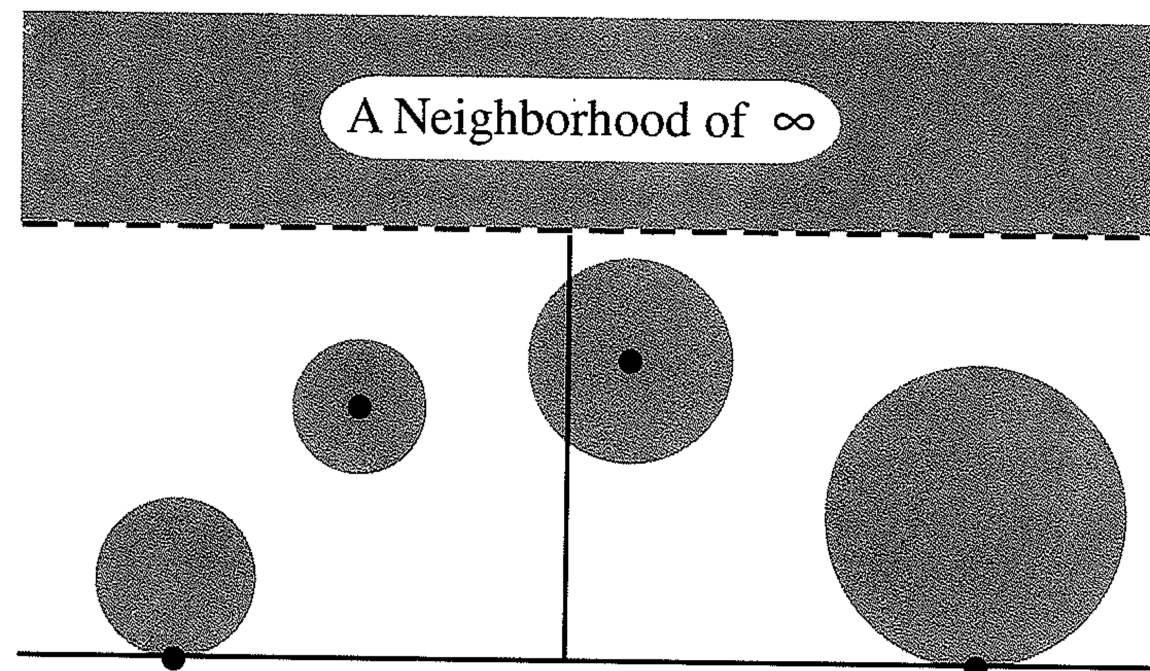
Some Open Sets in \mathbf{H}^*
