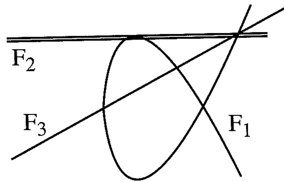
The Special Fiber \mathcal{C}_5 : (y^2 - x^3 - 3x^2)(y - 2)^2(2y - x - 3) = 0
