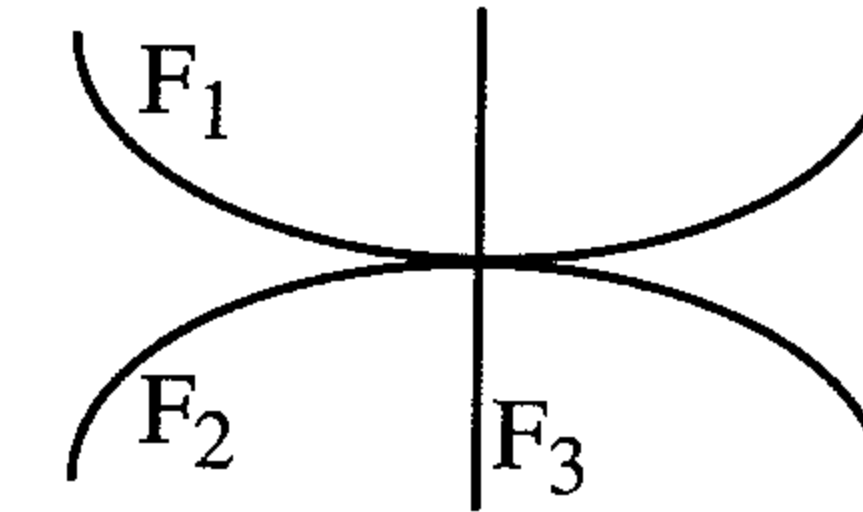
The Special Fiber \tilde{\mathcal{S}} of the Scheme \mathcal{S} : X^2 + Y = T^4 , \pi = TY
