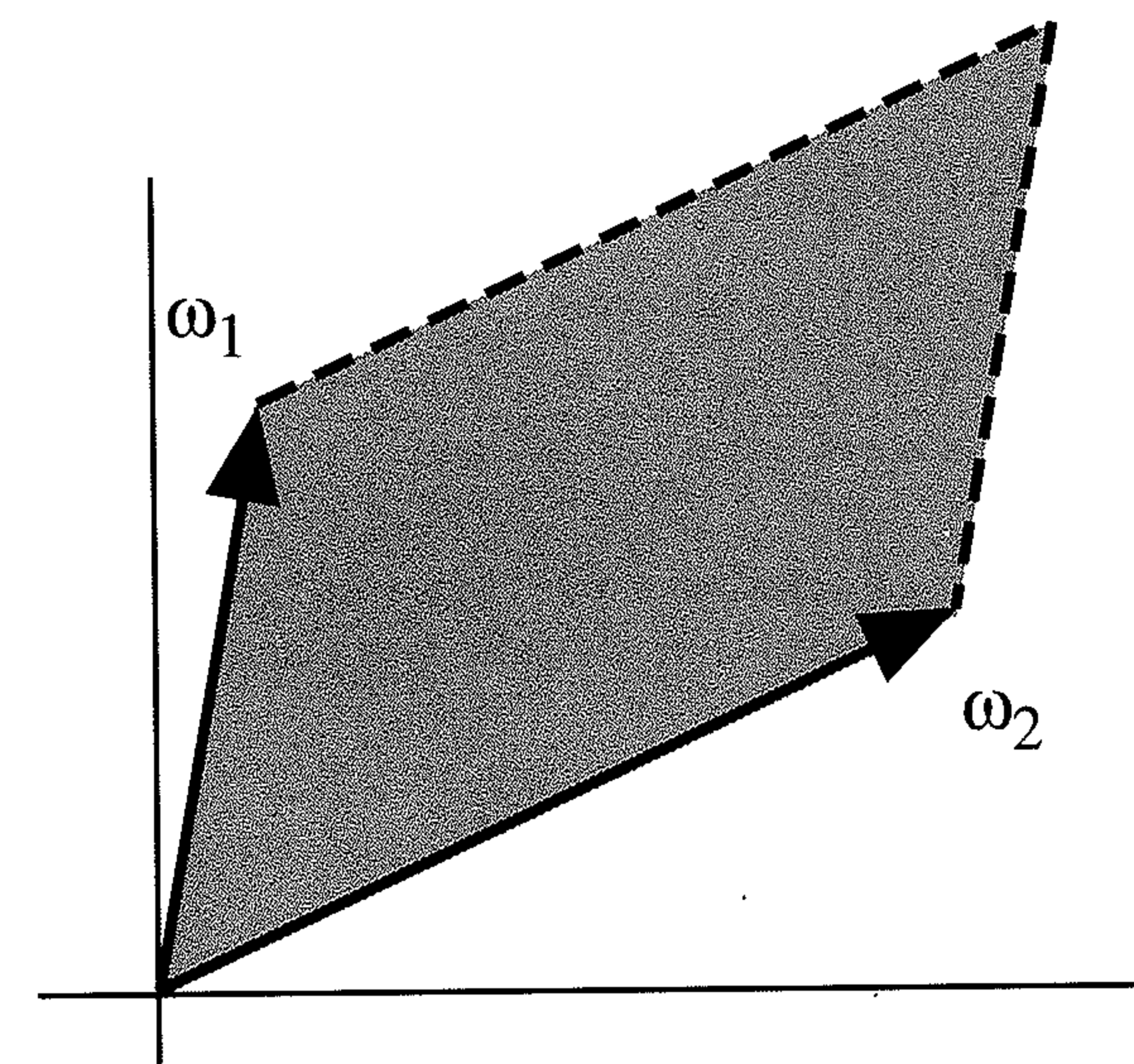
An Oriented Basis for the Lattice \Lambda
