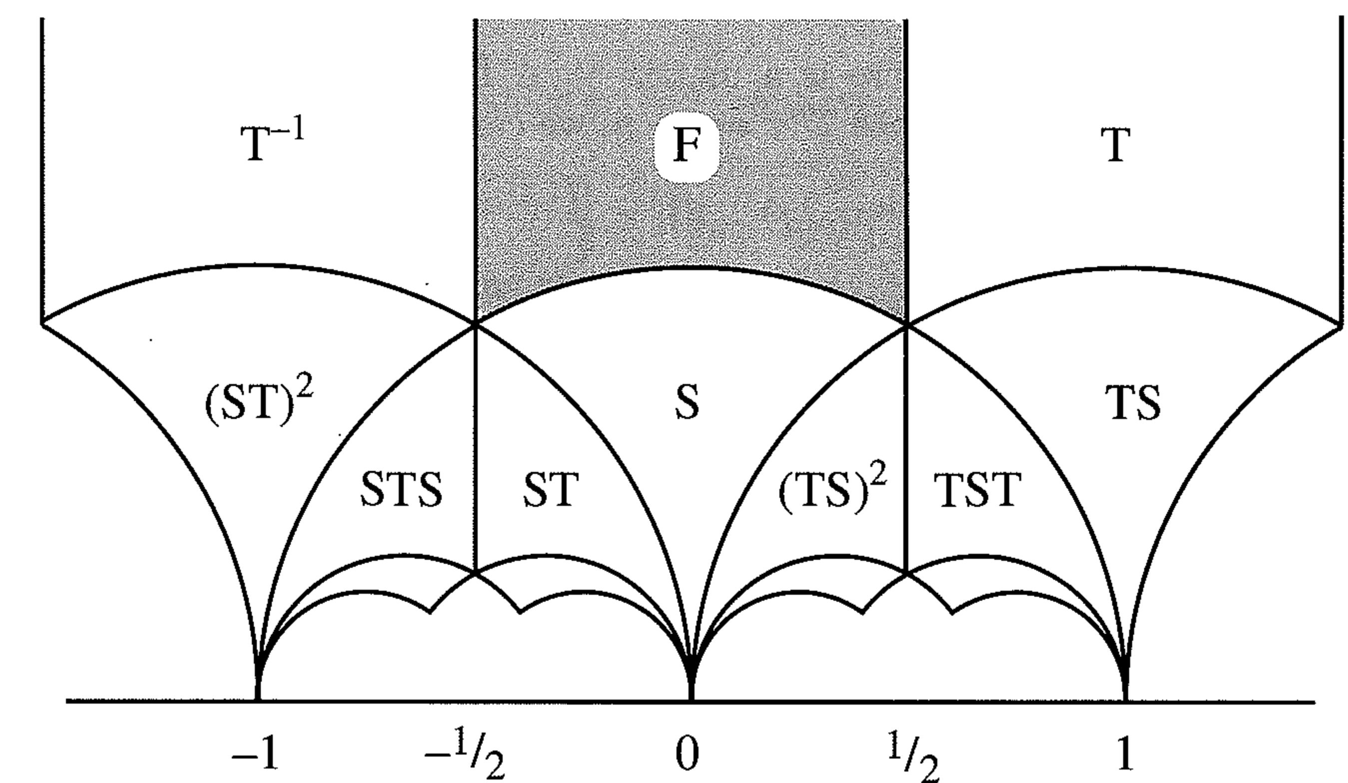
\mathcal{F} and Some of Its \Gamma(1) -Translates
