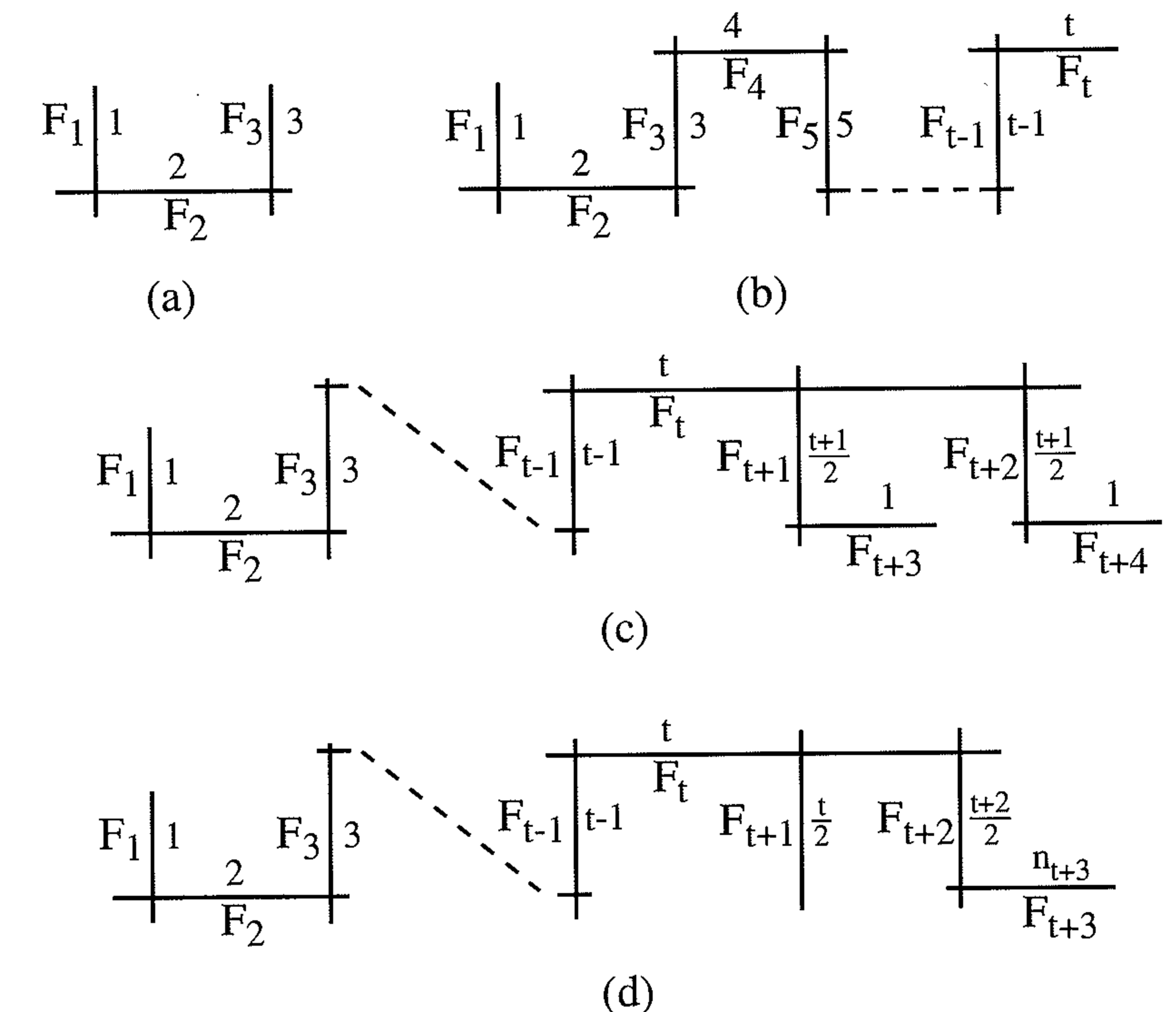
Building Fibers of Type IV^* , III^* , II^*
