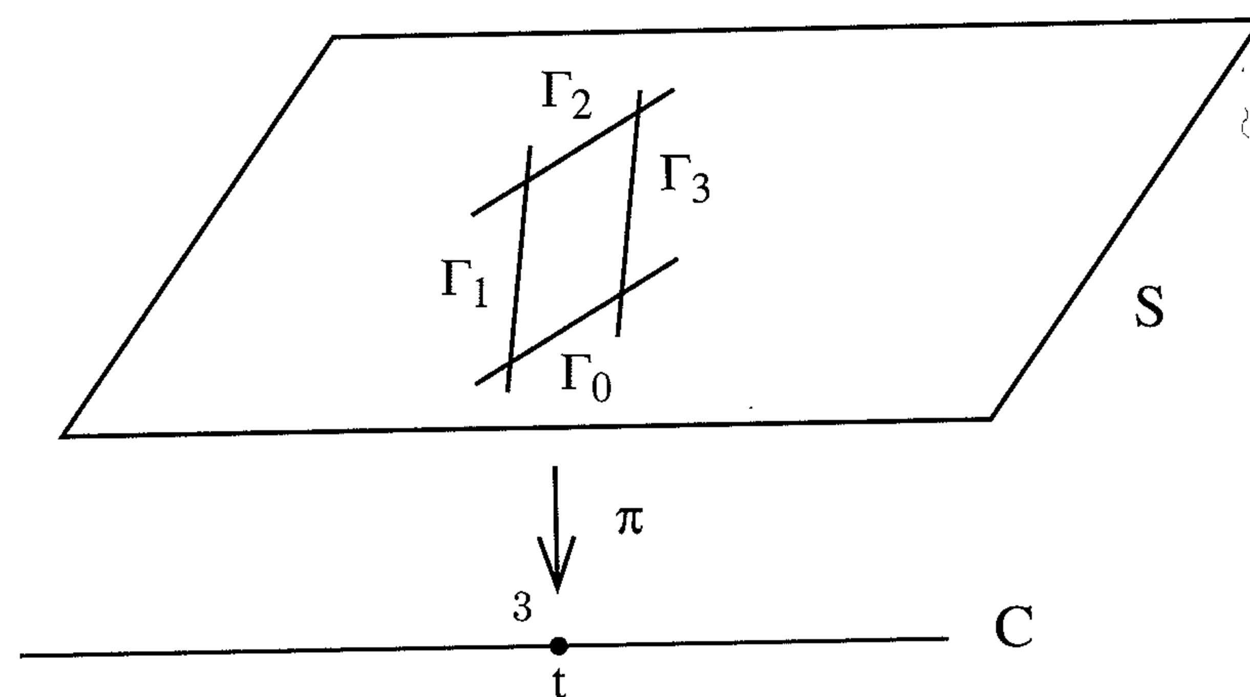
A Reducible Fiber on a Fibered Surface
