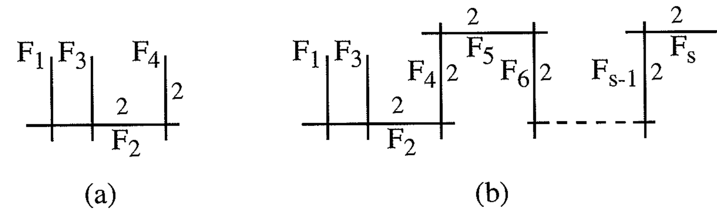
Building a Fiber of Type I_n^*
