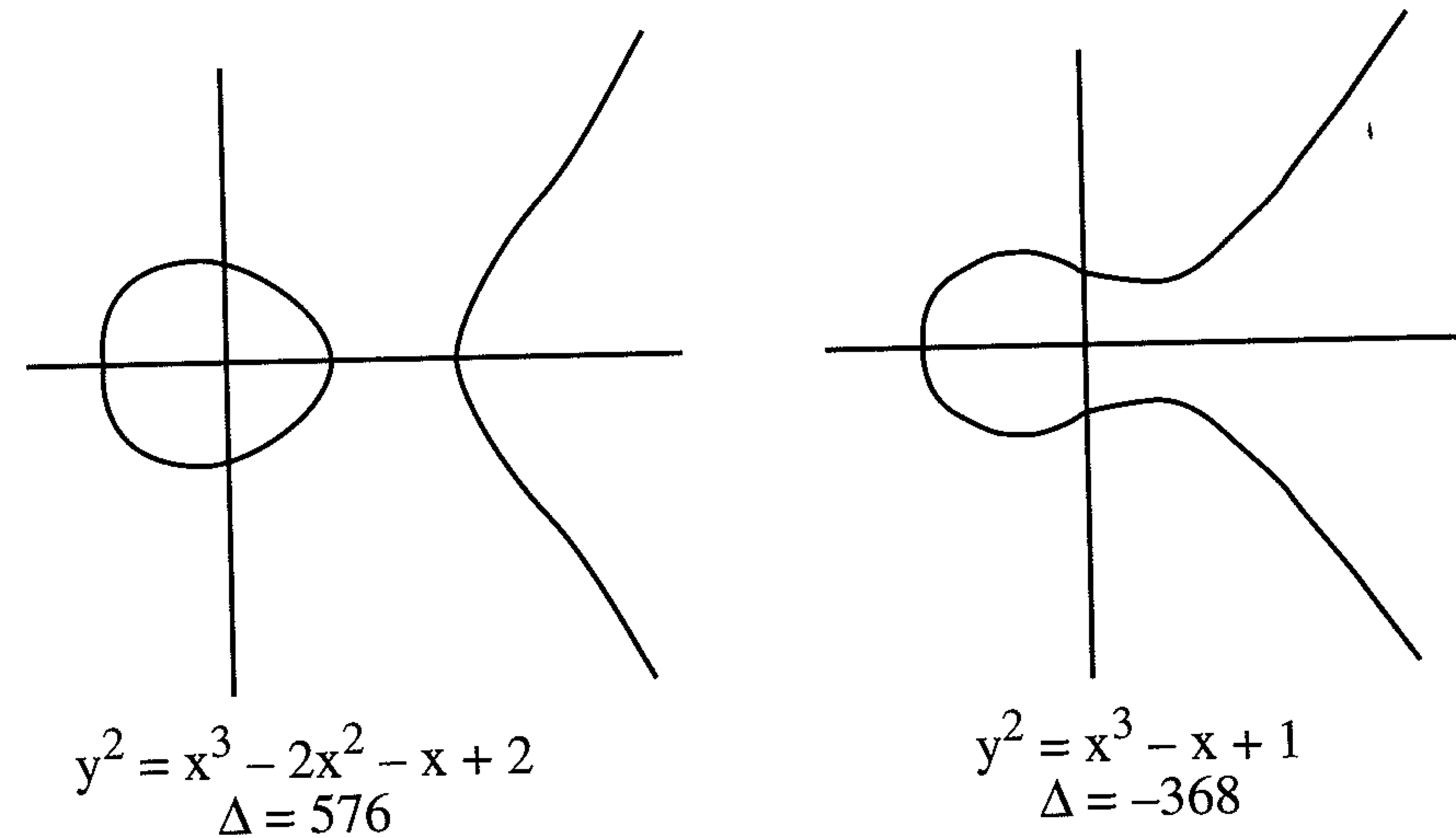
Elliptic Curves over \mathbb{R} with One and Two Components
