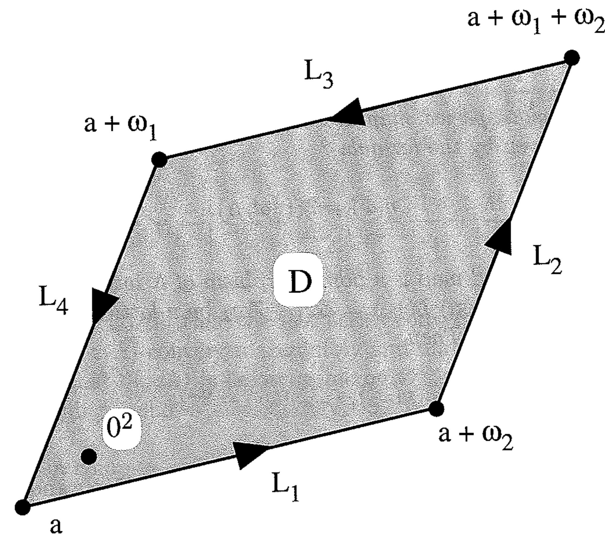
An Offset Fundamental Domain for \mathbb{C}/\Lambda
