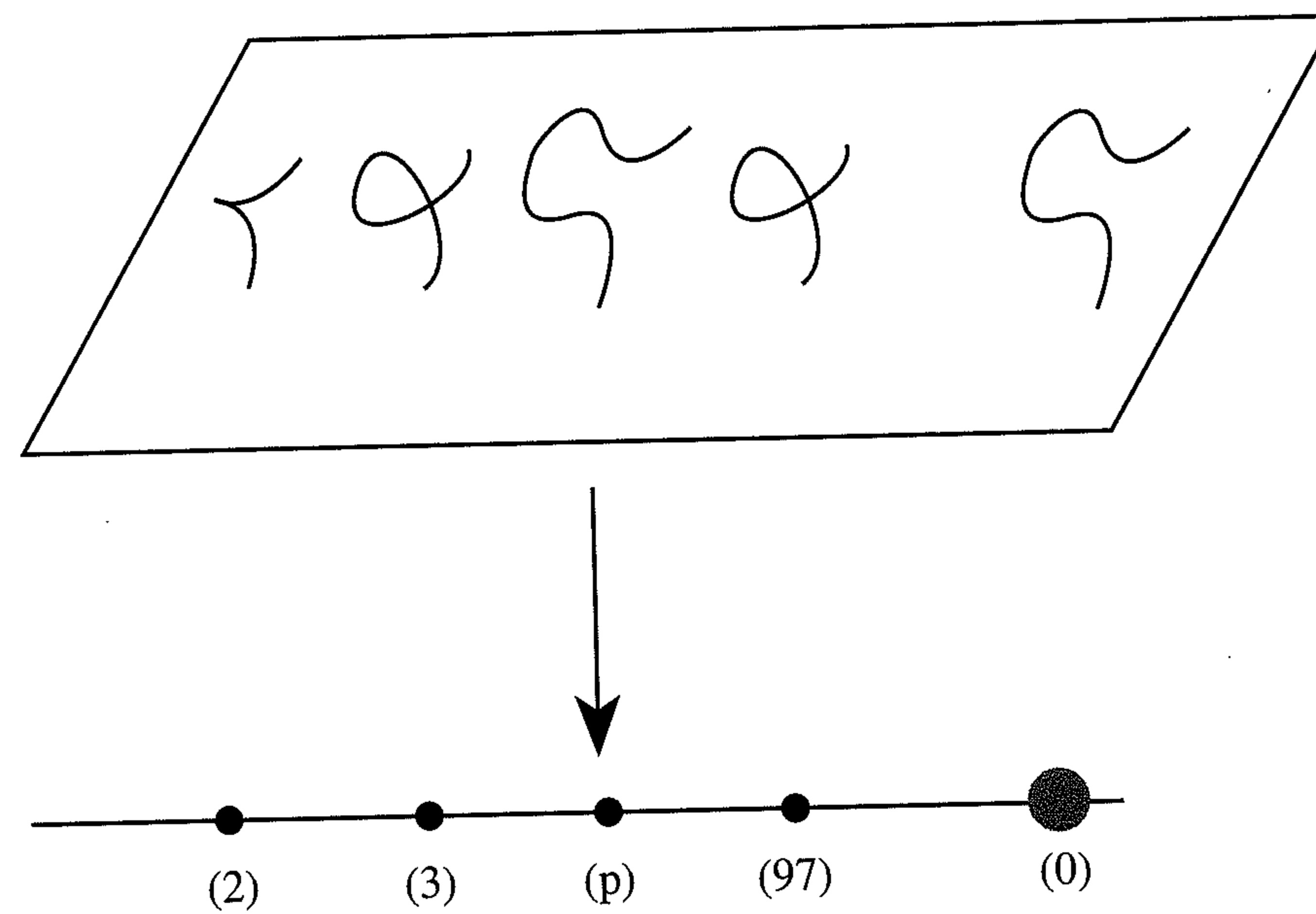
The Arithmetic Surface \mathcal{C} : y^2 = x^3 + 2x^2 + 6 over \text{Spec}(\mathbb{Z})
