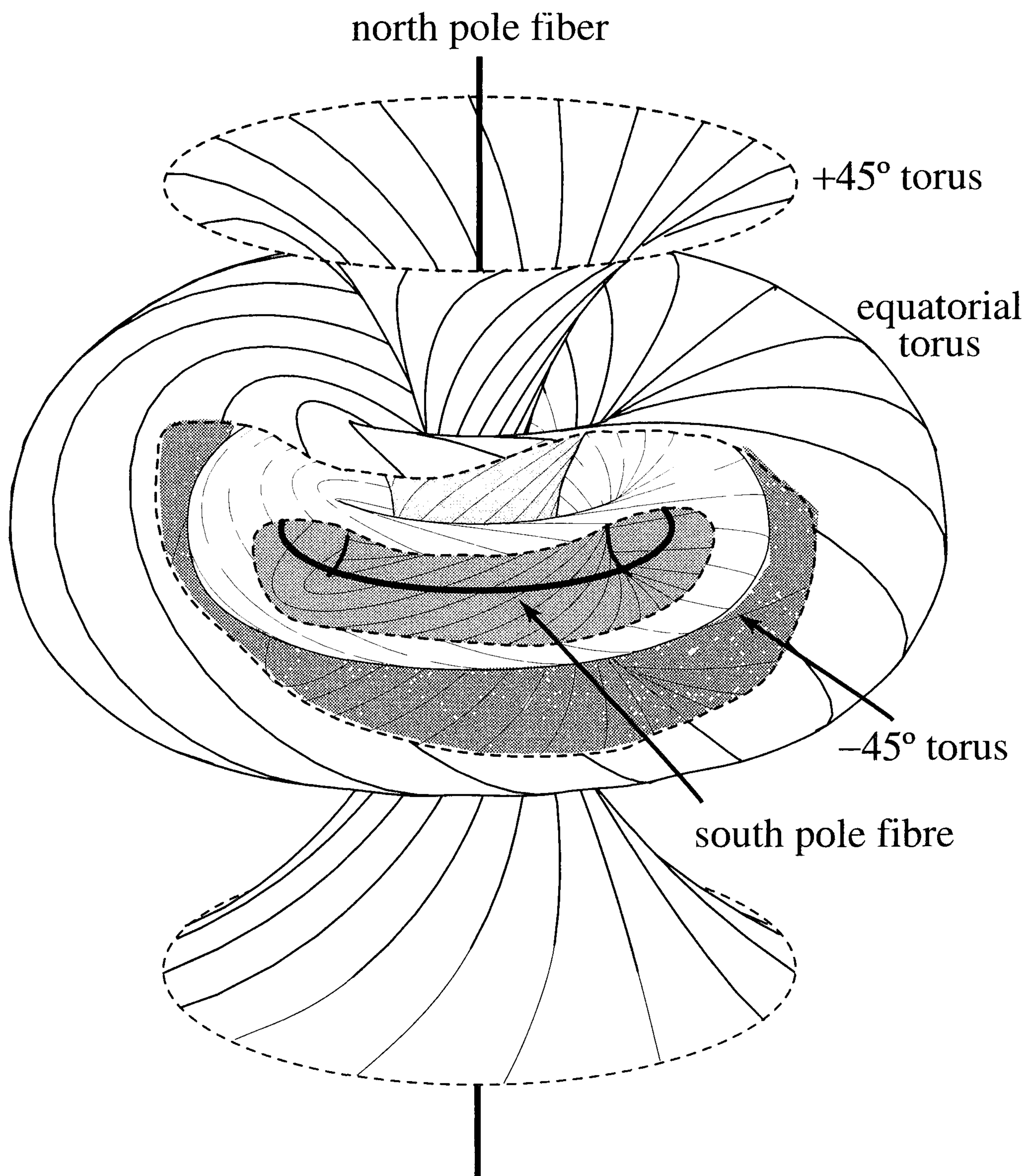
FIGURE 3.15. The Hopf fibration.
