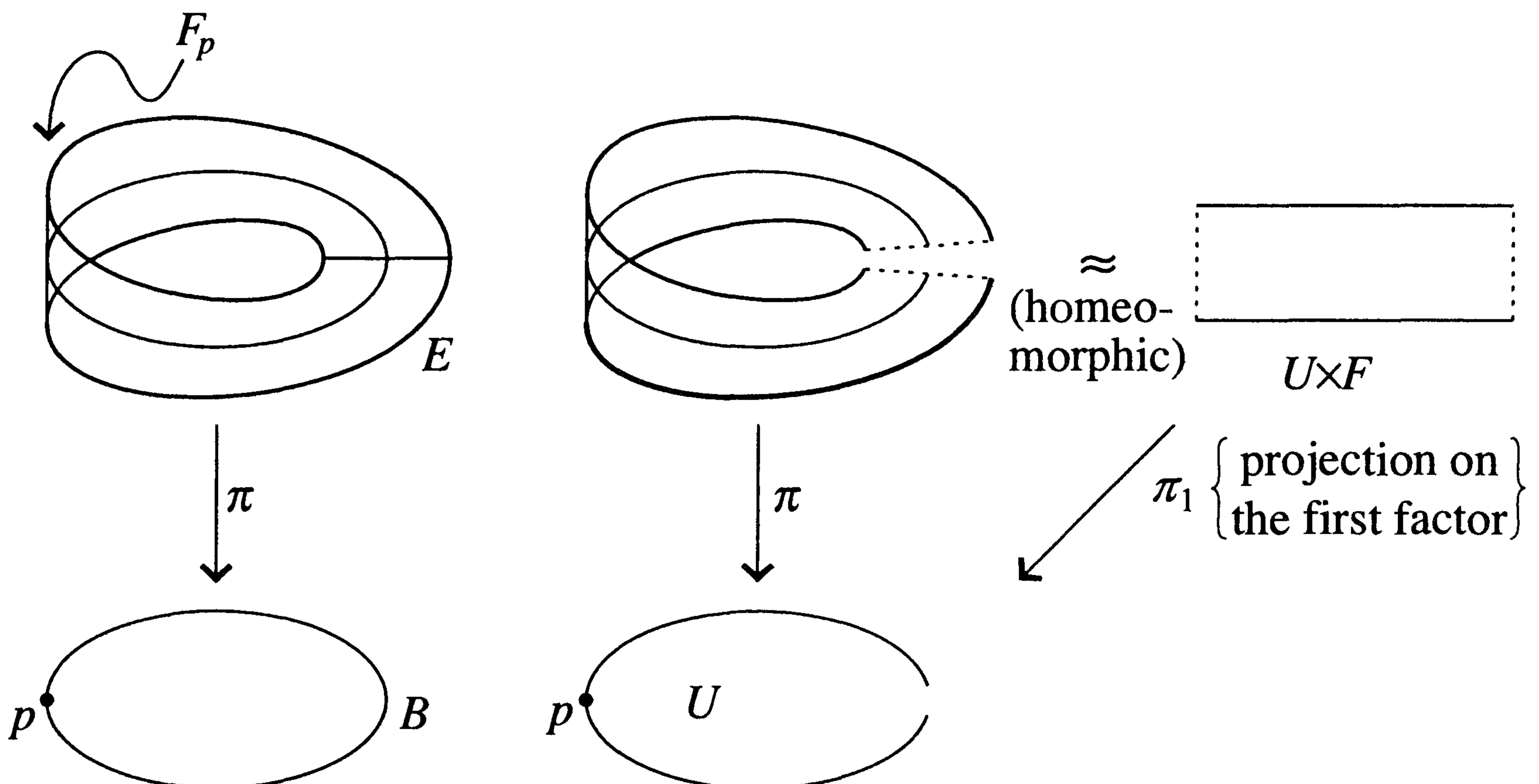
FIGURE 3.4. Möbius band.
