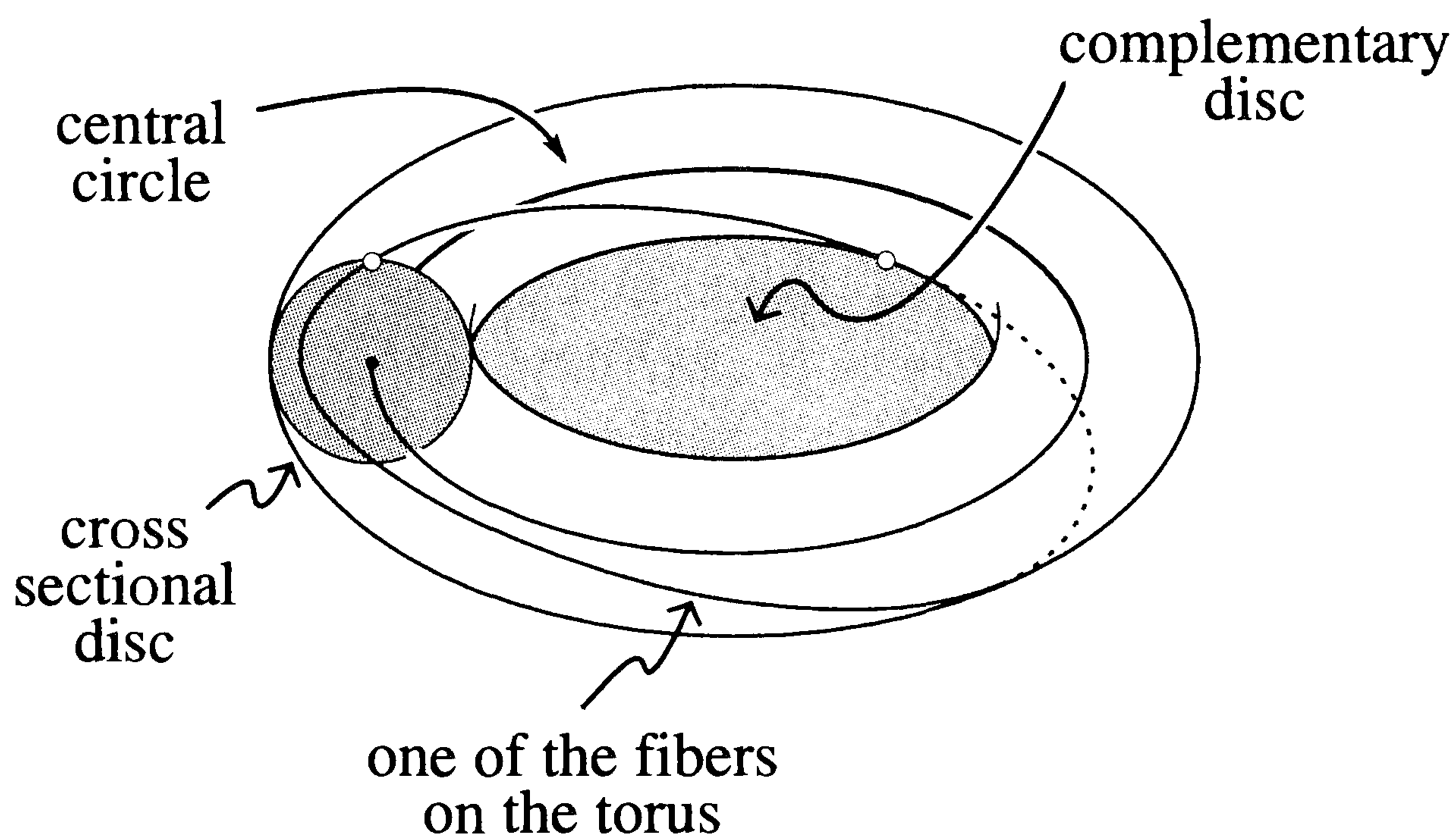
FIGURE 3.16. Topology of the space of fibers.
