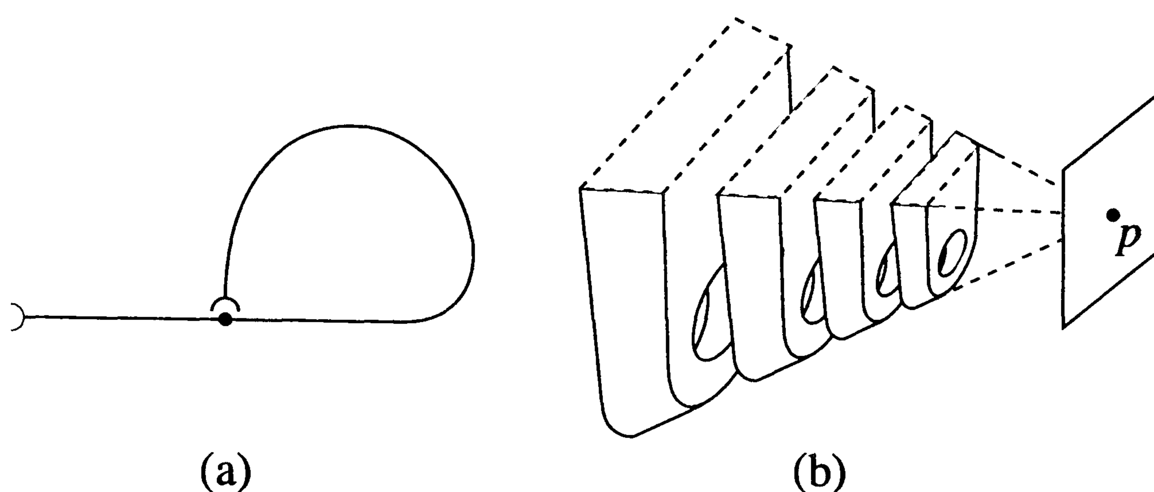
FIGURE 2.3. Odd limit points.
