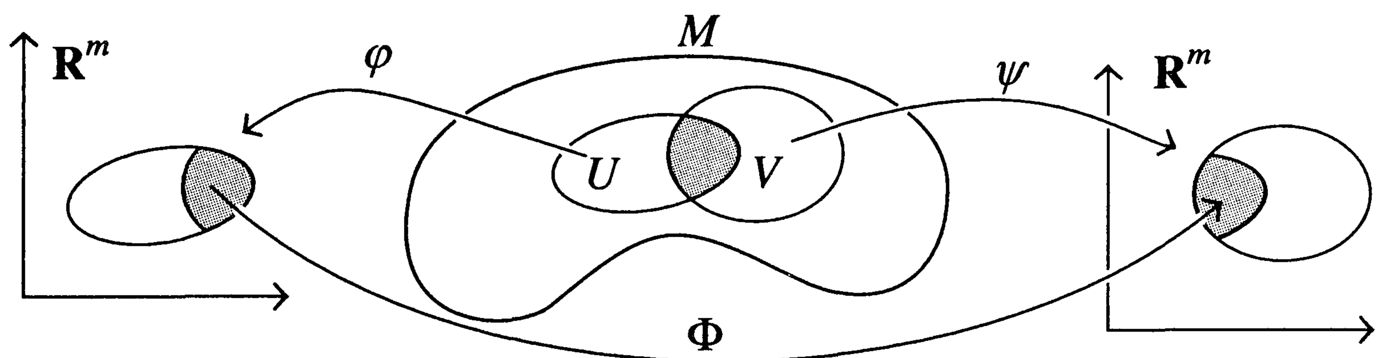
FIGURE 1.6. Change of coordinate system.
