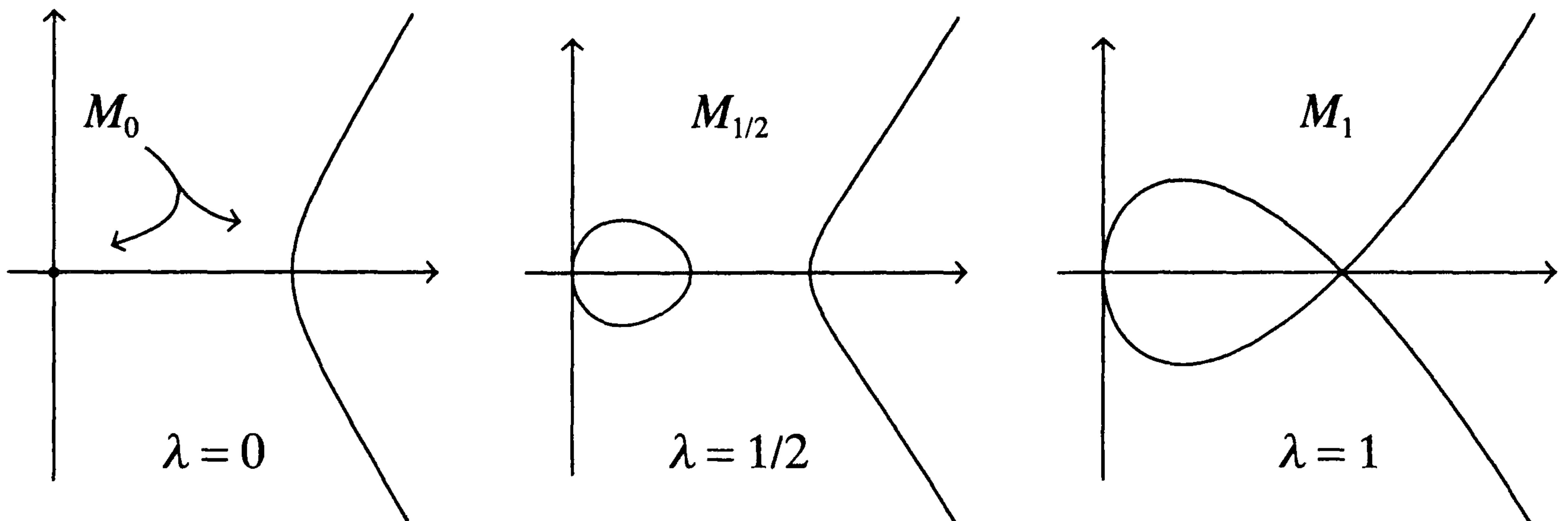
FIGURE 2.15. Various elliptic curves.
