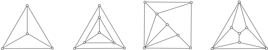
Fig. 10.14. Self-dual plane graphs
