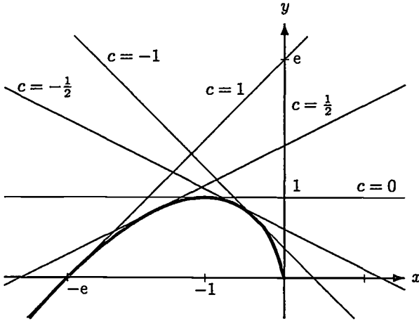
Solution curves of Clairaut's equation y = xy' + e^{y'}
