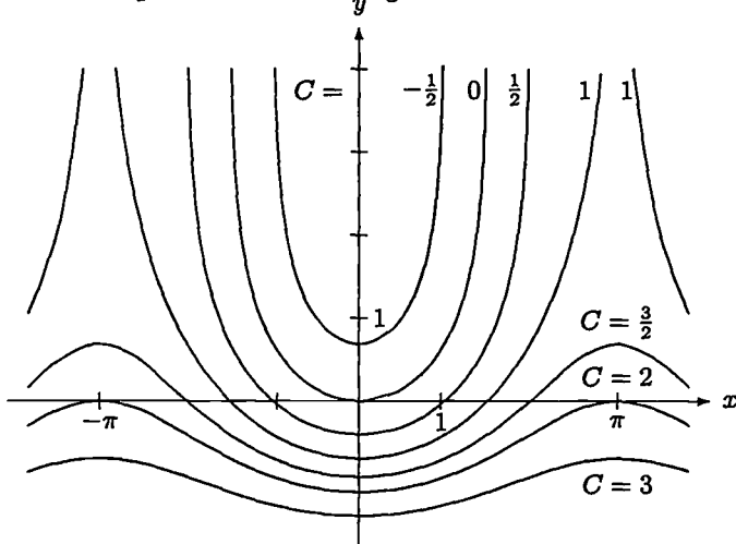
Solution curves of the differential equation y' = e^y \sin x
