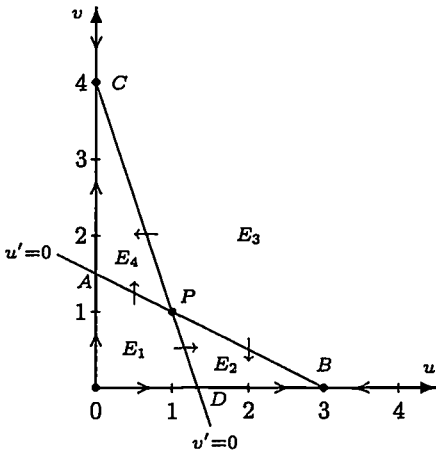
Nullclines: u' = f = 0, v' = g = 0
