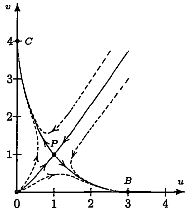
Phase Portrait
