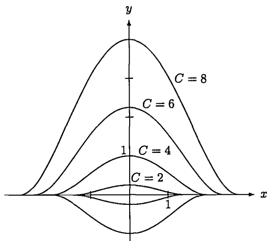
Solution curves of the differential equation y' = -x(\operatorname{sgn} y)\sqrt{|y|}
