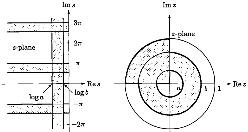
The mapping s = \log z
