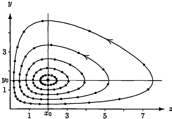
The predator-prey model with (a, b, c, d) = (3, 2, 2, 1) , (x_0, y_0) = (2, \frac{3}{2})
