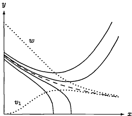
Example 1 with v_1 = 1/(x + x^{-2}) , w as in the text (the dashed curve is \phi )
