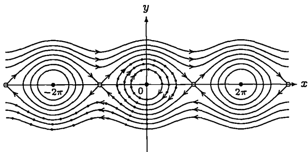
Mathematical pendulum
