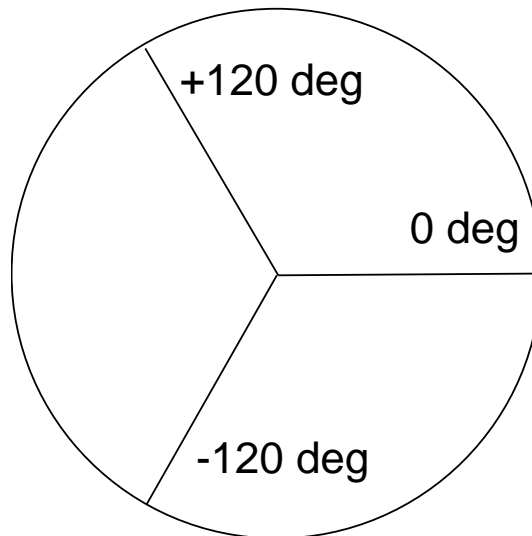
Figure 2-5 The n roots of 1^{1/n} on the unit circle
