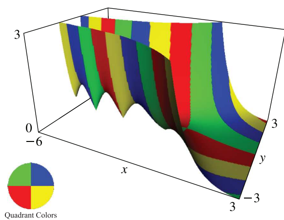
Figure 9.3.5: Ai'(x + iy) .
