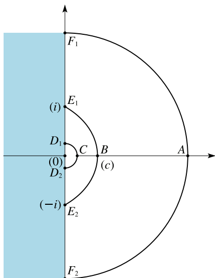
Figure 10.41.1: z -plane.
