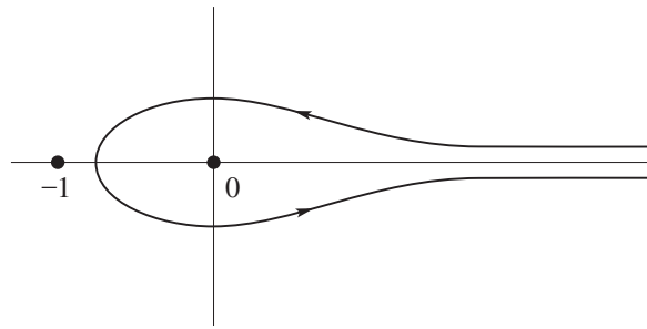
Figure 5.12.2: t -plane. Contour for second loop integral for the beta function.
