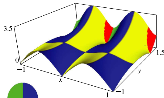
Figure 20.3.17: \theta_4(\pi x + iy, 0.12) , -1 \leq x \leq 1 , -1 \leq y \leq 1.5 .
