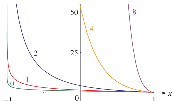
Figure 14.20.3: P_{-\frac{1}{2}+i\tau}^{-1/2}(x), \tau = 0, 1, 2, 4, 8.
