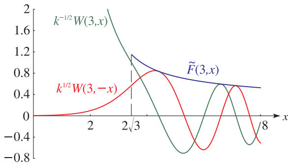
Figure 12.14.1: k^{-1/2} W(3, x) , k^{1/2} W(3, -x) , \tilde{F}(3, x) , 0 \leq x \leq 8 .
