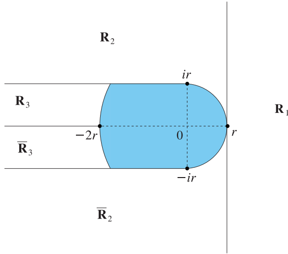
Figure 13.7.1: Regions \mathbf{R}_1 , \mathbf{R}_2 , \overline{\mathbf{R}}_2 , \mathbf{R}_3 , and \overline{\mathbf{R}}_3 are the closures of the indicated unshaded regions bounded by the straight lines and circular arcs centered at the origin, with r = |b - 2a| .
