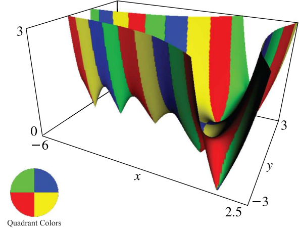
Figure 9.3.6: Bi'(x + iy) .
