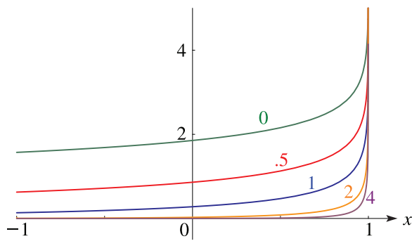
Figure 14.20.2: \hat{Q}_{-\frac{1}{2}+i\tau}^0(x), \tau = 0, \frac{1}{2}, 1, 2, 4.
