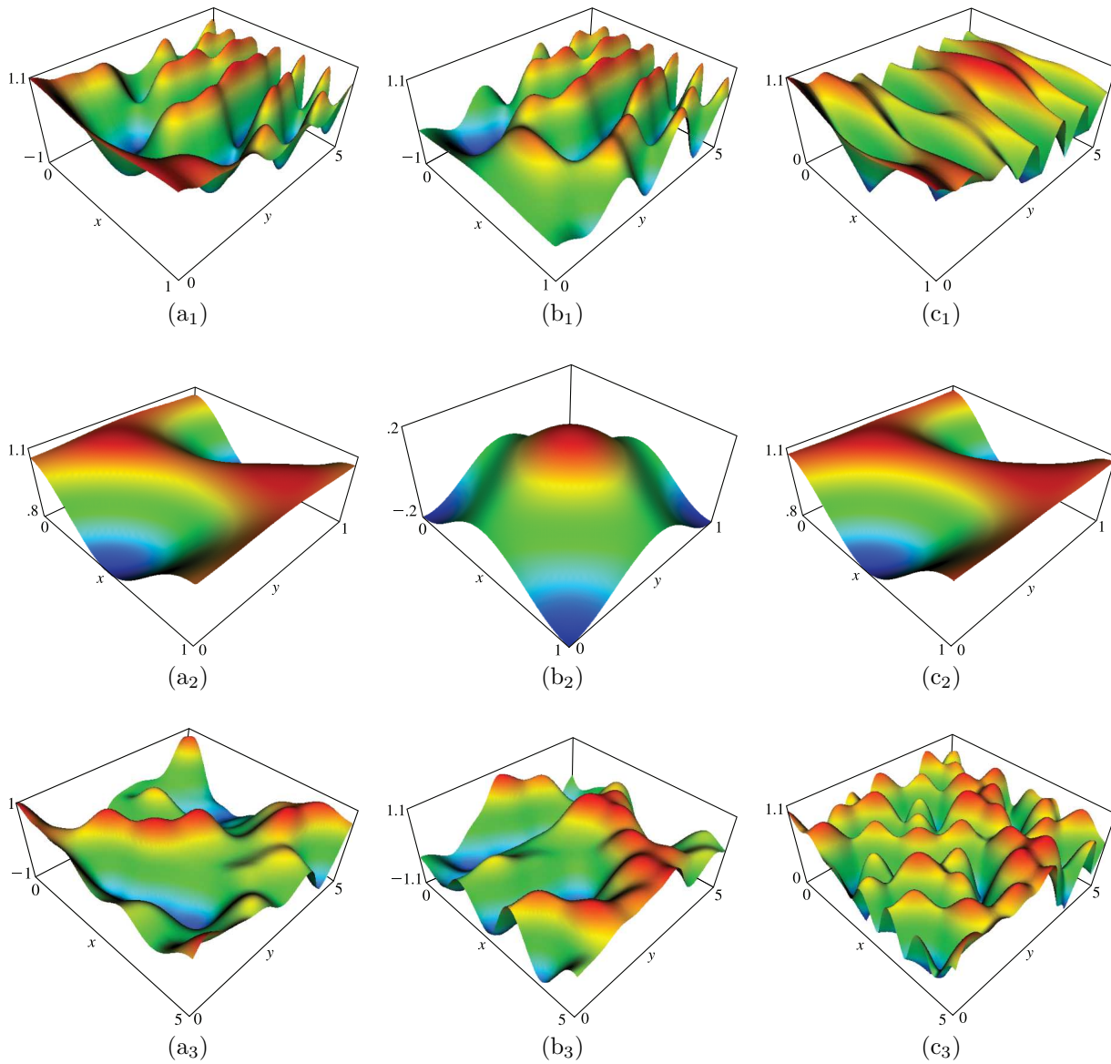
Figure 21.4.1: \hat{\theta}(\mathbf{z}|\Omega) parametrized by (21.4.1). The surface plots are of \hat{\theta}(x + iy, 0|\Omega) , 0 \leq x \leq 1 , 0 \leq y \leq 5 (suffix 1); \hat{\theta}(x, y|\Omega) , 0 \leq x \leq 1 , 0 \leq y \leq 1 (suffix 2); \hat{\theta}(ix, iy|\Omega) , 0 \leq x \leq 5 , 0 \leq y \leq 5 (suffix 3). Shown are the real part (a), the imaginary part (b), and the modulus (c).
