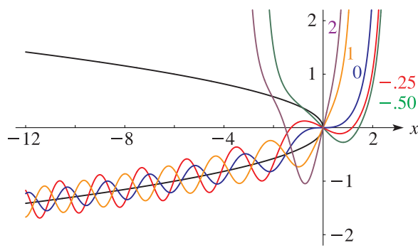
Figure 32.3.2: w_k(x) for -12 \leq x \leq 2.43 and k = -0.5, -0.25, 0, 1, 2 , and the parabola 6w^2 + x = 0 , shown in black.
