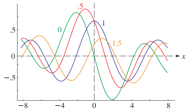
Figure 11.10.2: Weber function E_\nu(x) for -8 \leq x \leq 8 and \nu = 0, \frac{1}{2}, 1, \frac{3}{2} .
