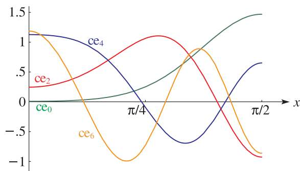
Figure 28.3.2: ce_{2n}(x, 10) for 0 \leq x \leq \pi/2 , n = 0, 1, 2, 3 .
