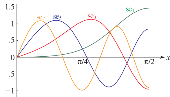
Figure 28.3.6: se_{2n+1}(x, 10) for 0 \leq x \leq \pi/2 , n = 0, 1, 2, 3 .
