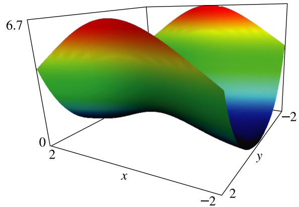
Figure 30.7.16: |Ps_0^0(x + iy, 4)| , -2 \leq x \leq 2 , -2 \leq y \leq 2 .
