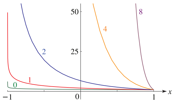
Figure 14.20.1: P_{-\frac{1}{2}+i\tau}^0(x), \tau = 0, 1, 2, 4, 8.
