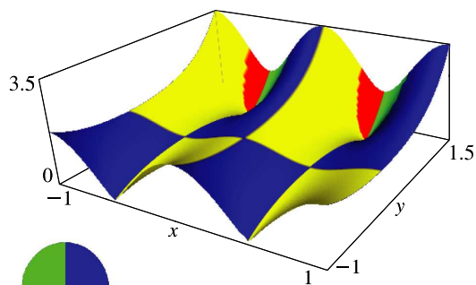
Figure 20.3.16: \theta_3(\pi x + iy, 0.12) , -1 \leq x \leq 1 , -1 \leq y \leq 1.5 .
