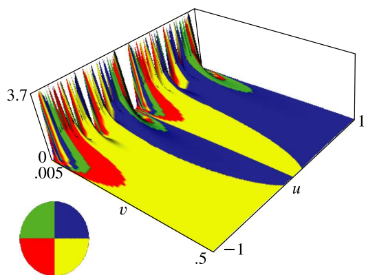
Figure 20.3.18: \theta_1(0.1|u + iv) , -1 \leq u \leq 1 , 0.005 \leq v \leq 0.5 . The value 0.1 of z is chosen arbitrarily since \theta_1 vanishes identically when z = 0 .
