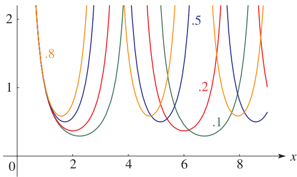
Figure 23.4.2: \wp(x; 0, g_3) for 0 \leq x \leq 9 , g_3 = 0.1, 0.2, 0.5, 0.8 . (Equianharmonic case.)
