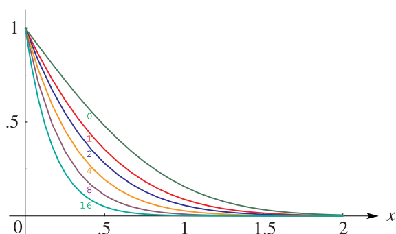
Figure 7.18.1: Repeated integrals of the scaled complementary error function 2^n \Gamma(\frac{1}{2}n + 1) i^n \operatorname{erfc}(x) , n = 0, 1, 2, 4, 8, 16 .
