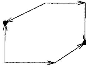
bad (two sinks)
