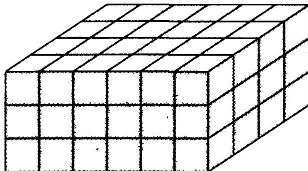
\mathcal{P}_3(6, 4, 3)
