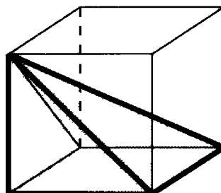
d = 3 \dim(P) = 3 \delta(G(P)) = 2
