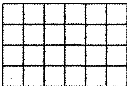
\mathcal{P}_2(6, 4)
