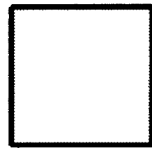
d = 2 \dim(P) = 2 \delta(G(P)) = 2
