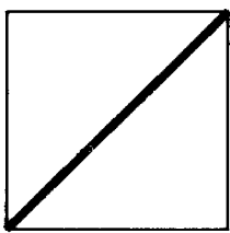
d = 2 \dim(P) = 1 \delta(G(P)) = 1
