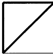
d = 2 \dim(P) = 2 \delta(G(P)) = 1
