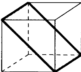
d = 3 \dim(P) = 2 \delta(G(P)) = 2
