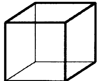
d = 3 \dim(P) = 3 \delta(G(P)) = 3
