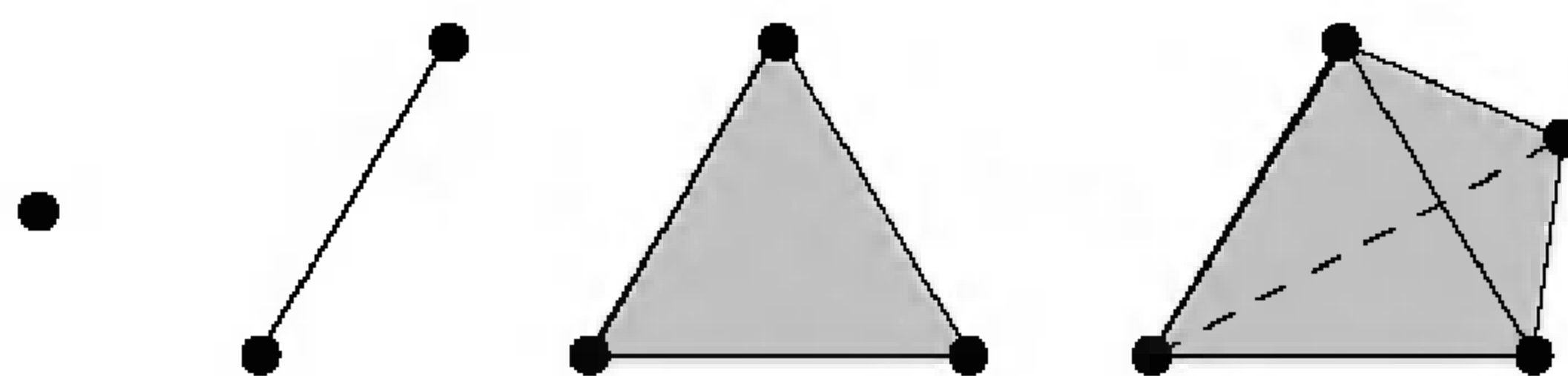
FIGURE 5.1. Simplicies.
