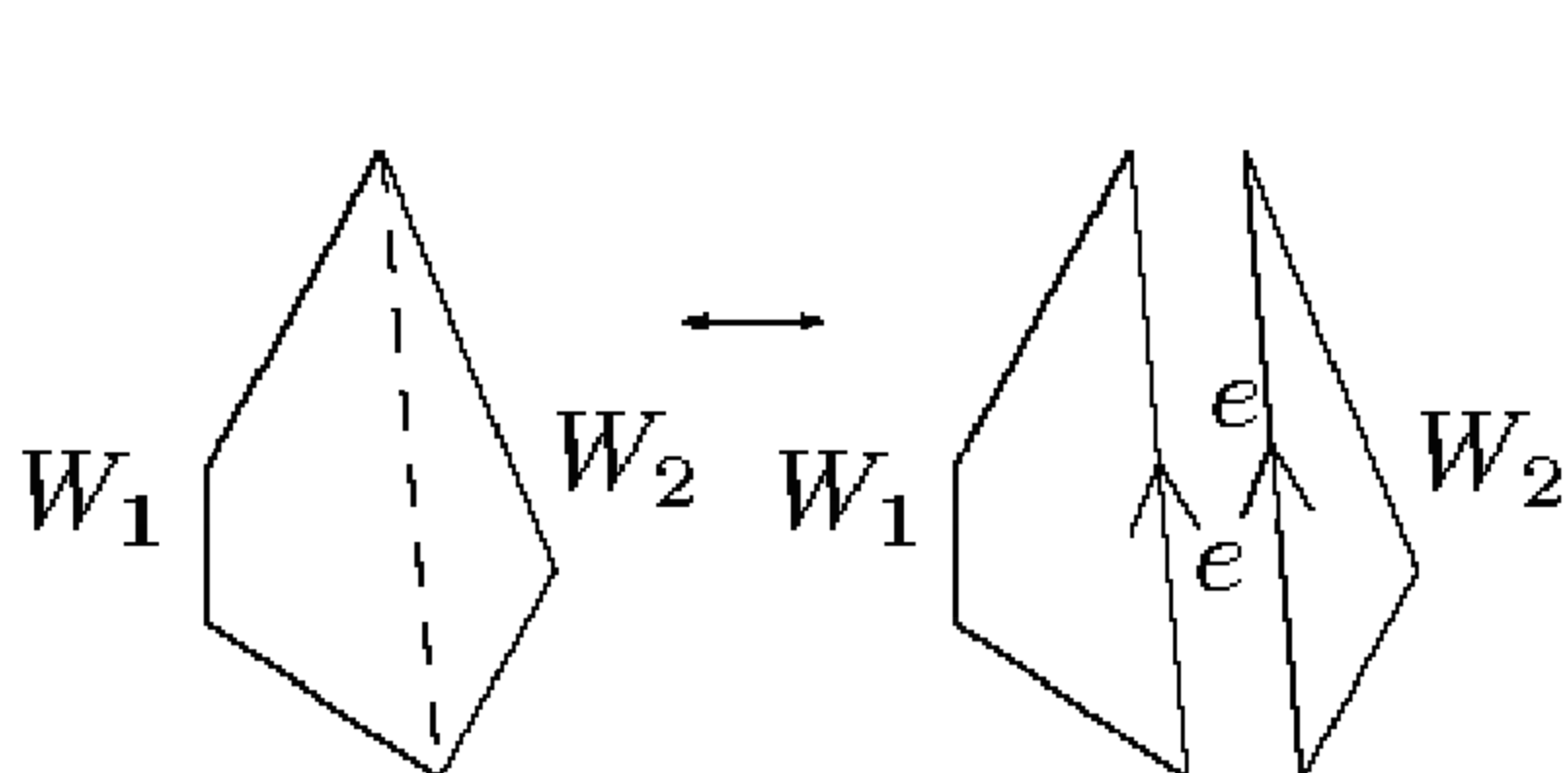
FIGURE 6.20. Cutting/pasting.
