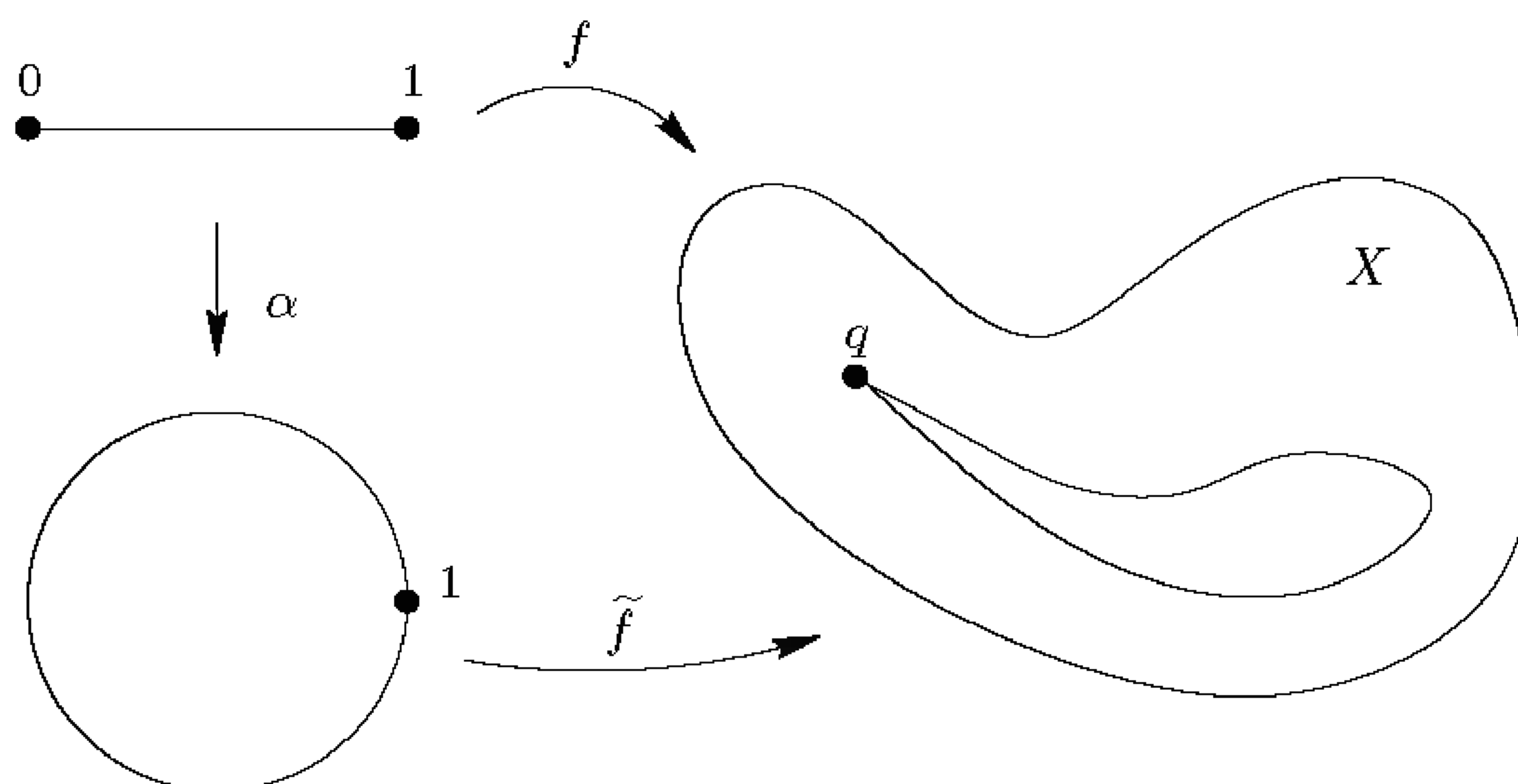
FIGURE 7.8. The circle representative of a loop.
