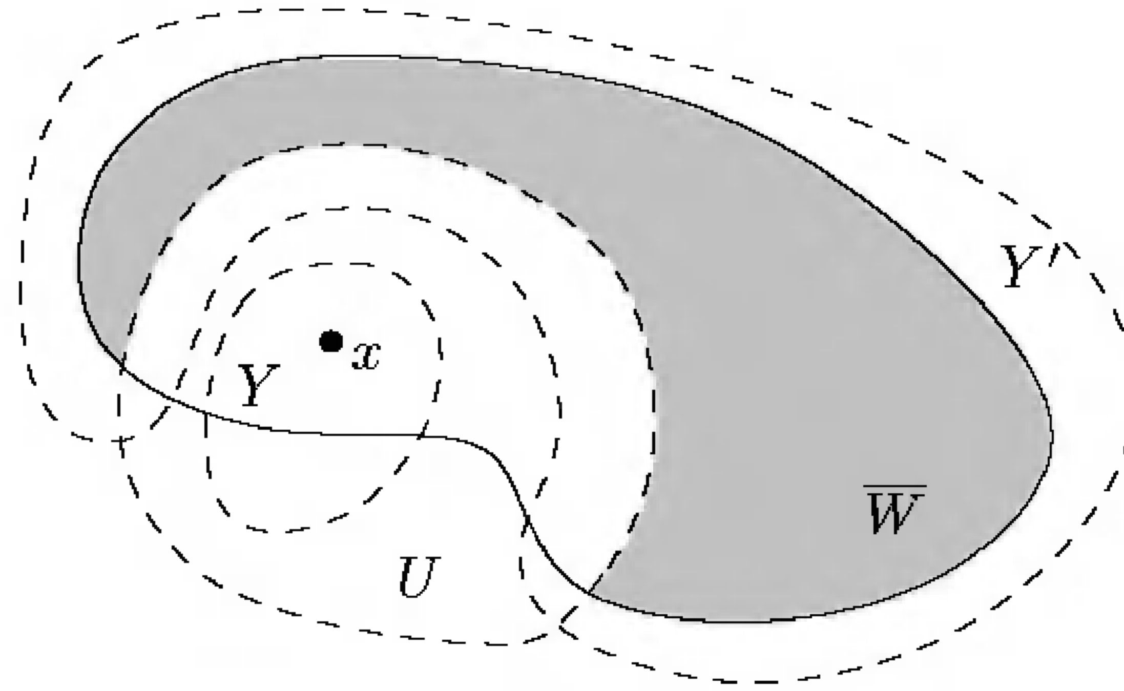
FIGURE 4.9. Proof of the shrinking lemma.
