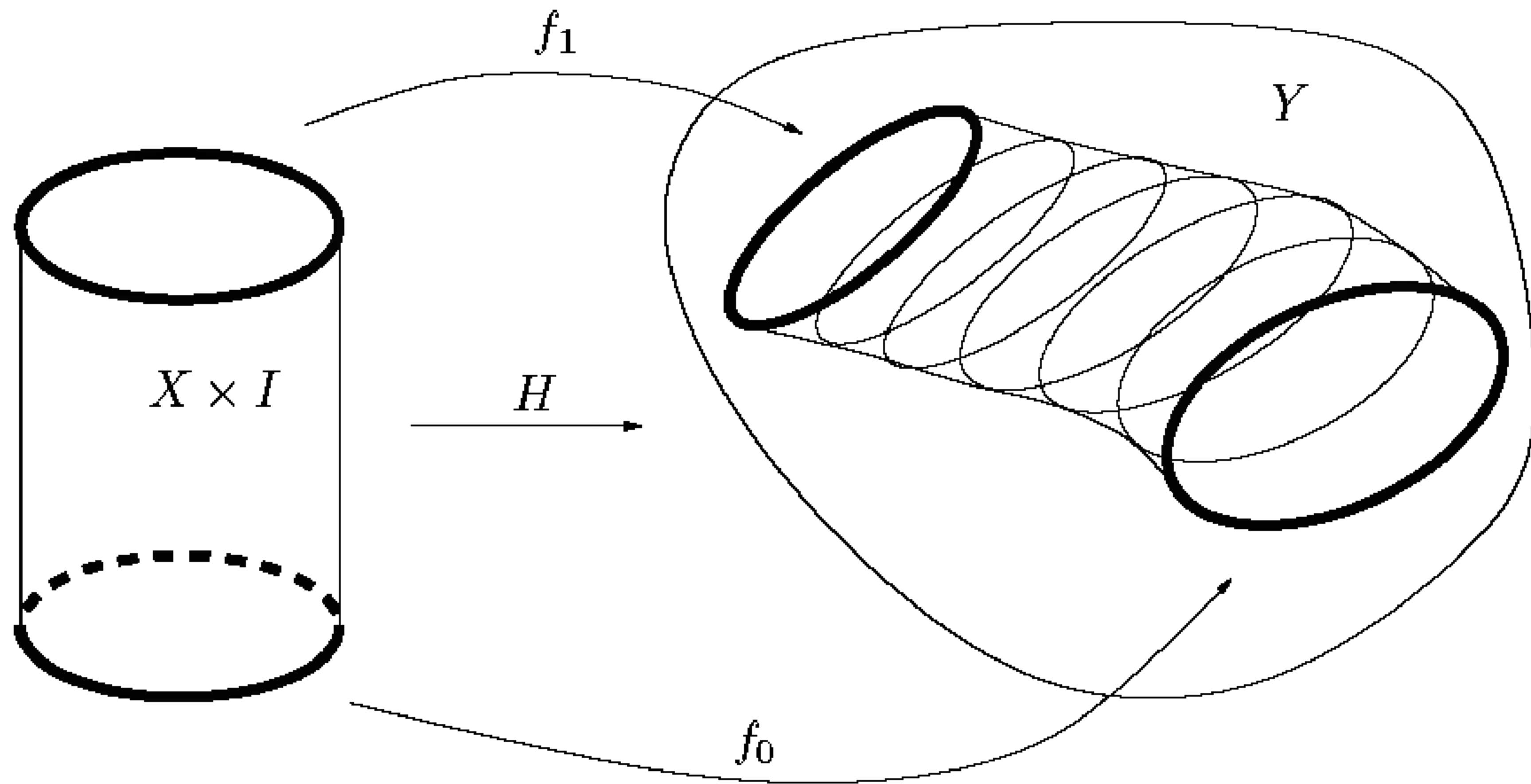
FIGURE 7.1. A homotopy between f_0 and f_1 .
