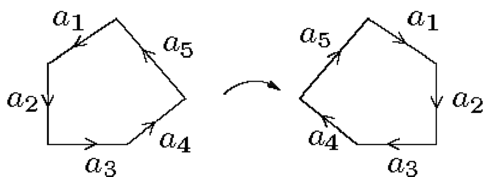
FIGURE 6.18. Reflecting.
