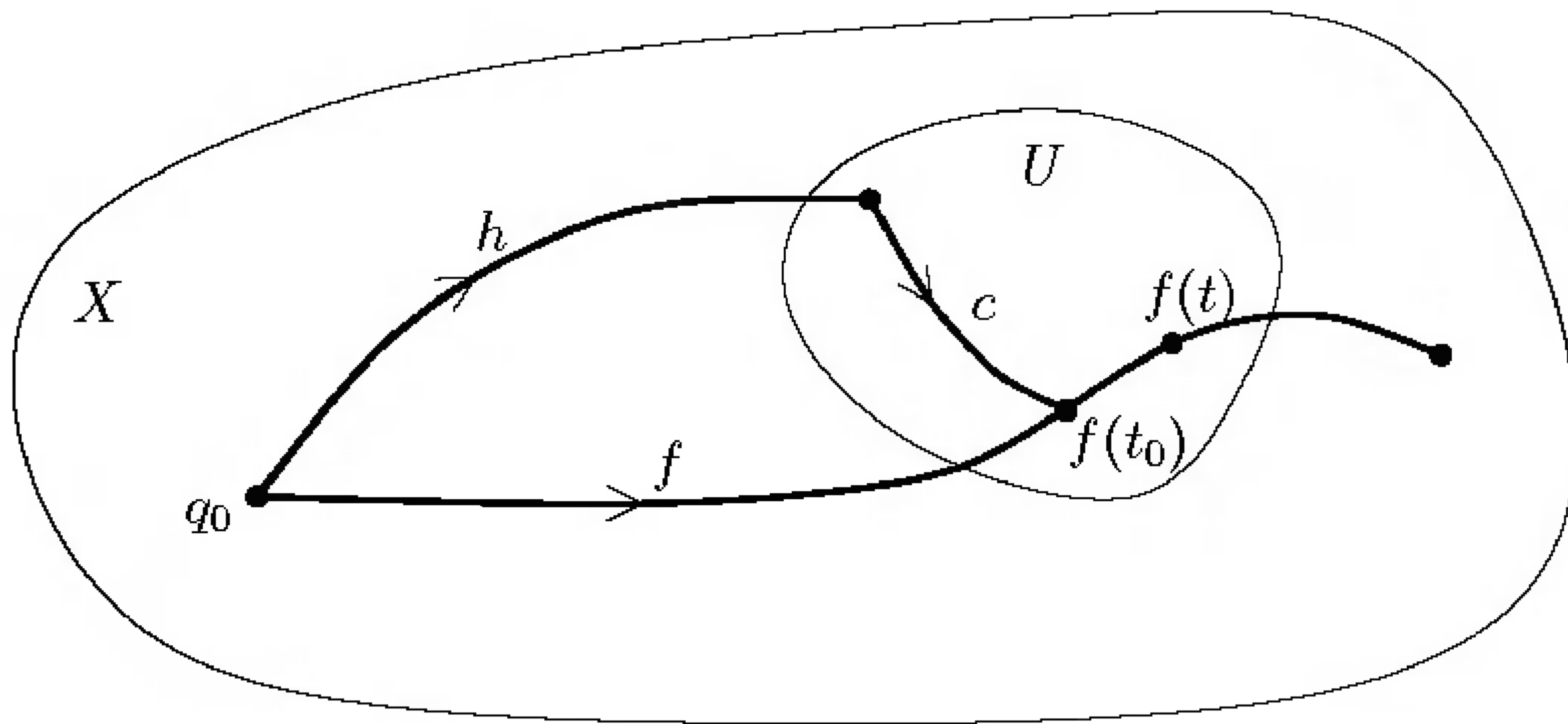
FIGURE 12.4. Proof that \tilde{X} is path connected.
