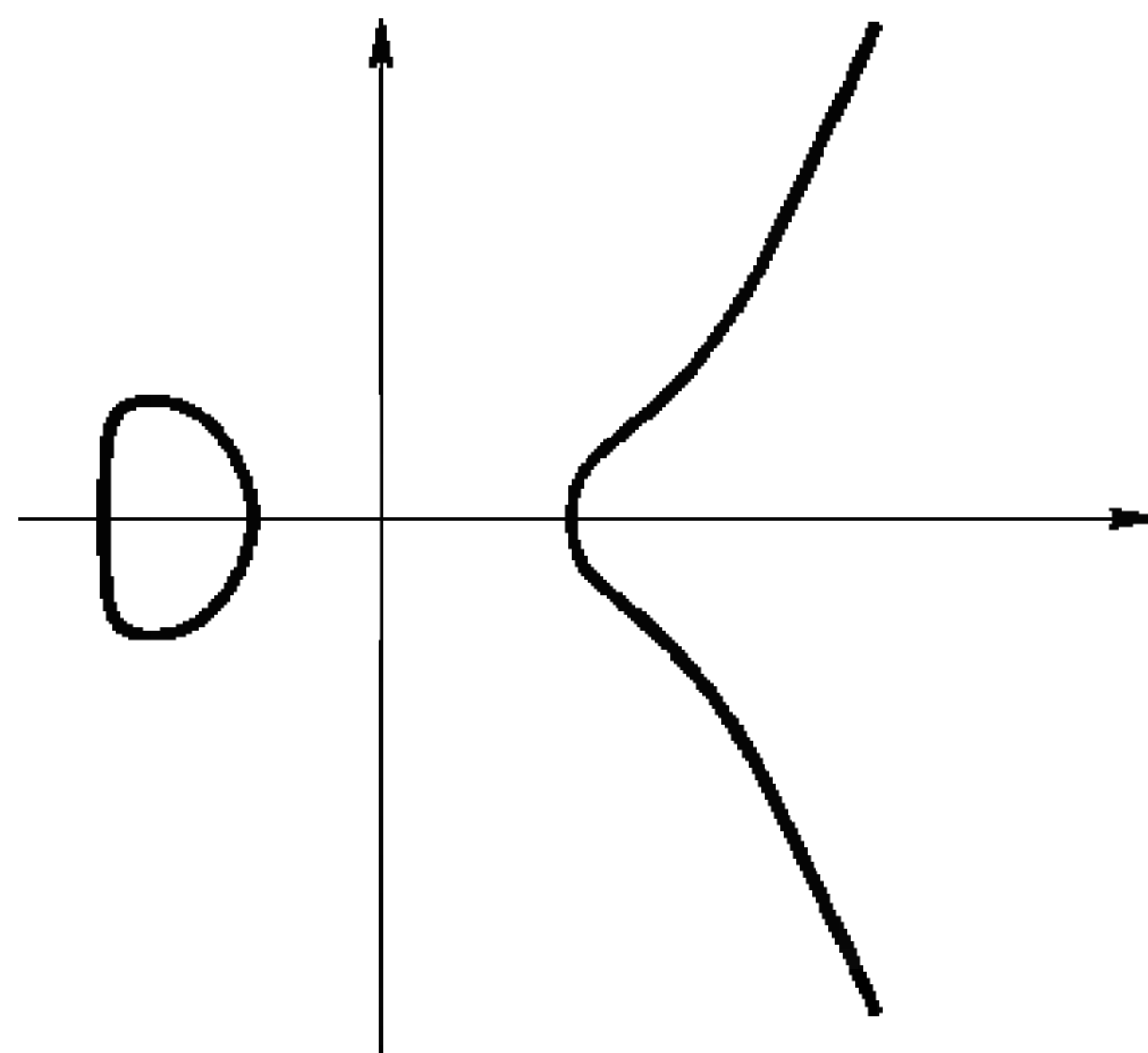
FIGURE 1.8. A plane curve with disconnected pieces.
