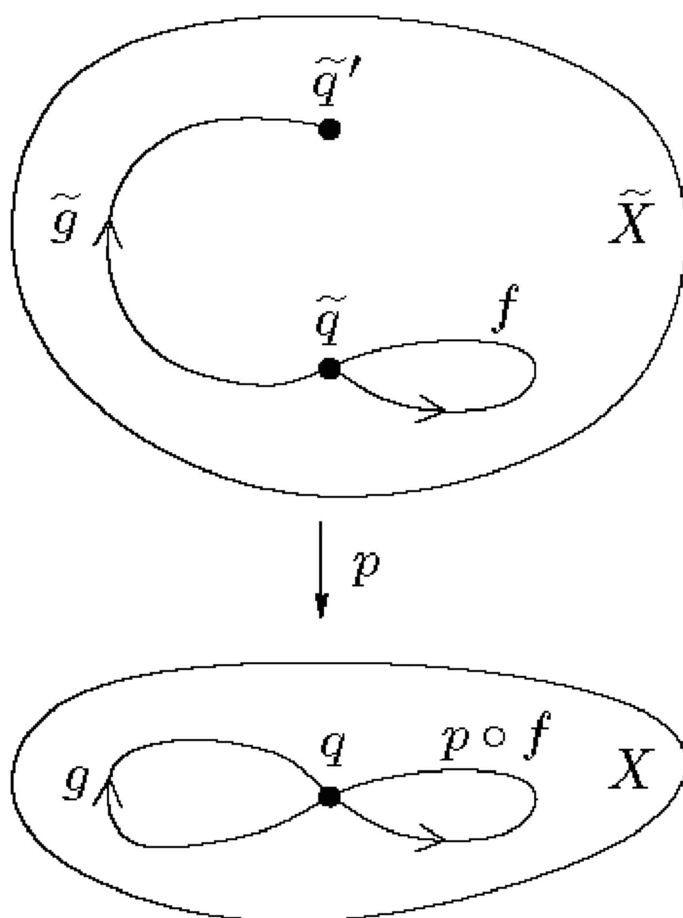
FIGURE 11.7. Proof of the conjugacy theorem.
