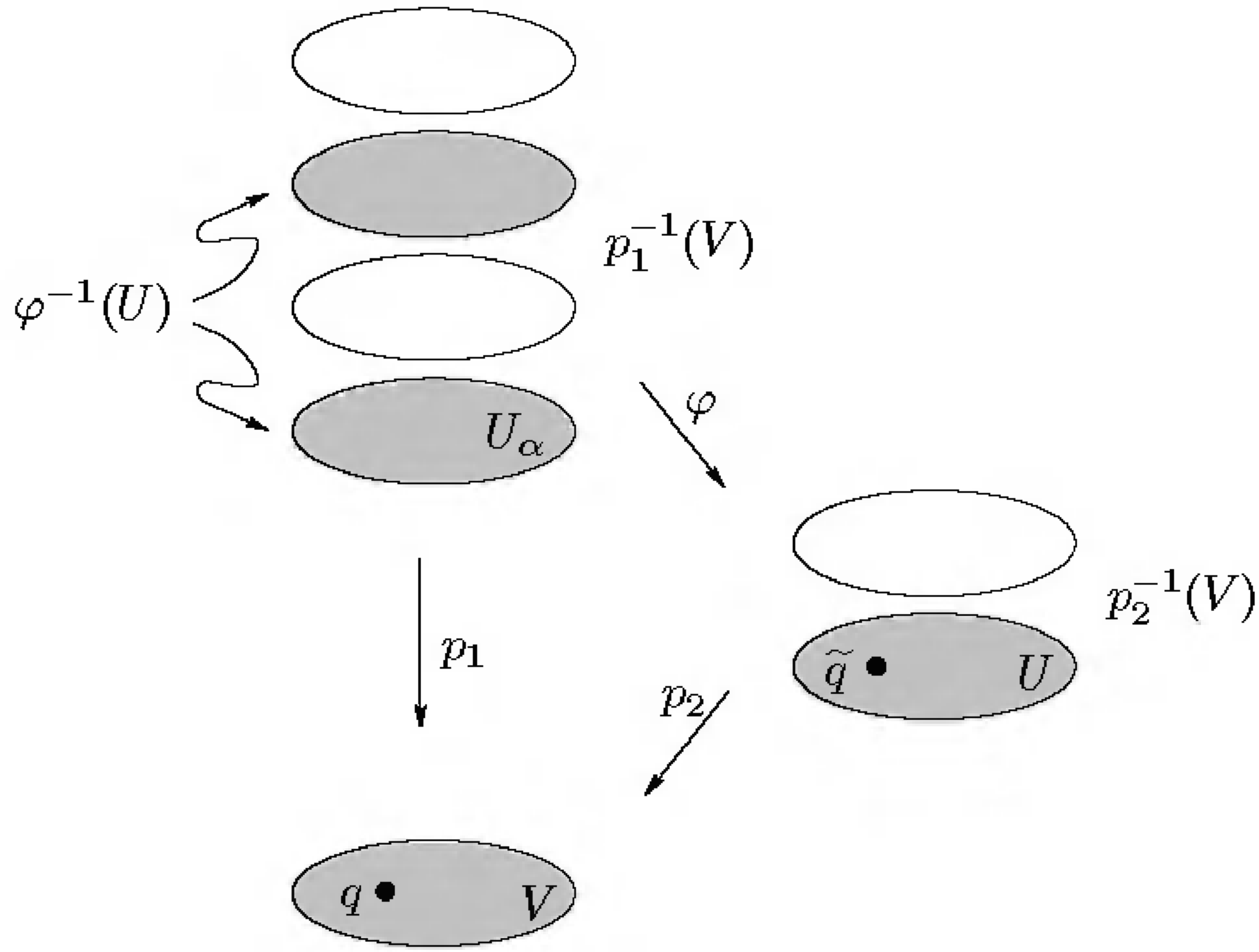
FIGURE 12.2. An evenly covered neighborhood of \tilde{q} .
