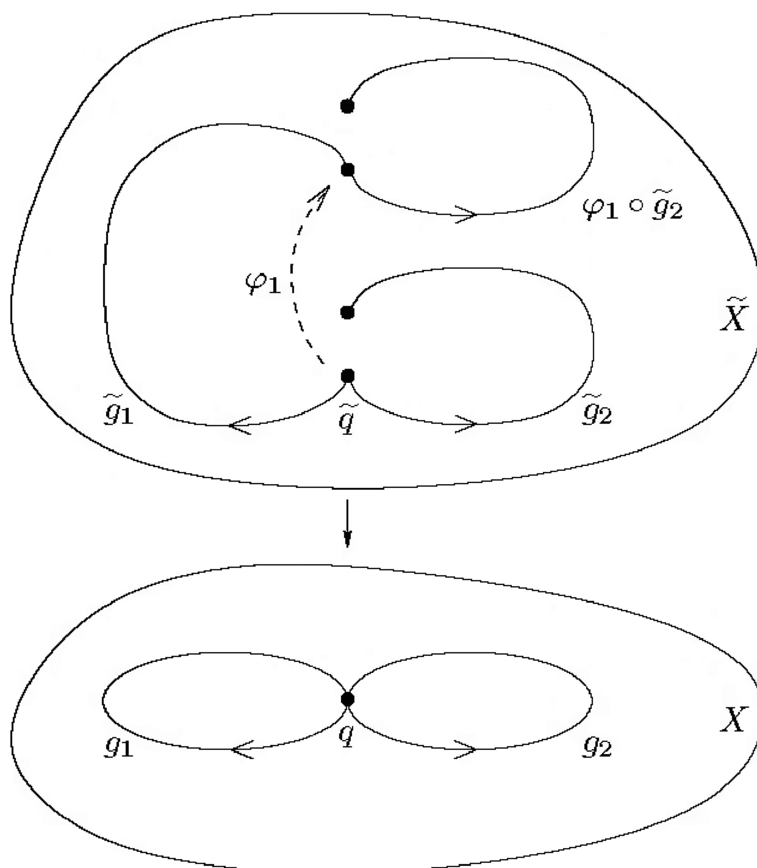
FIGURE 11.9. Proof that \alpha is a homomorphism.
