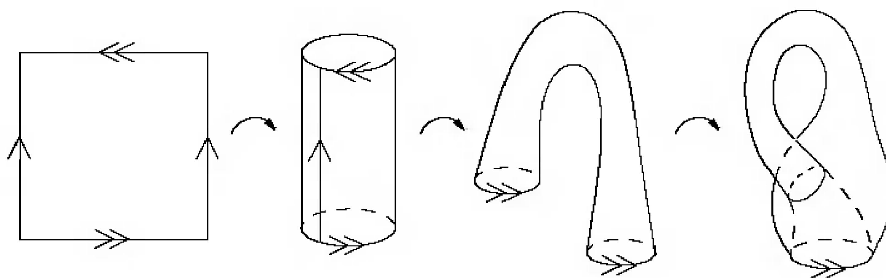
FIGURE 6.9. The Klein bottle.
