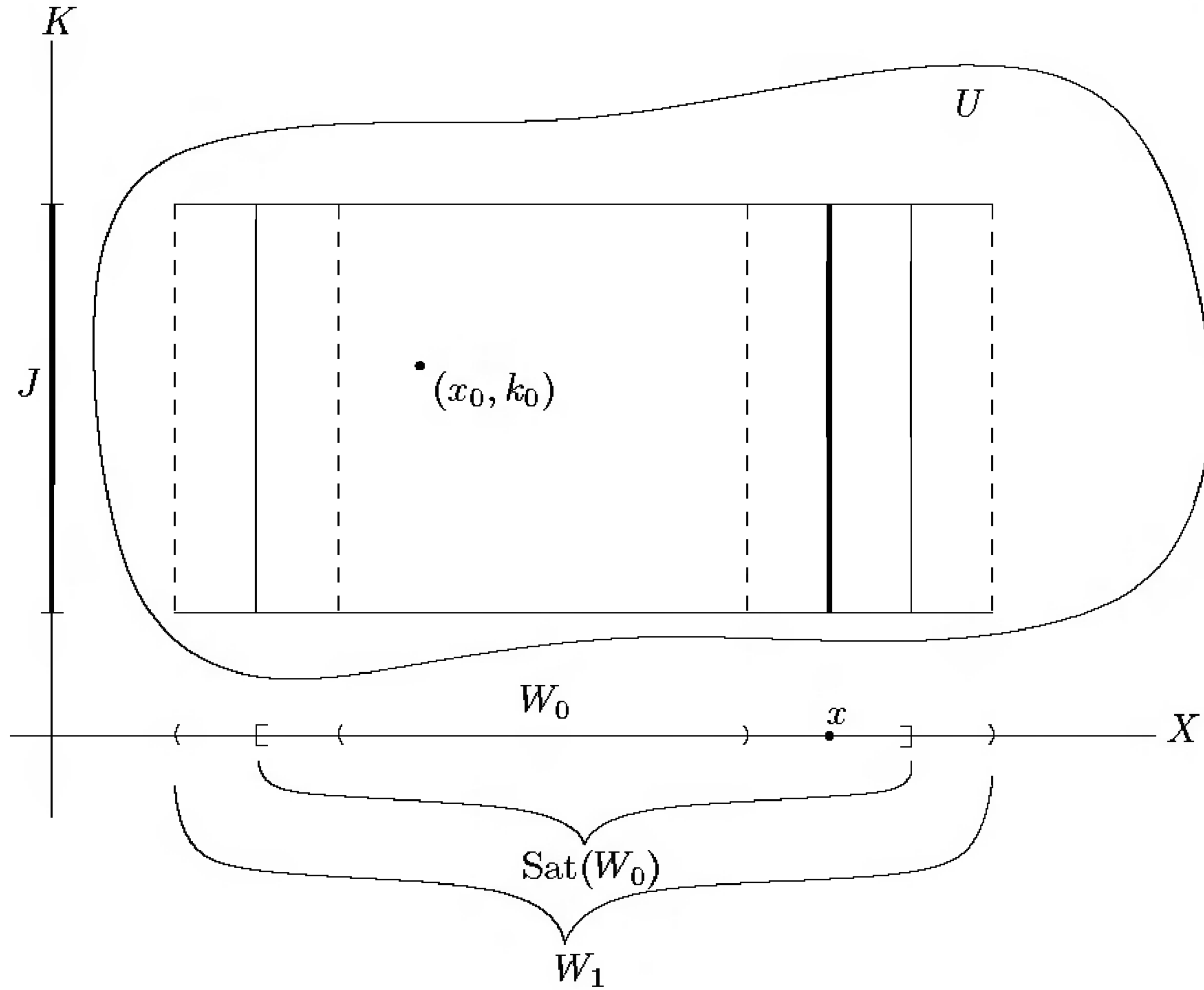
FIGURE 4.11. Finding a saturated product neighborhood.
