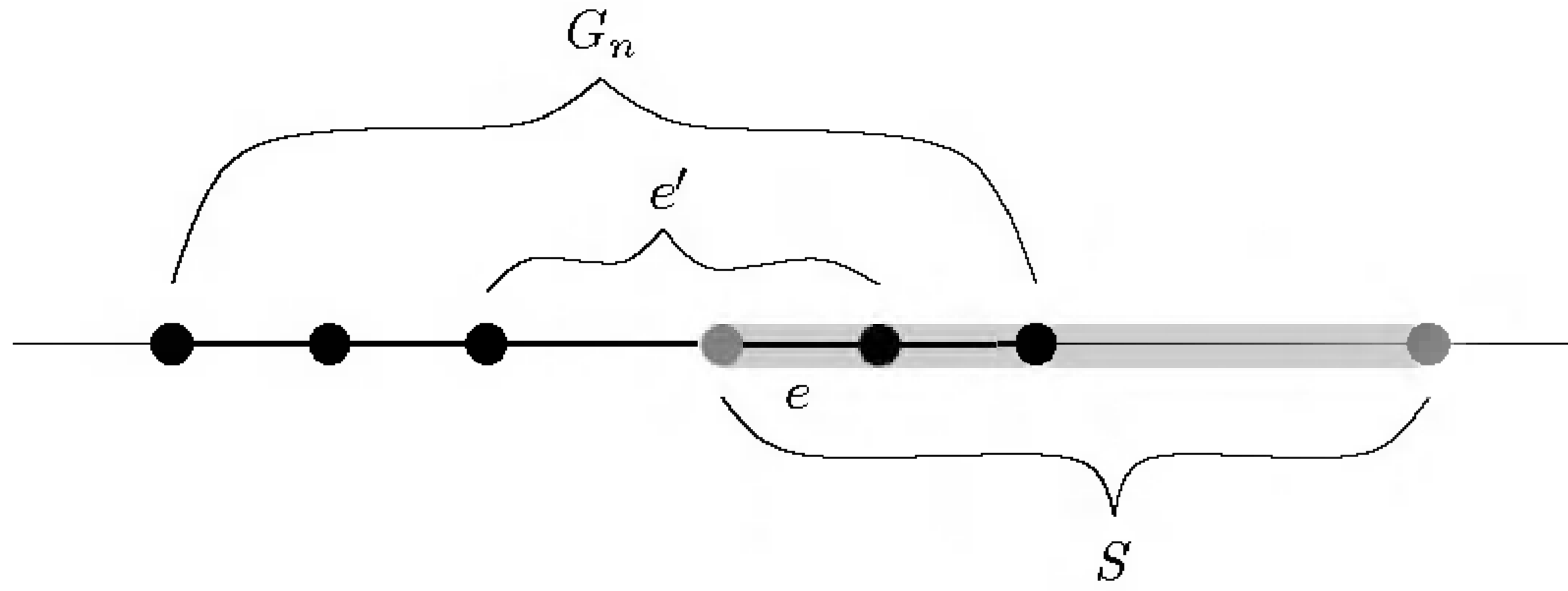
FIGURE 5.6. Proof that e \subset e' .
