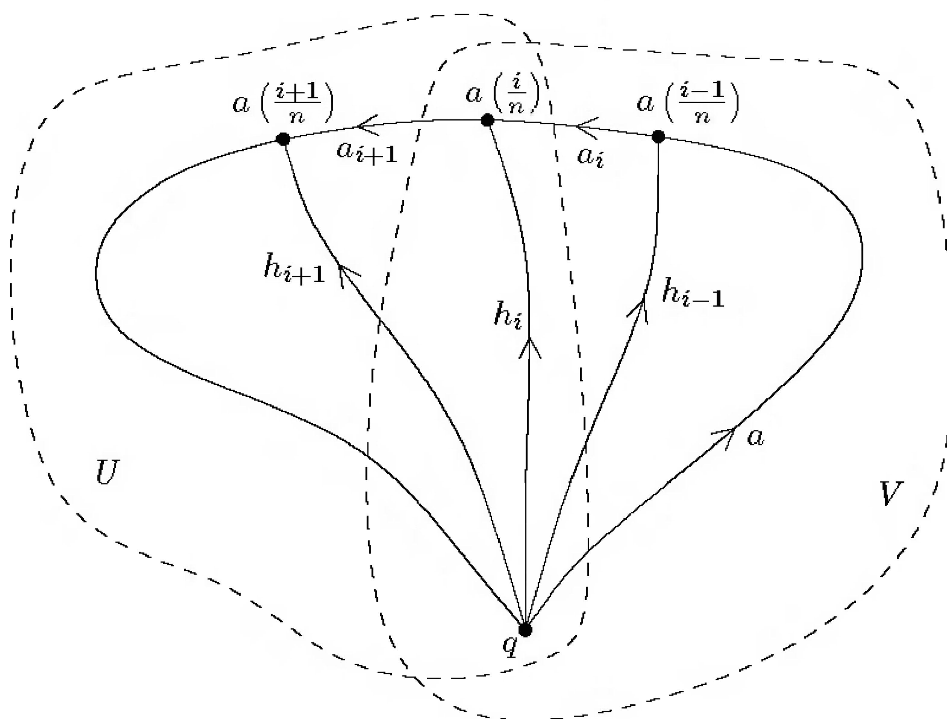
FIGURE 10.5. Proof that \Phi is surjective.
