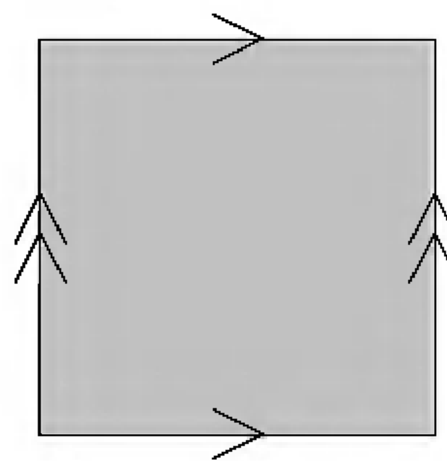
FIGURE 3.9. A quotient of I \times I .
