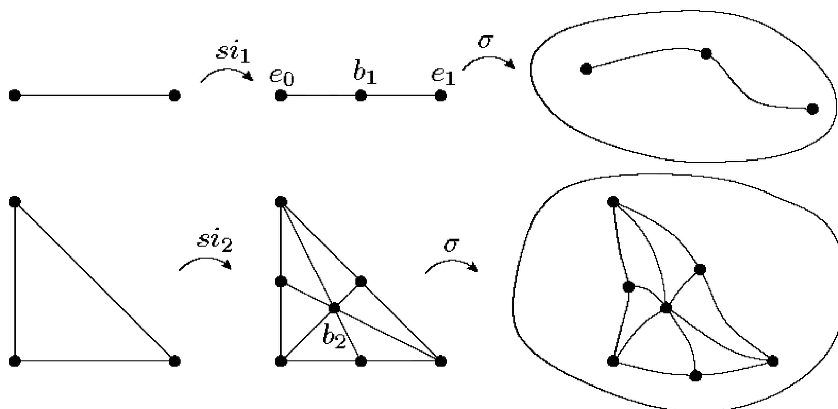
FIGURE 13.9. Singular subdivisions in dimensions 1 and 2.
