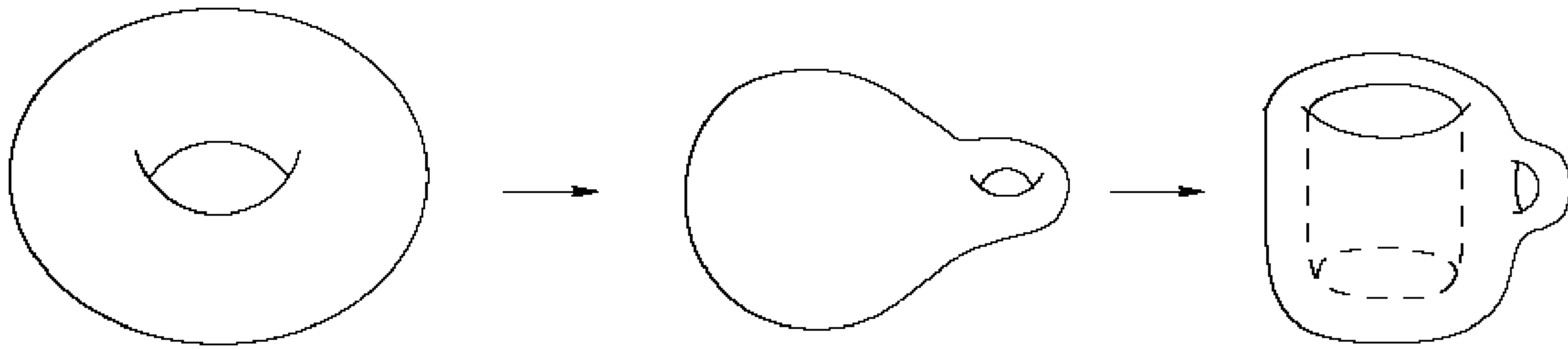
FIGURE 1.4. Deforming a doughnut into a coffee cup.
