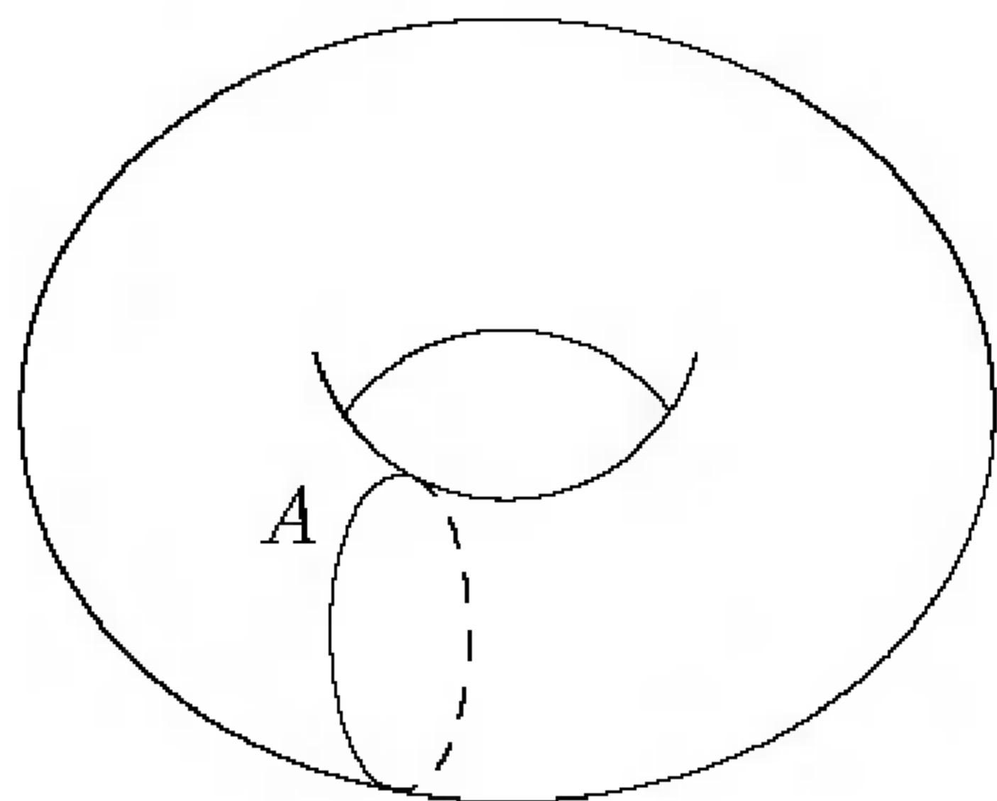
FIGURE 7.10. S^1 is a retract of \mathbb{T}^2 .
