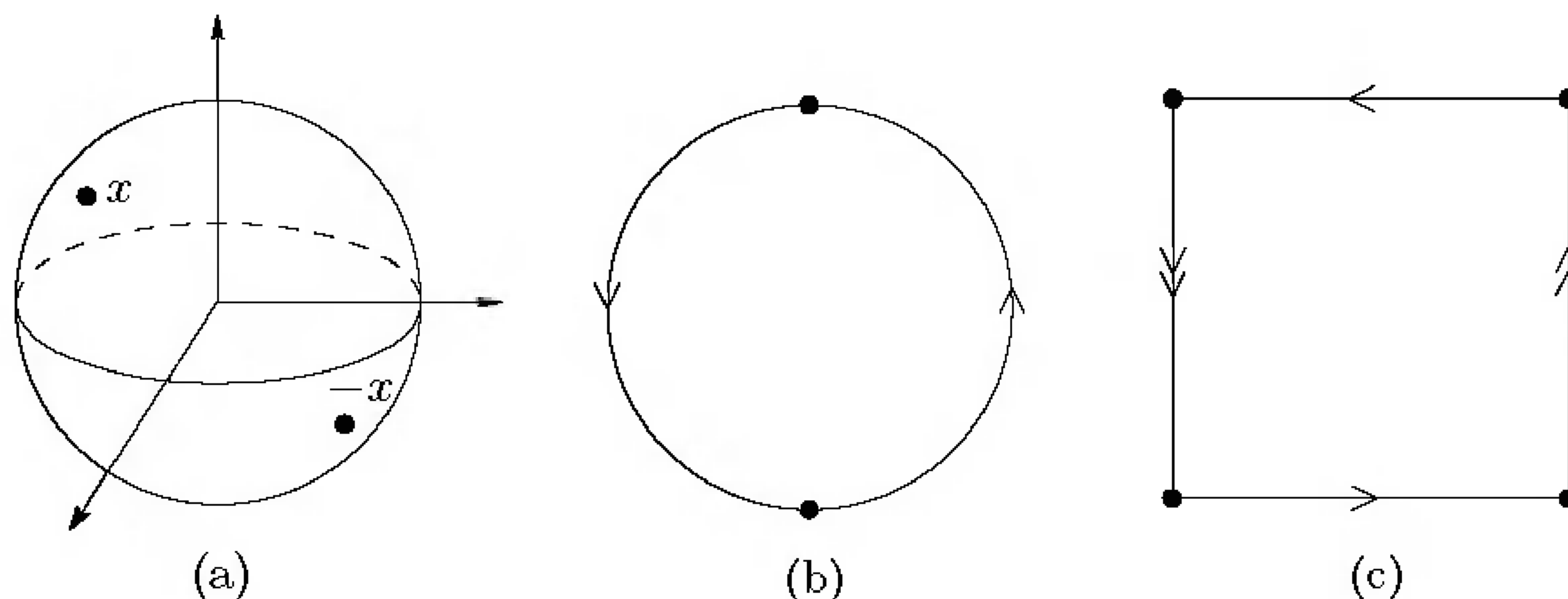
FIGURE 6.4. Representations of \mathbb{P}^2 as a quotient space.
