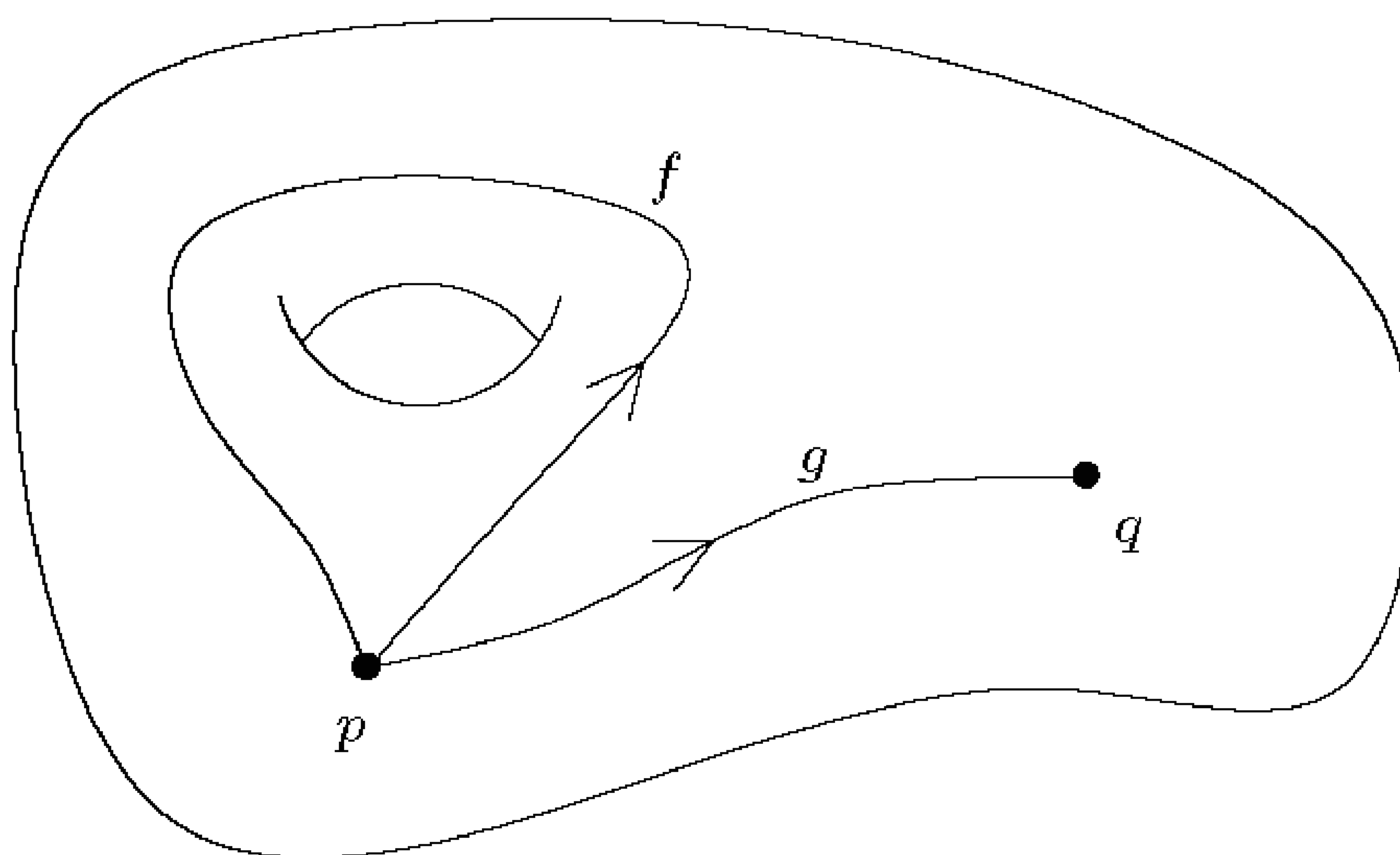
FIGURE 7.6. Change of base point.
