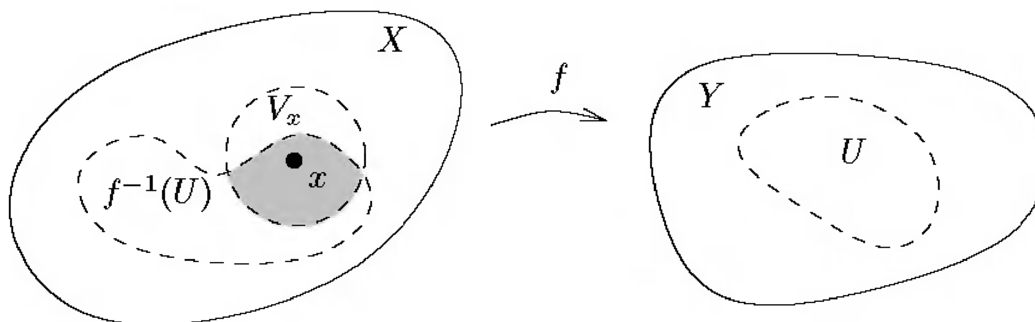
FIGURE 2.2. Local criterion for continuity.
