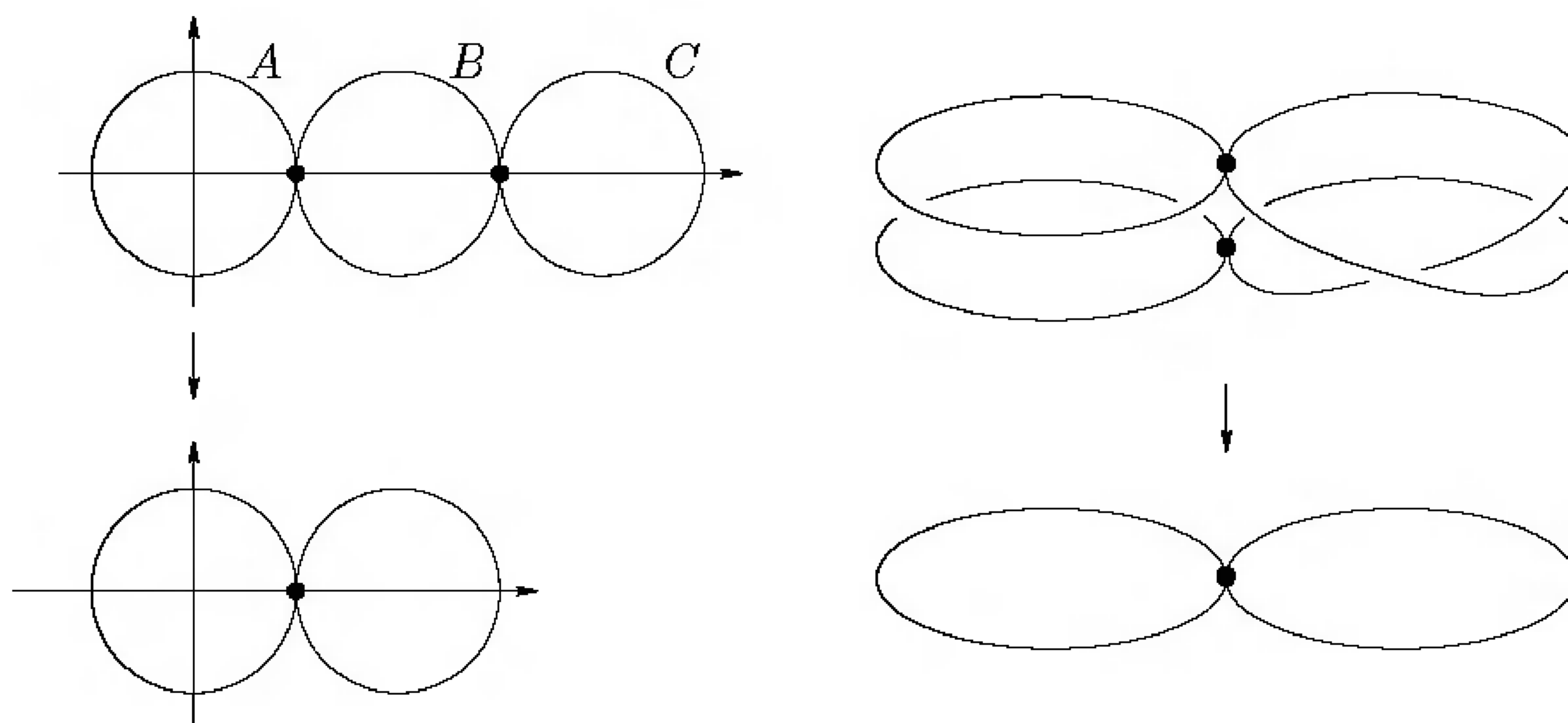
FIGURE 11.2. Two views of the map of Exercise 11.1.
