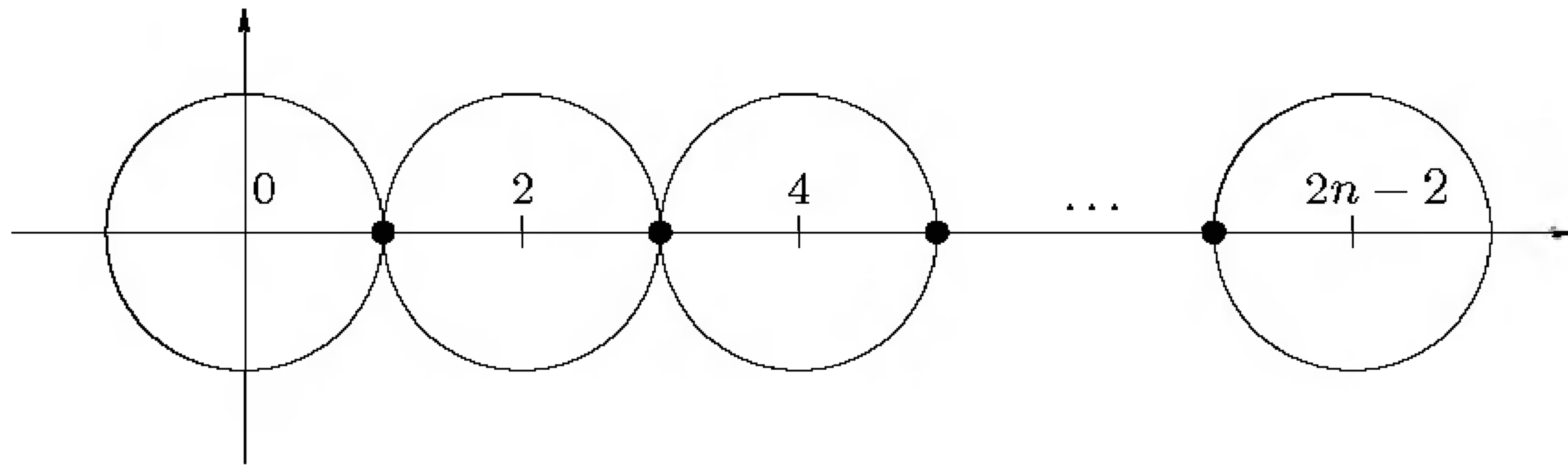
FIGURE 10.7. The space X_n of Problem 10-10.
