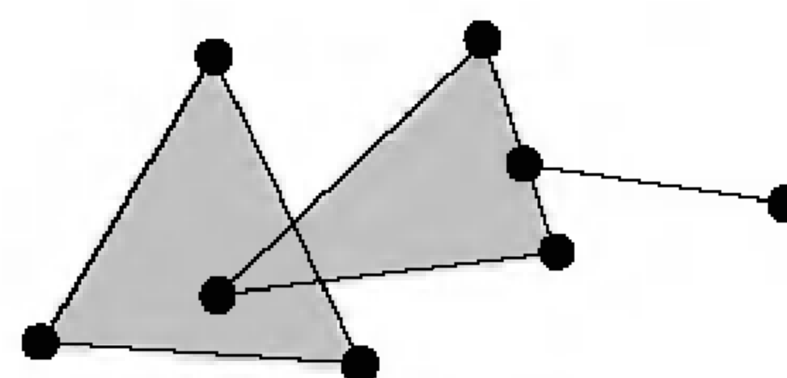
FIGURE 5.3. Not a complex.
