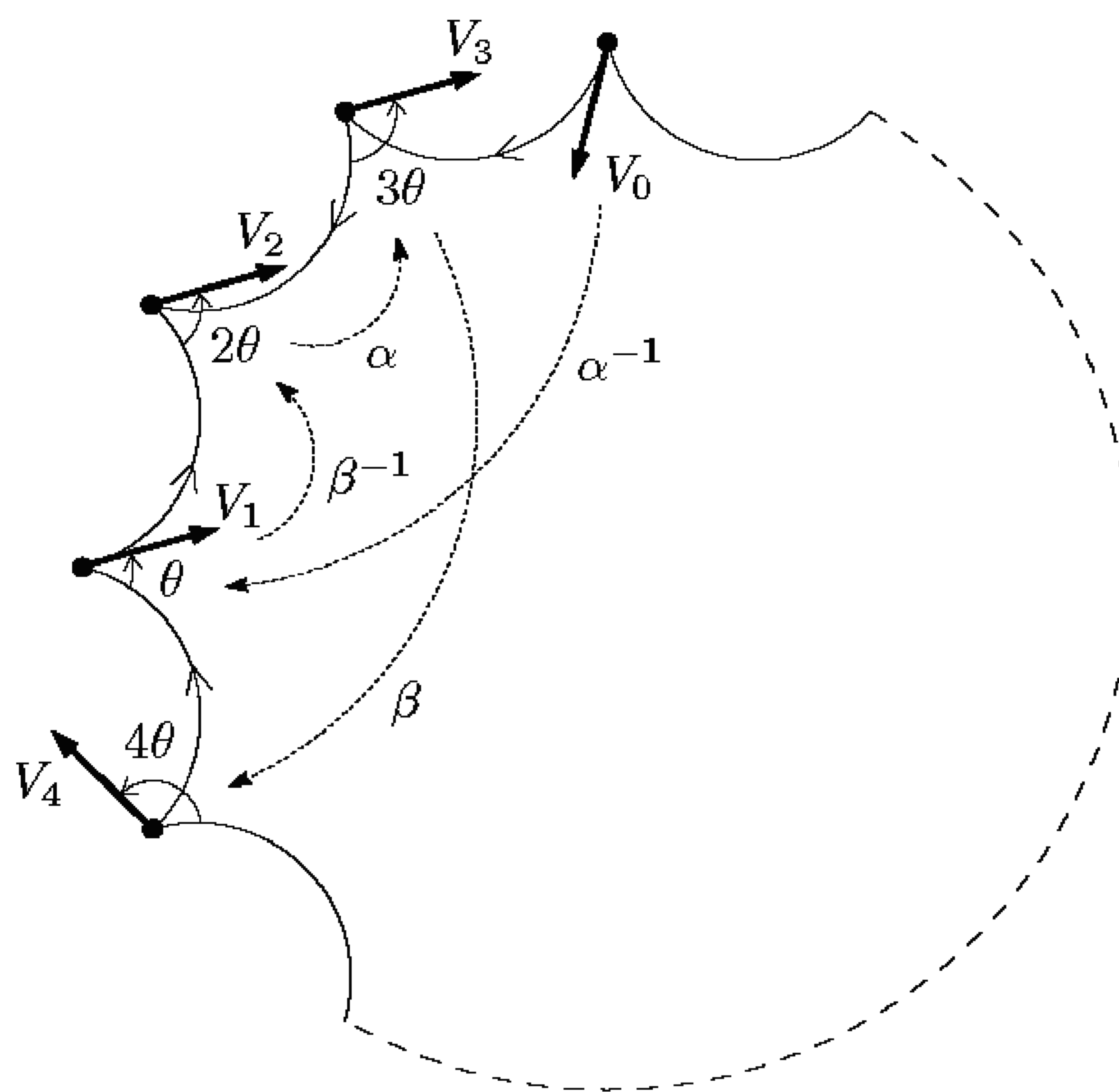
FIGURE 12.9. Images of a vector V_0 under edge pairing transformations.
