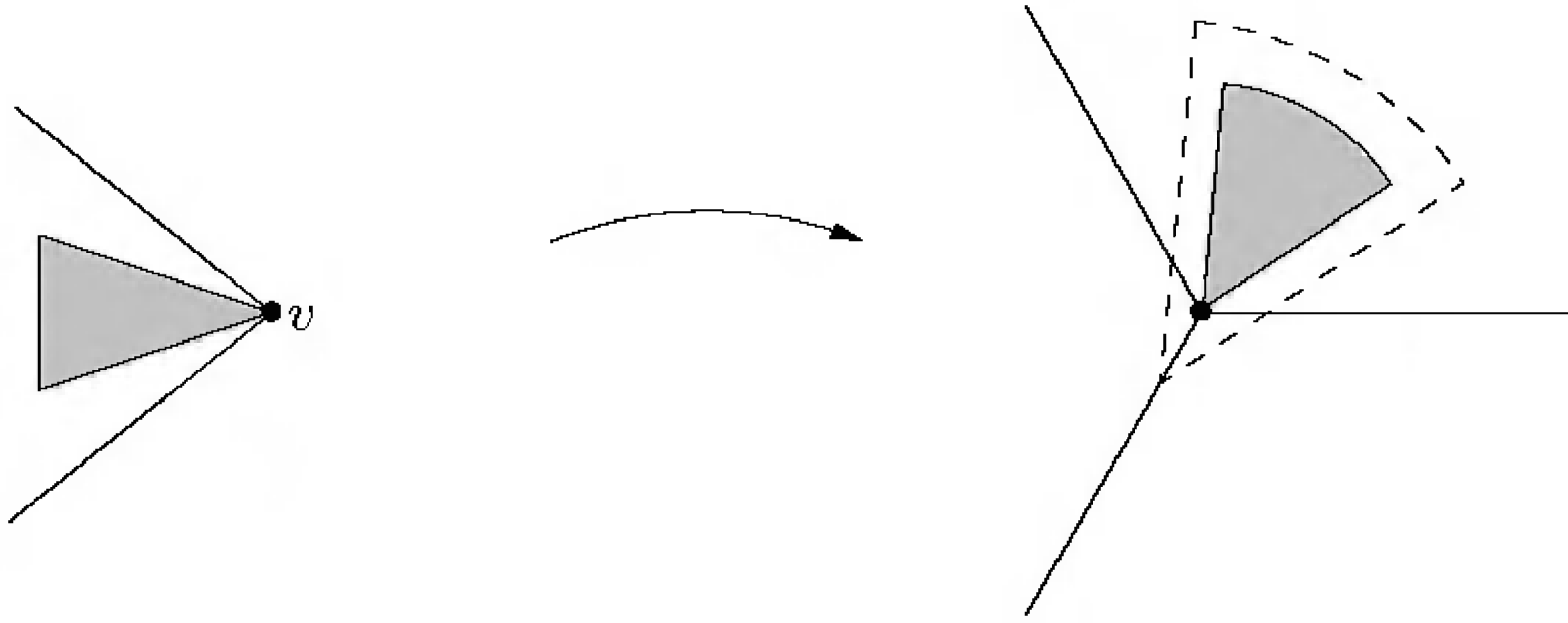
FIGURE 6.23. Showing that B_1 is a regular disk.
