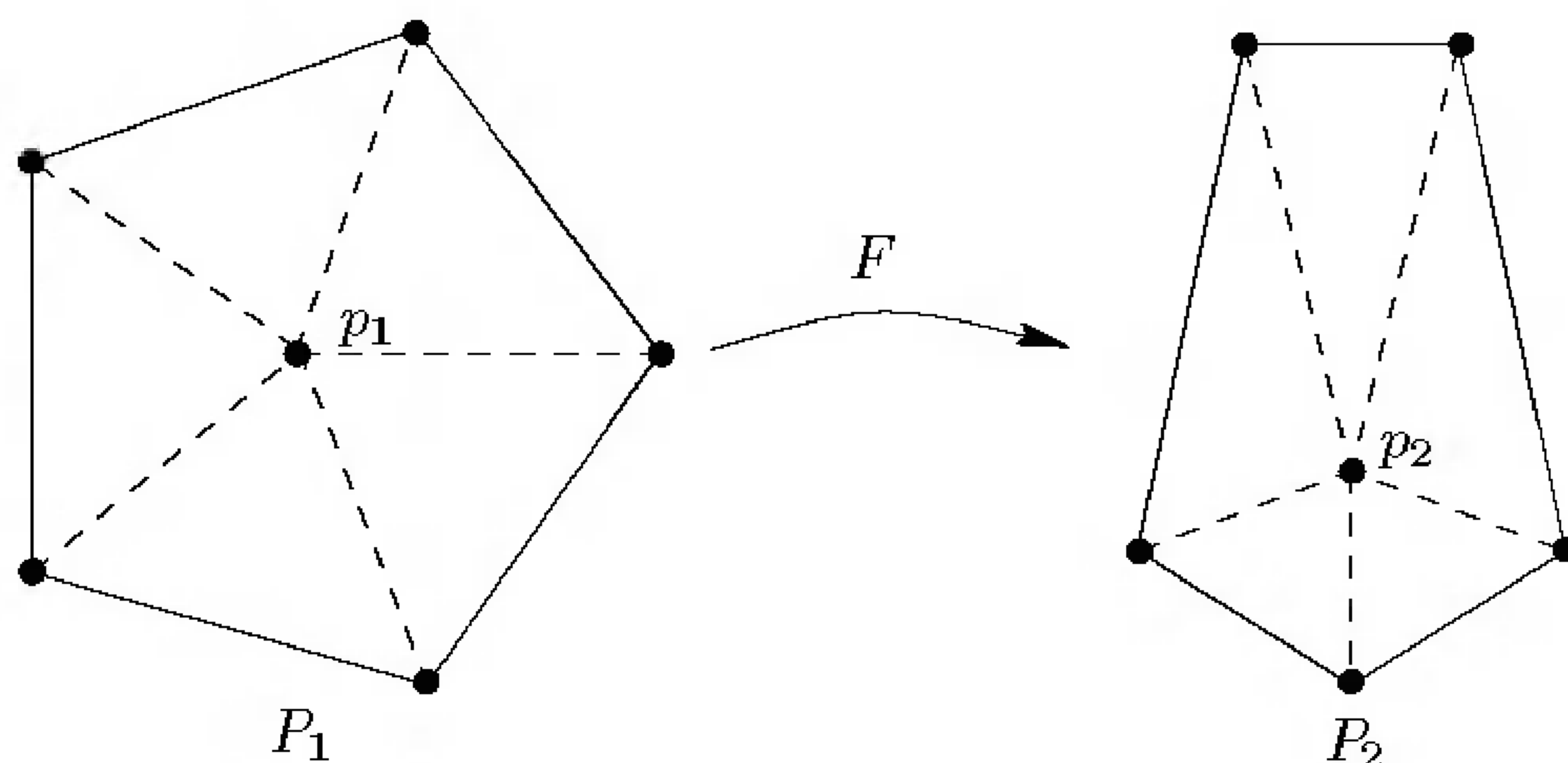
FIGURE 6.16. Simplicial homeomorphism between polygons.
