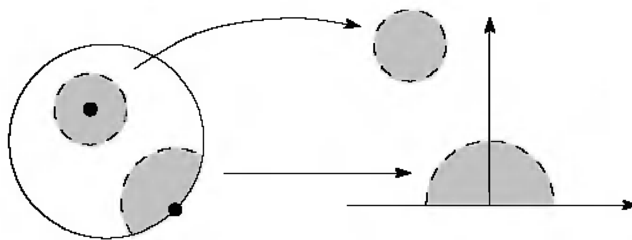
FIGURE 2.7. A manifold with boundary.
