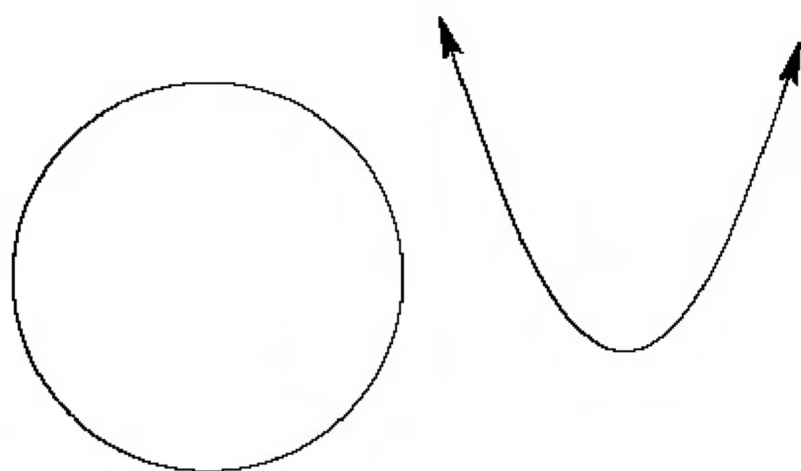
FIGURE 1.1. Plane curves.
