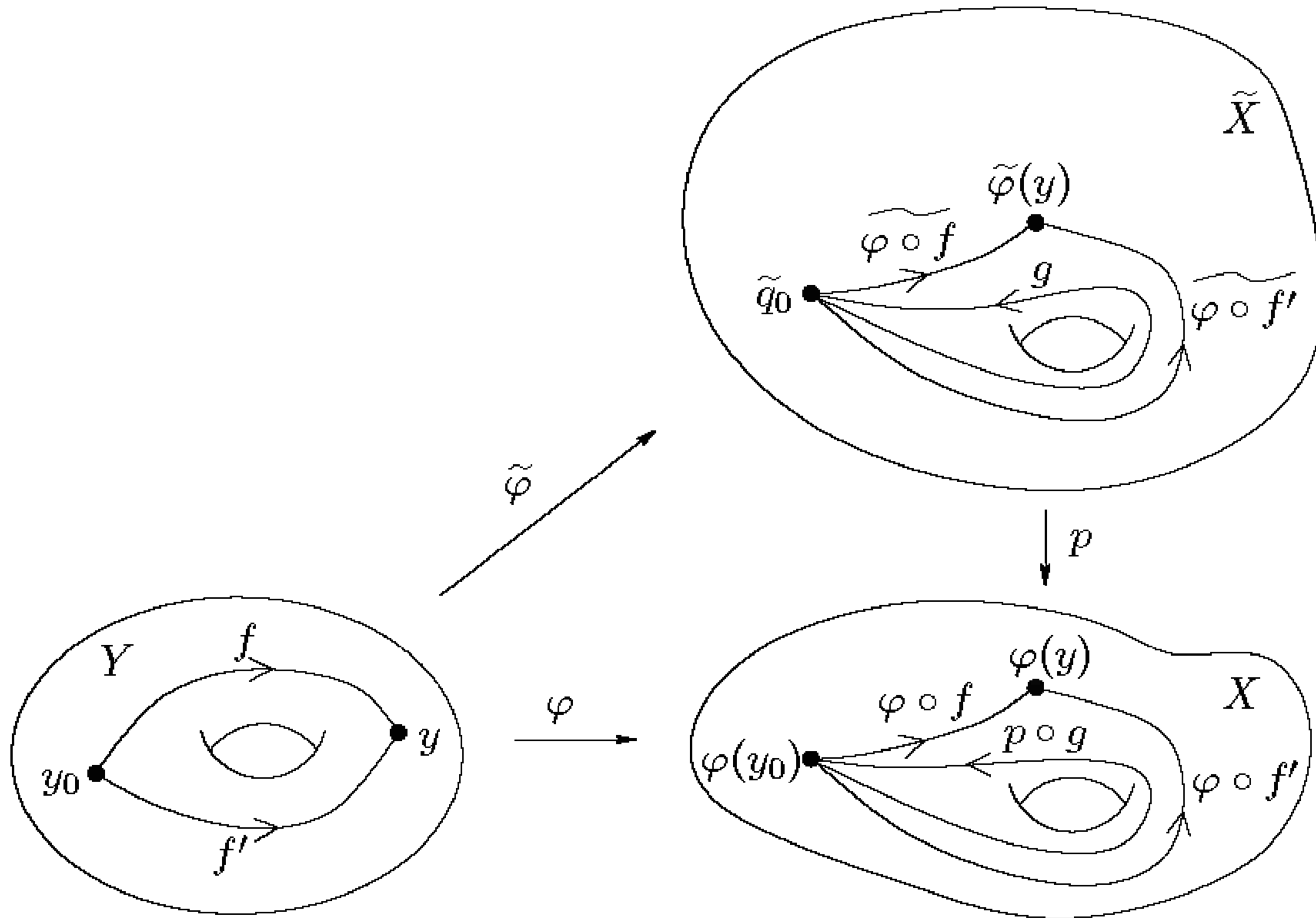
FIGURE 11.4. Proof that \tilde{\varphi} is well-defined.
