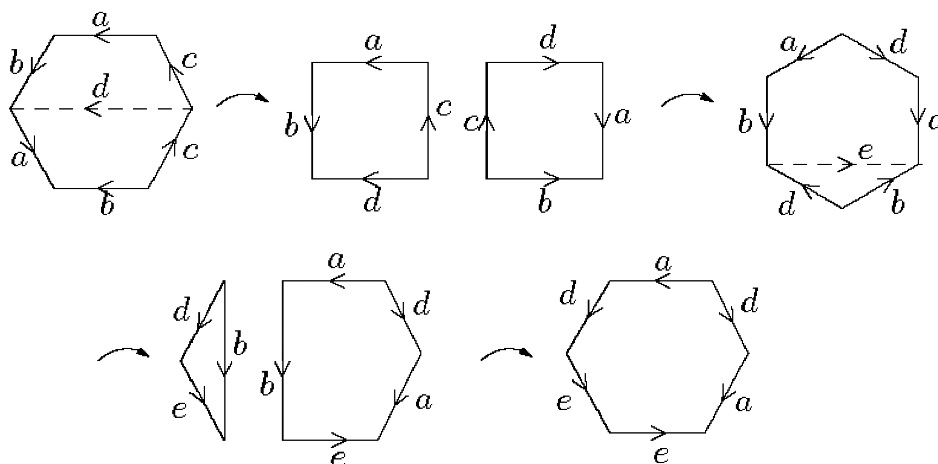
FIGURE 6.25. Transforming \mathbb{P}^2 \# \mathbb{P}^2 \# \mathbb{P}^2 to \mathbb{T}^2 \# \mathbb{P}^2 .
