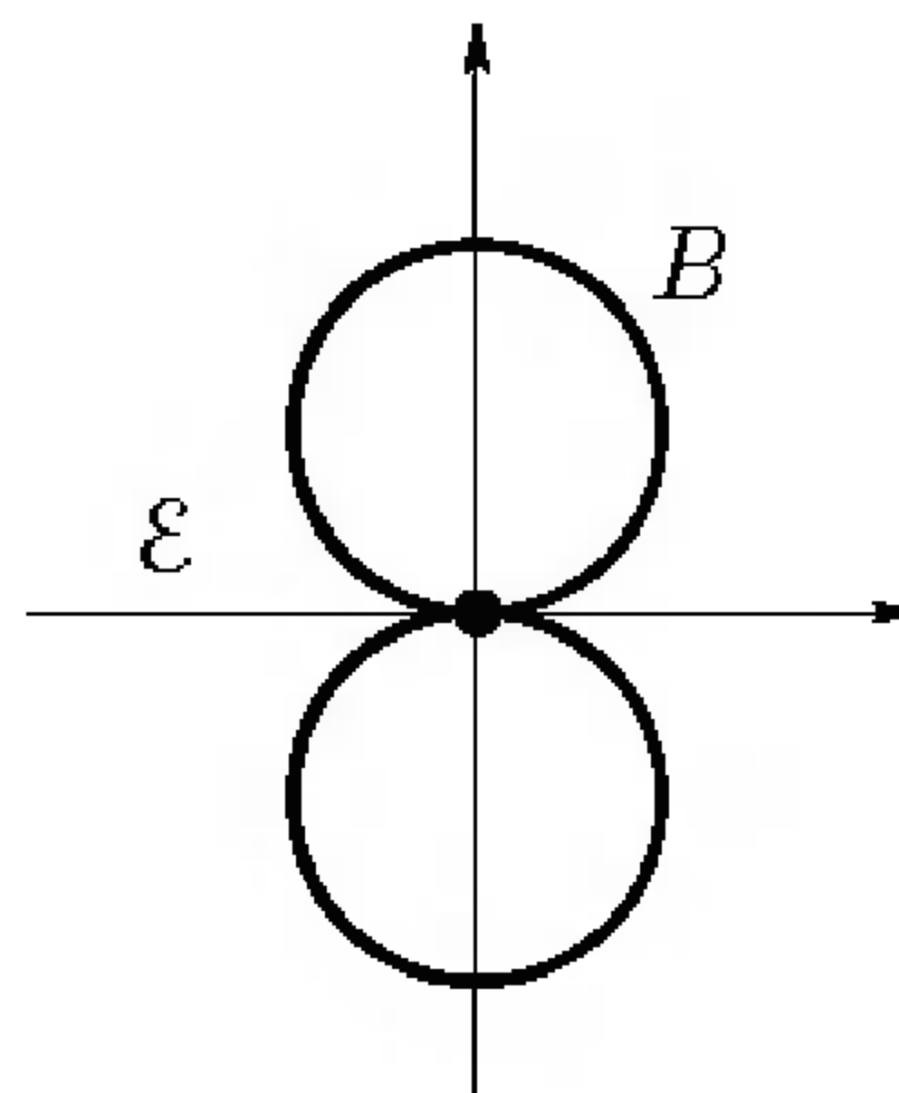
FIGURE 7.11. Figure eight space.
