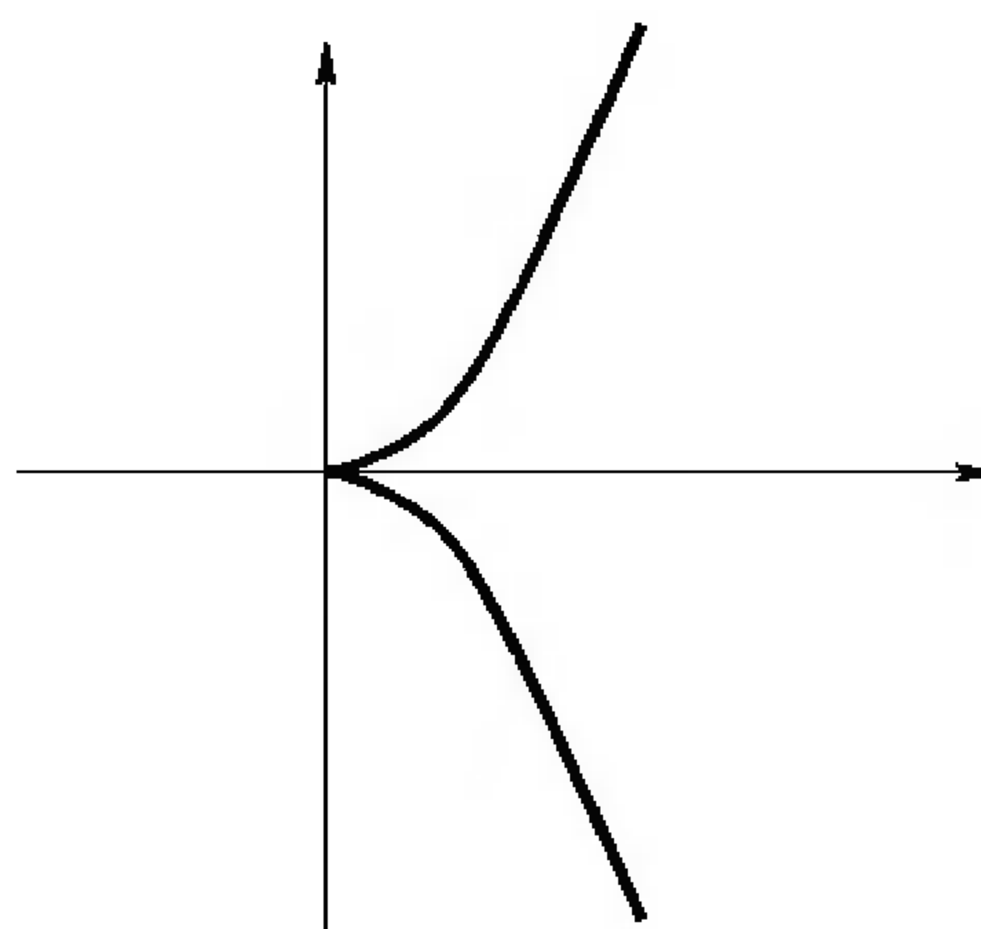
FIGURE 1.10. A cusp.
