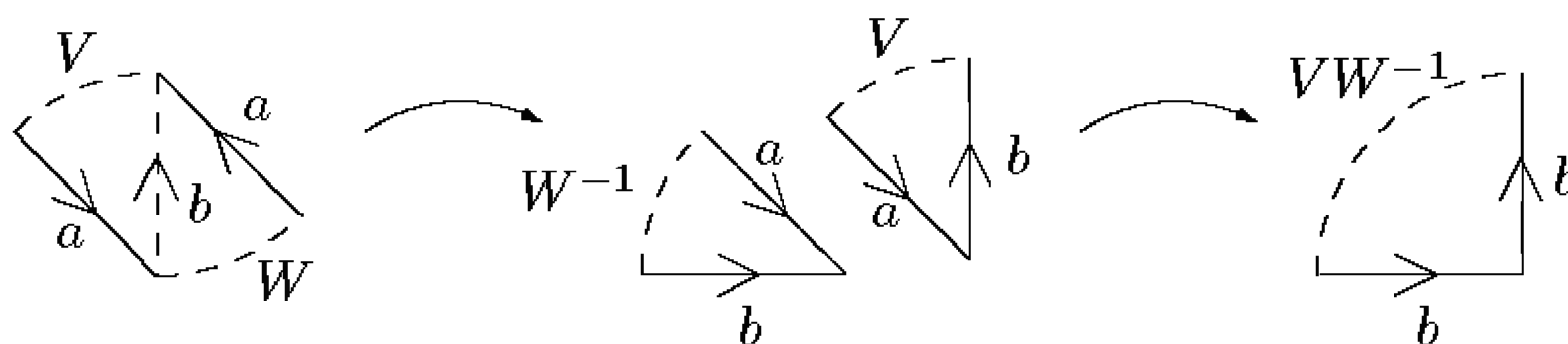
FIGURE 6.26. Making a twisted pair adjacent.
