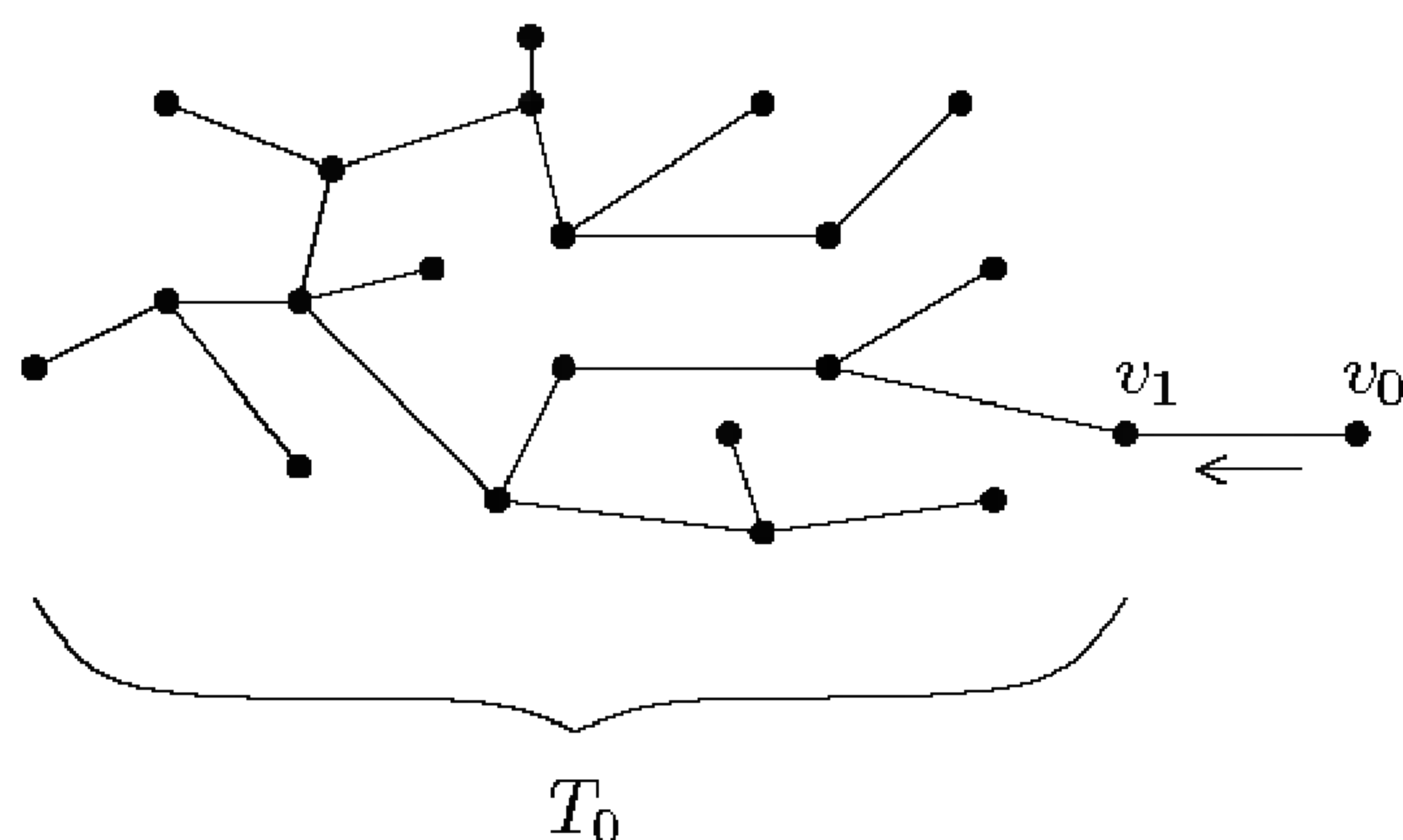
FIGURE 7.16. Proof that a tree is contractible.
