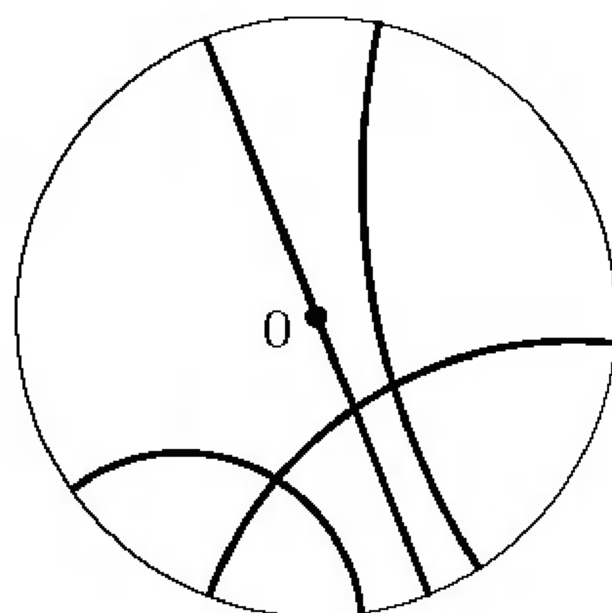
FIGURE 12.6. Hyperbolic geodesics.
