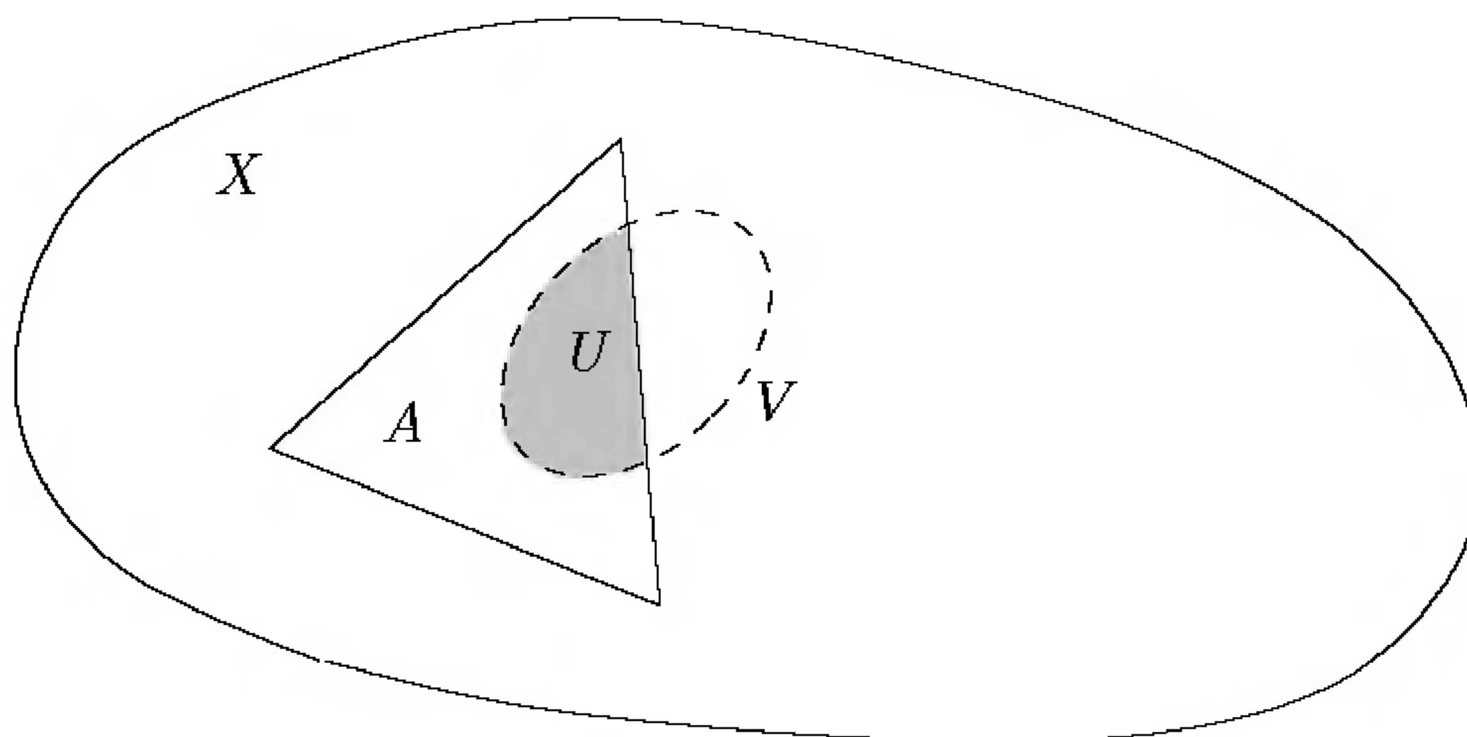
FIGURE 3.1. An open set in the subspace A .
