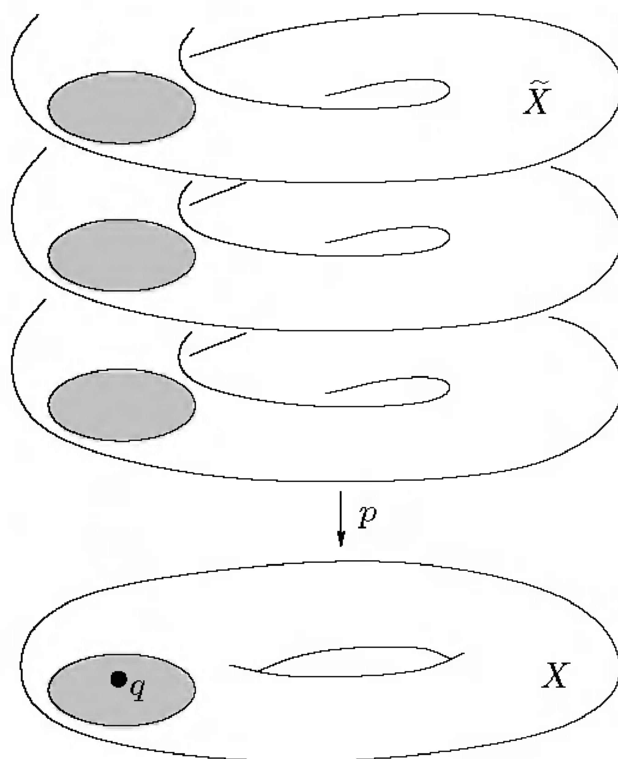
FIGURE 11.1. An evenly covered neighborhood of q .
