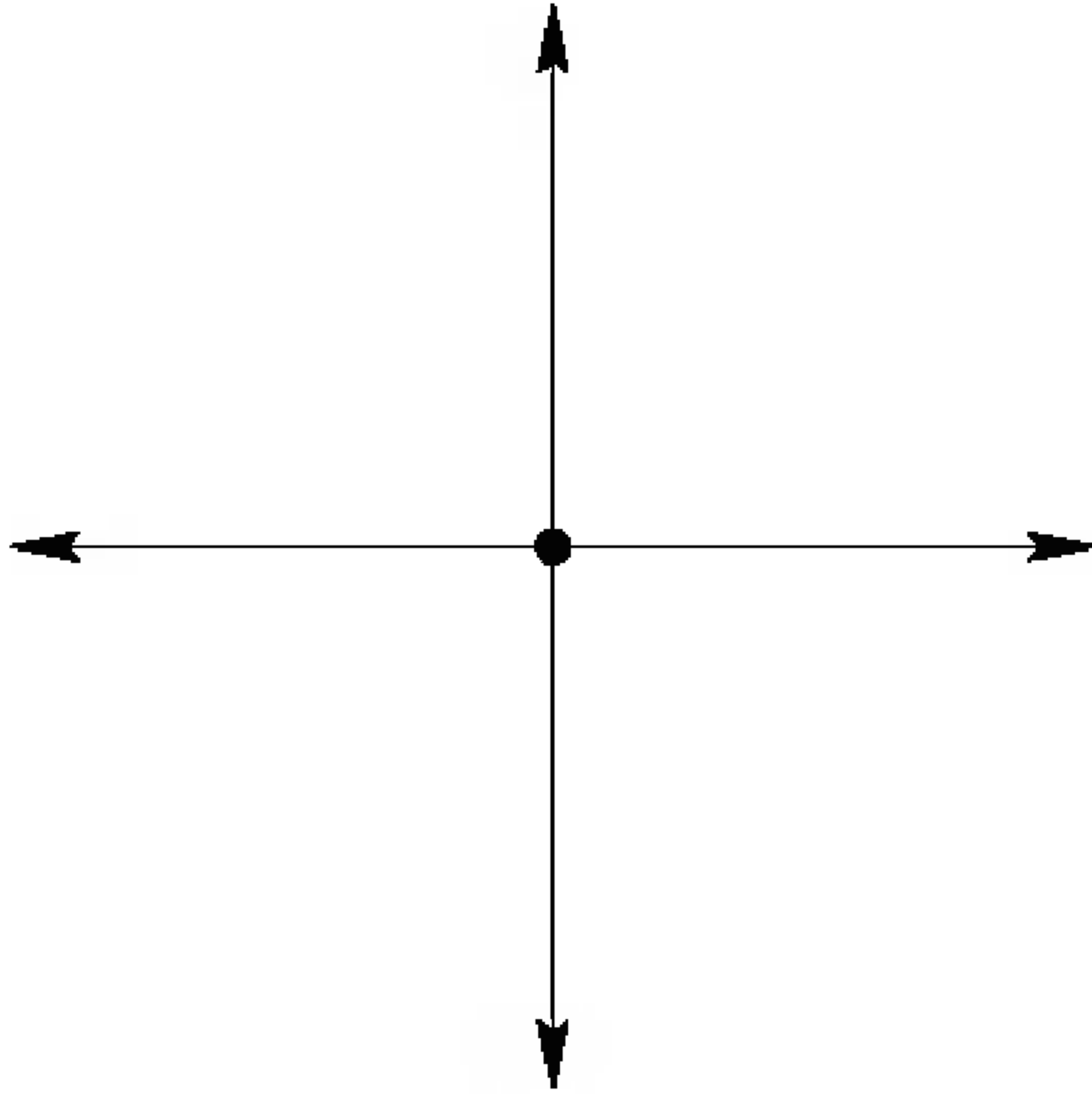
FIGURE 3.10. Wedge of two lines.
