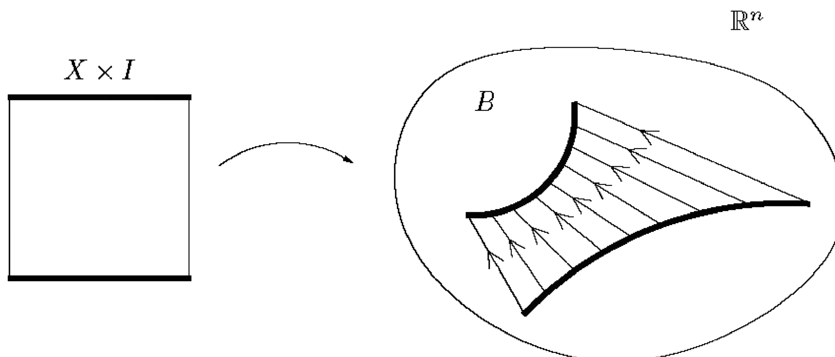
FIGURE 7.2. A straight-line homotopy.
