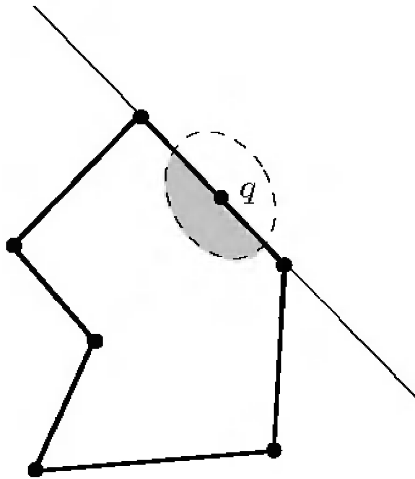
FIGURE 6.5. An edge point.
