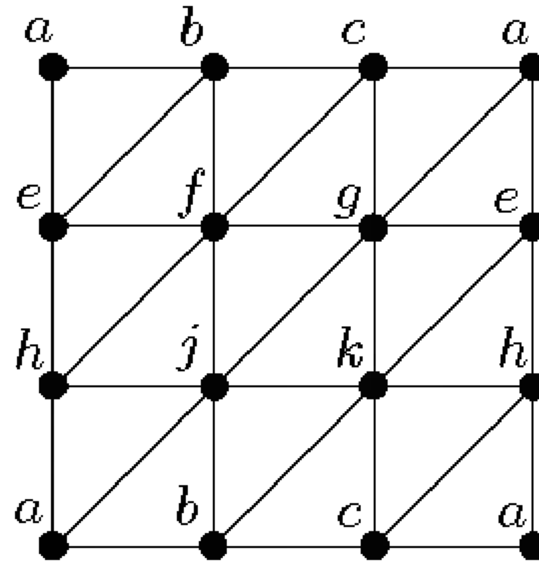
FIGURE 5.13. Triangulation of the torus.
