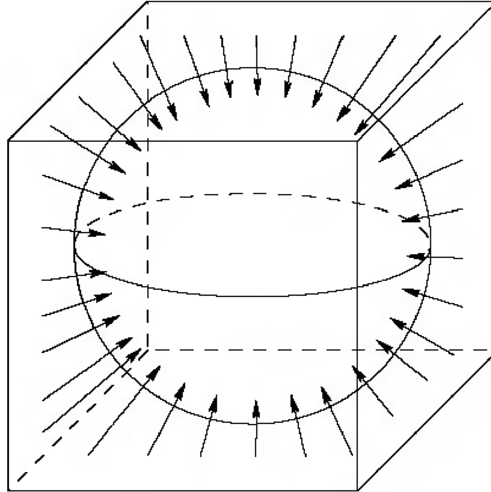
FIGURE 2.3. Deforming a cube into a sphere.
