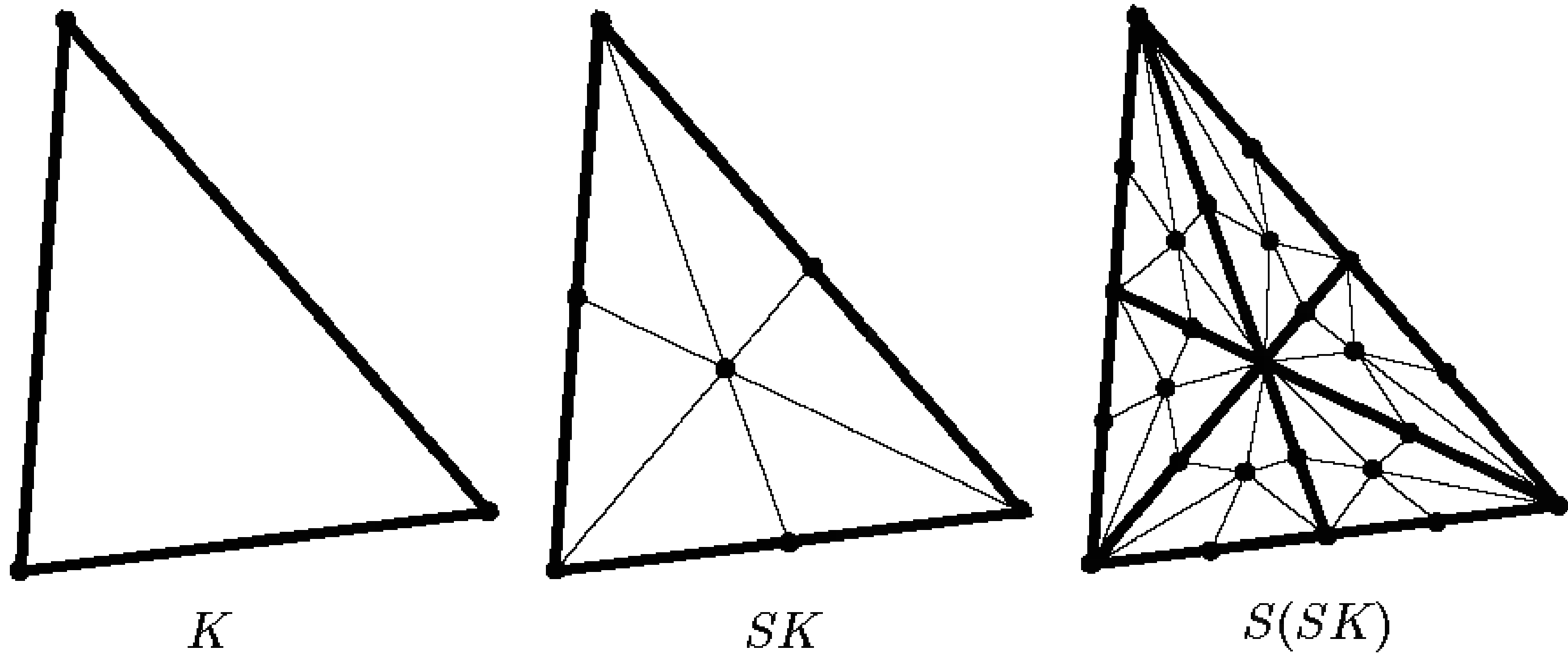
FIGURE 5.12. Barycentric subdivisions.
