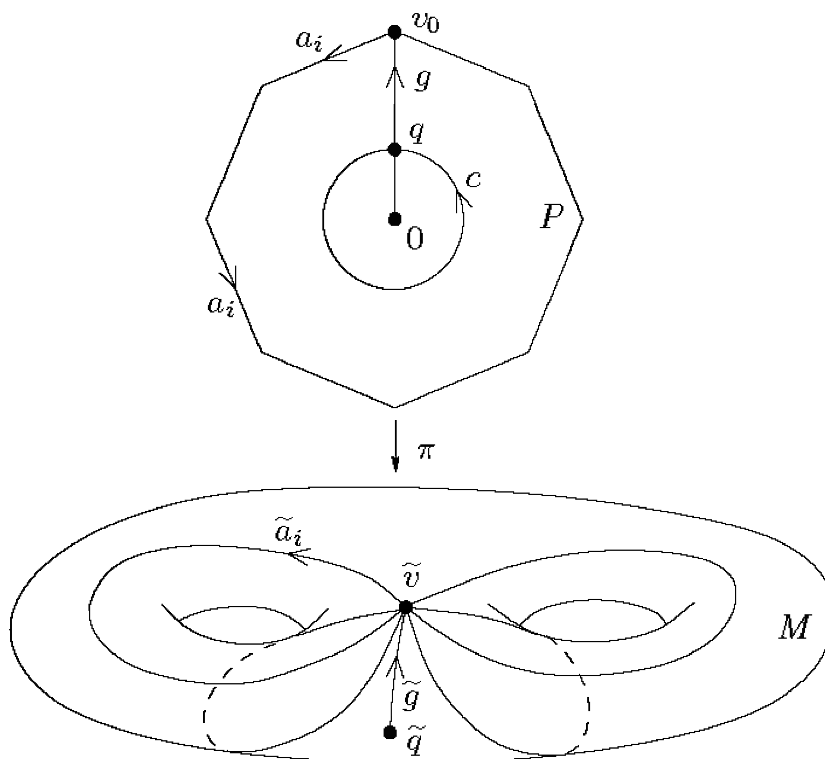
FIGURE 10.4. Proof of Proposition 10.9.
