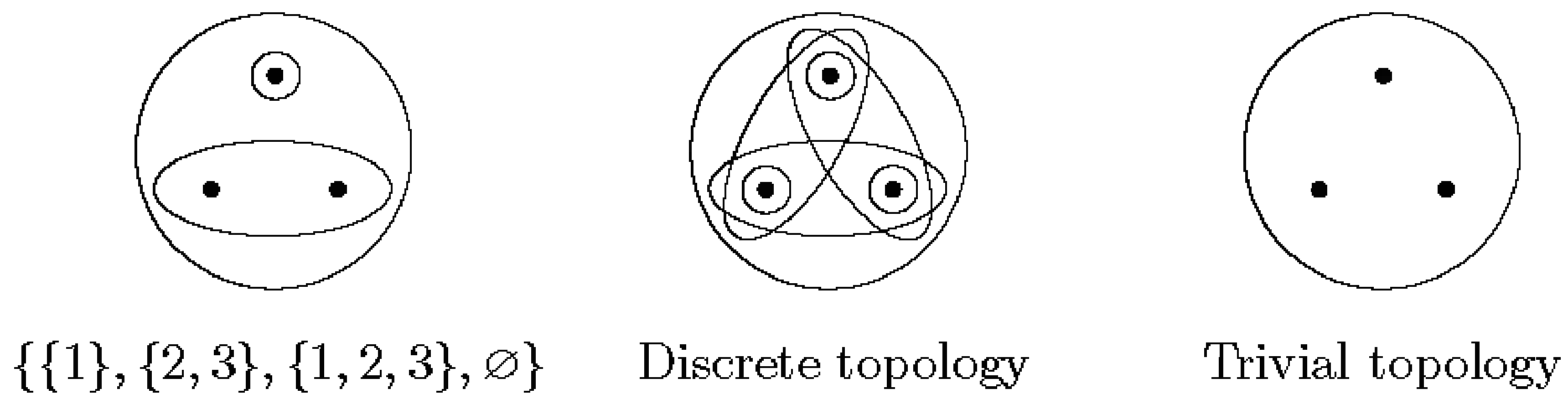
FIGURE 2.1. Topologies on \{1, 2, 3\} .
