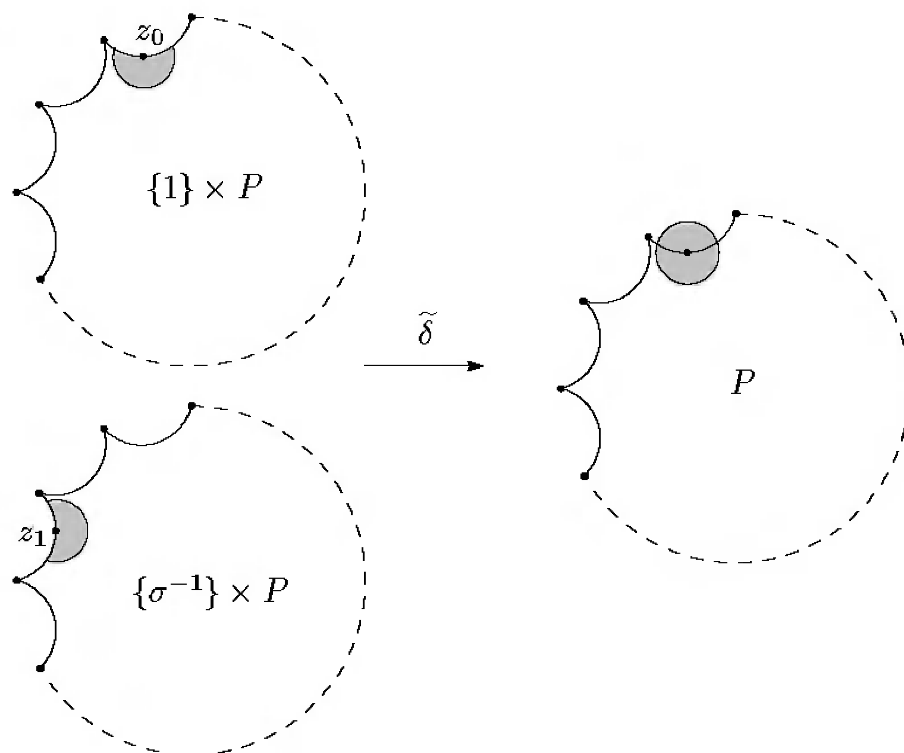
FIGURE 12.10. Hyperbolic neighborhood of an edge point.
