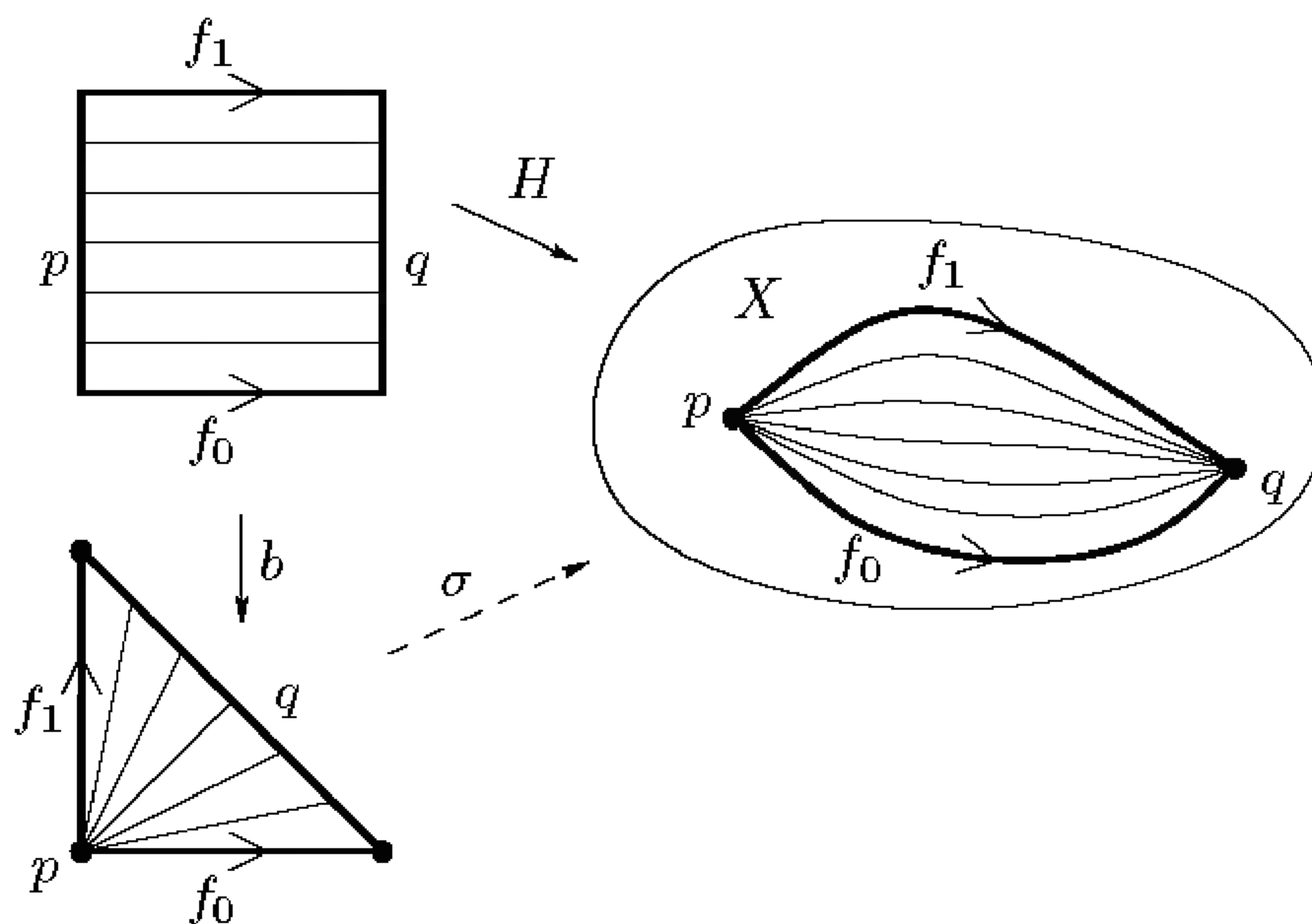
FIGURE 13.5. Path homotopic paths differ by a boundary.
