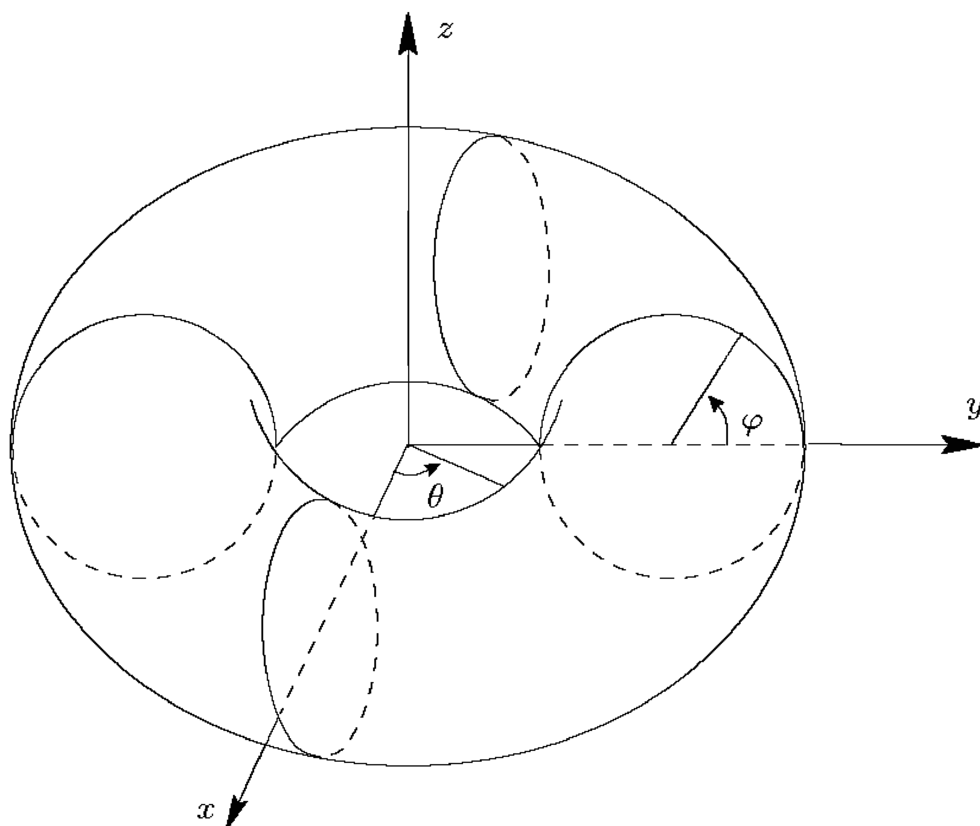
FIGURE 3.7. A doughnut surface of revolution.
