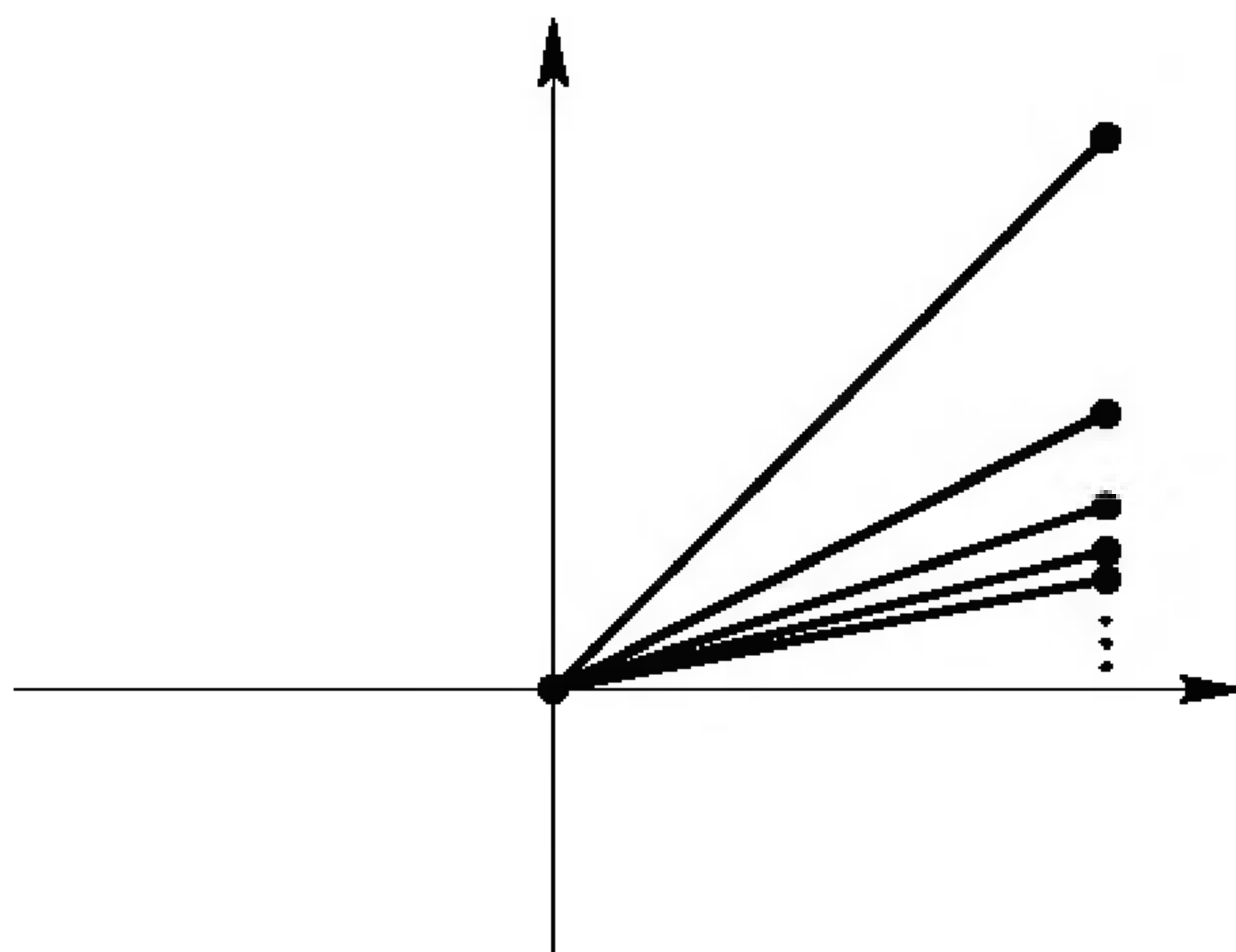
FIGURE 5.4. Failure of local finiteness.
