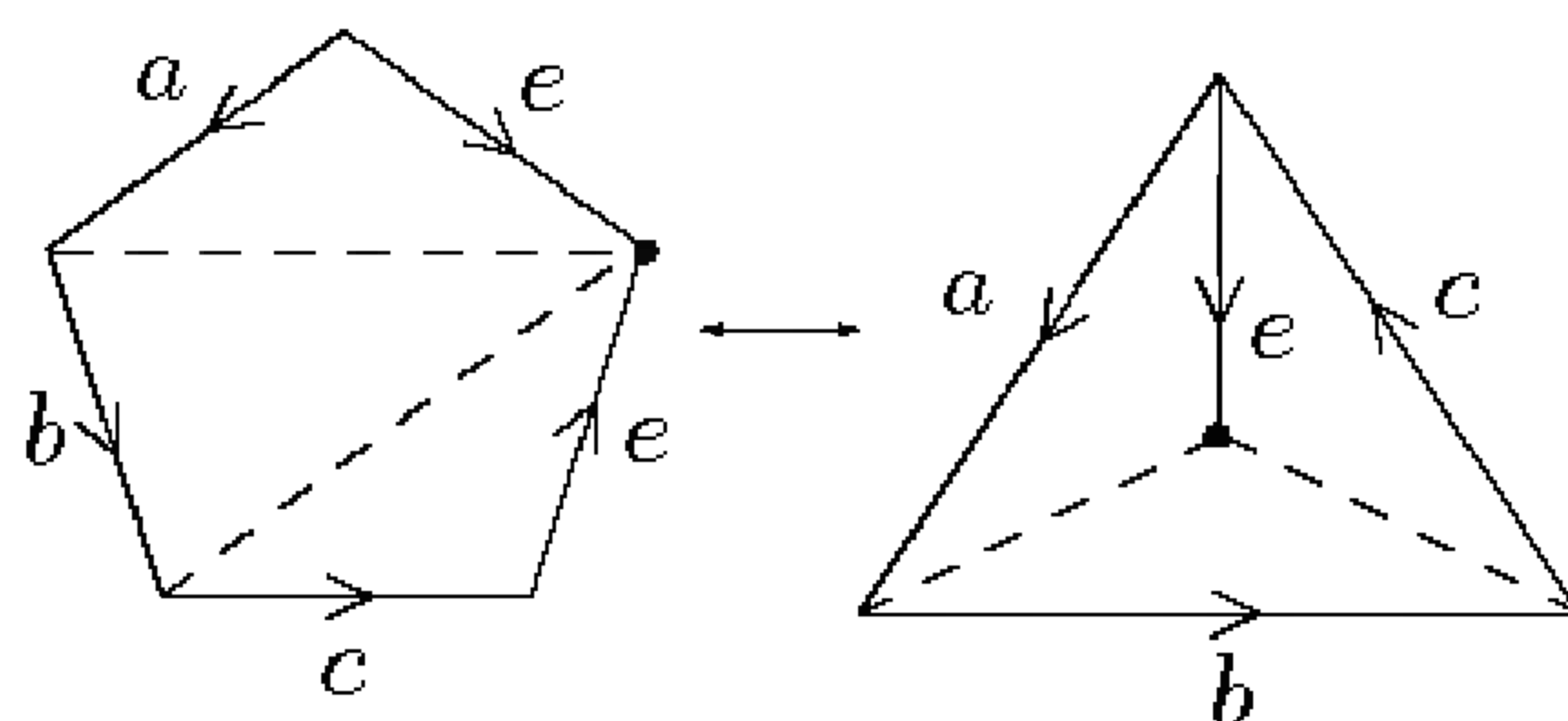
FIGURE 6.21. Folding/unfolding.
