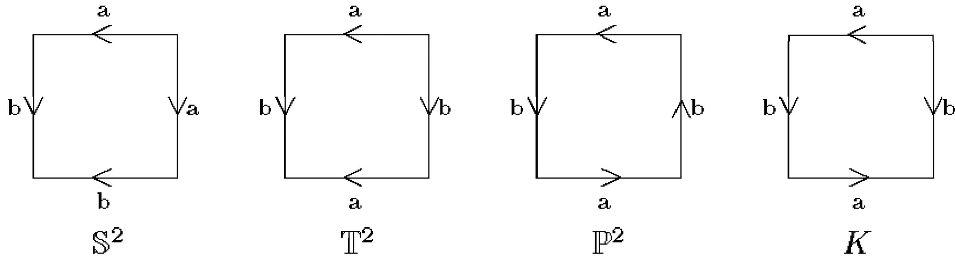
FIGURE 6.17. Standard presentations.
