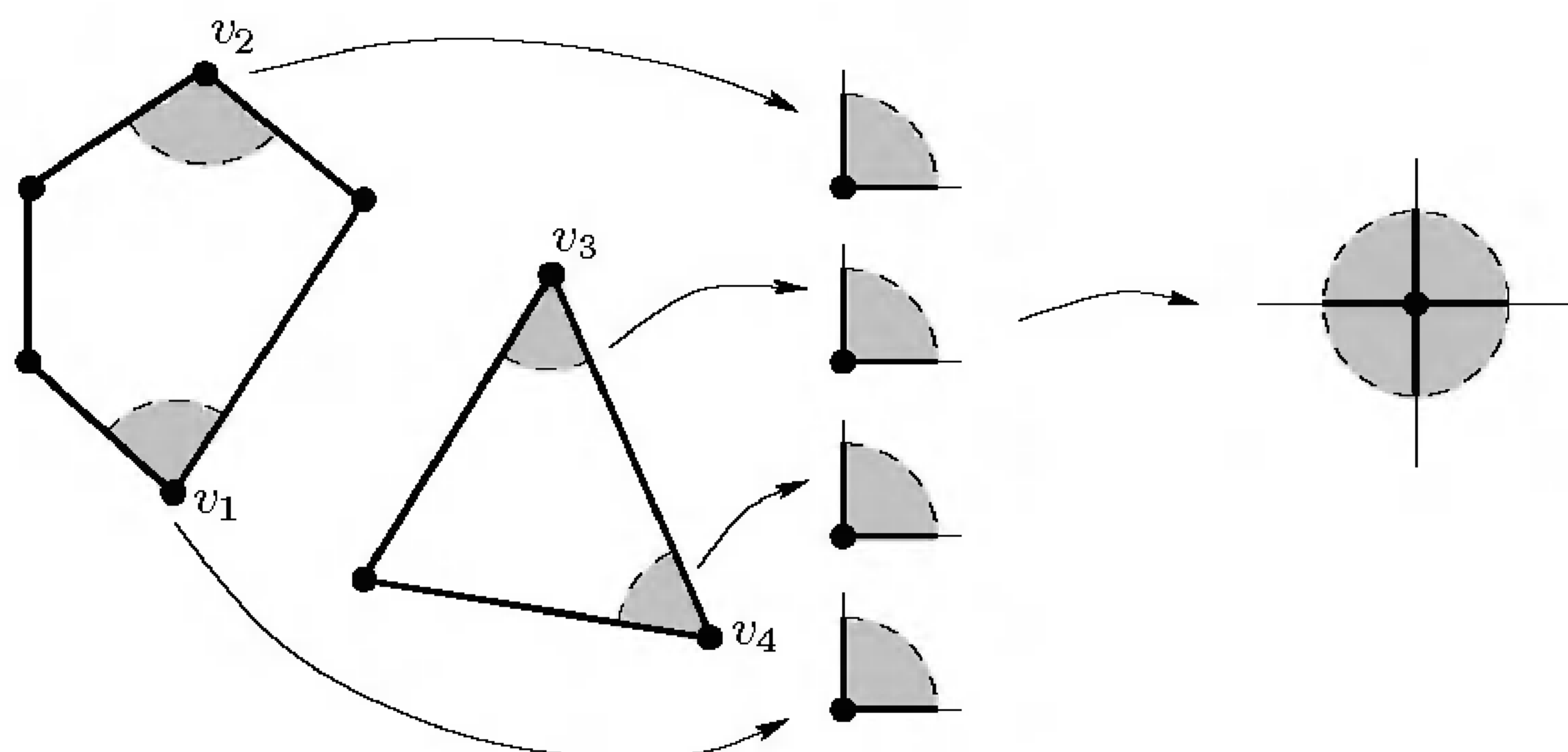
FIGURE 6.8. Euclidean neighborhood of a vertex point.
