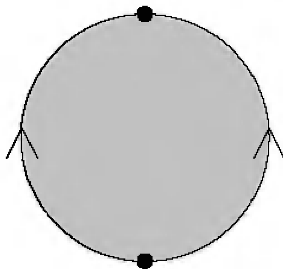
FIGURE 3.8. A quotient of \overline{\mathbb{B}^2} .
