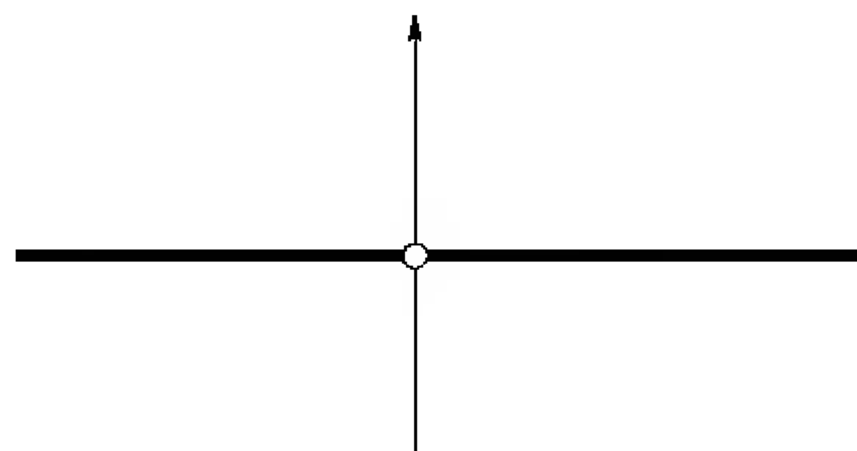
FIGURE 4.2. The x -axis minus 0.
