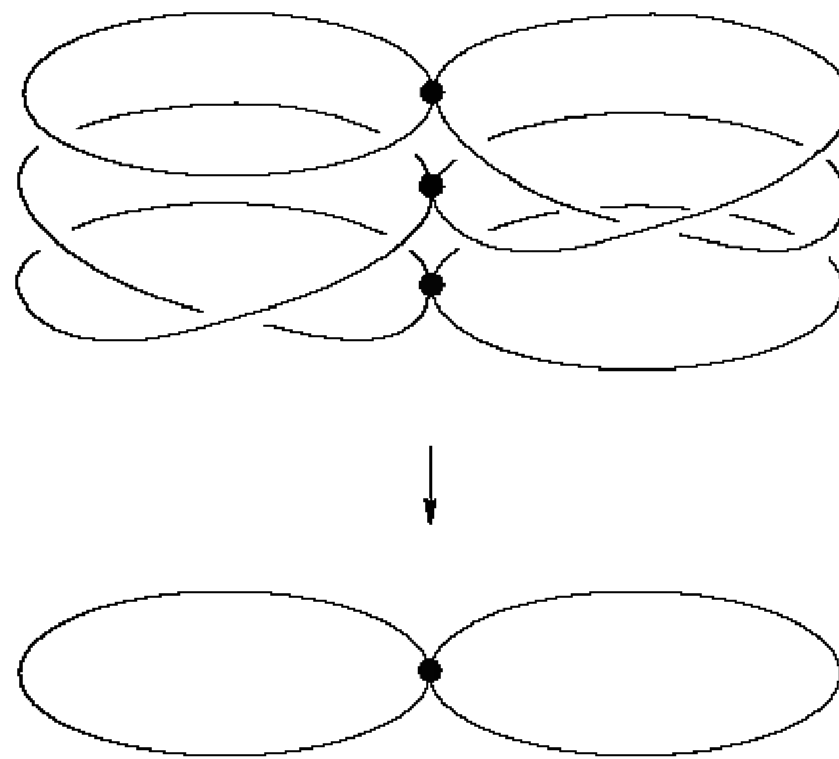
FIGURE 11.10. The covering map of Problem 11-14.
