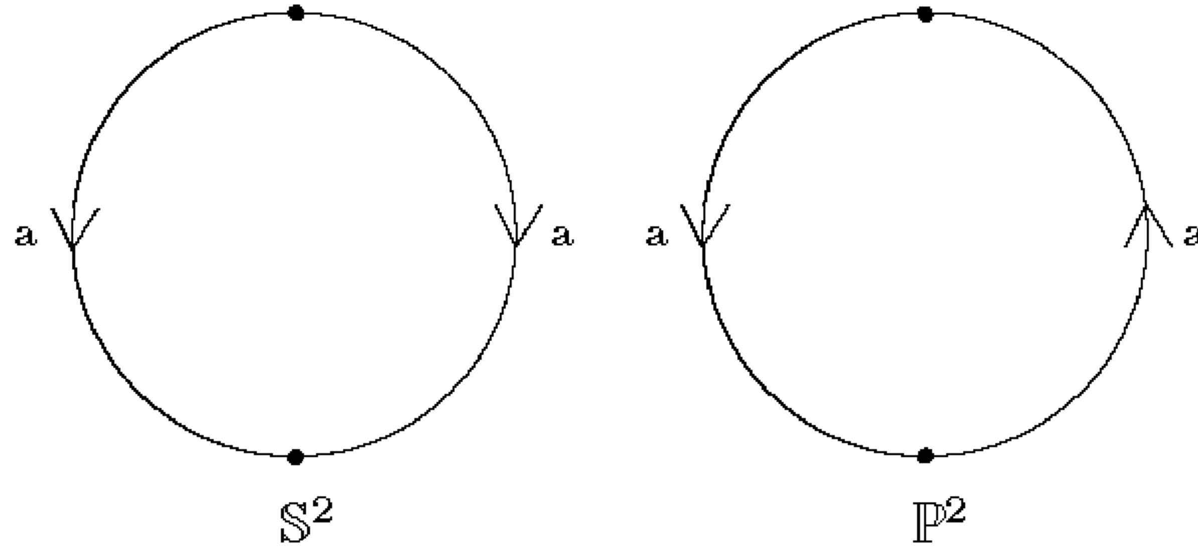
FIGURE 6.15. Presentations of S^2 and \mathbb{P}^2 .
