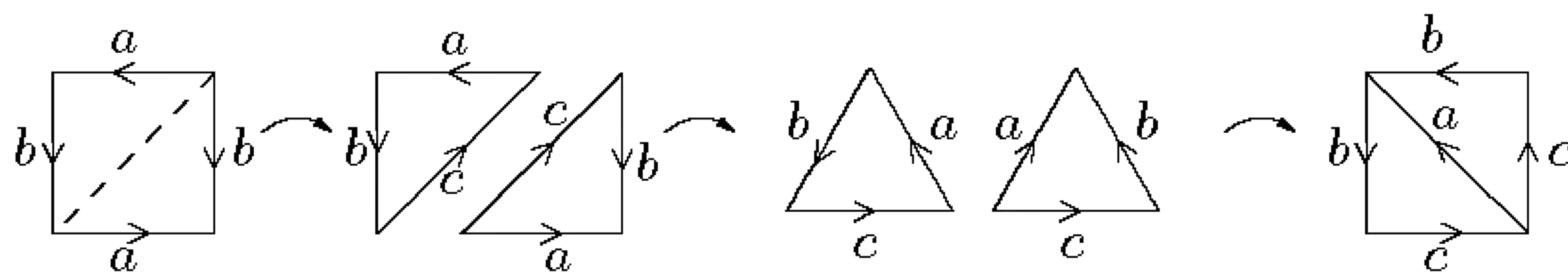
FIGURE 6.24. Transforming the Klein bottle to \mathbb{P}^2 \# \mathbb{P}^2 .
