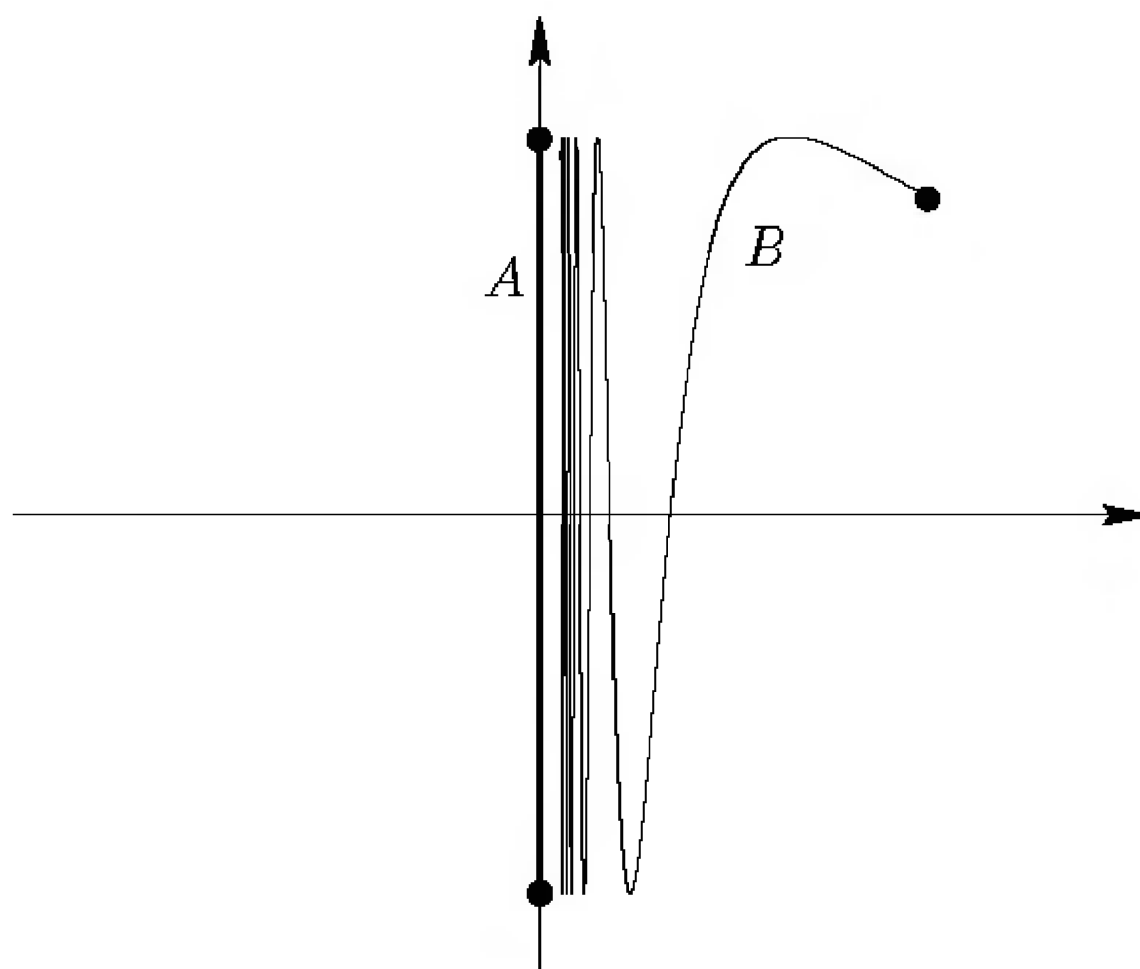
FIGURE 4.4. The topologists's sine curve.
