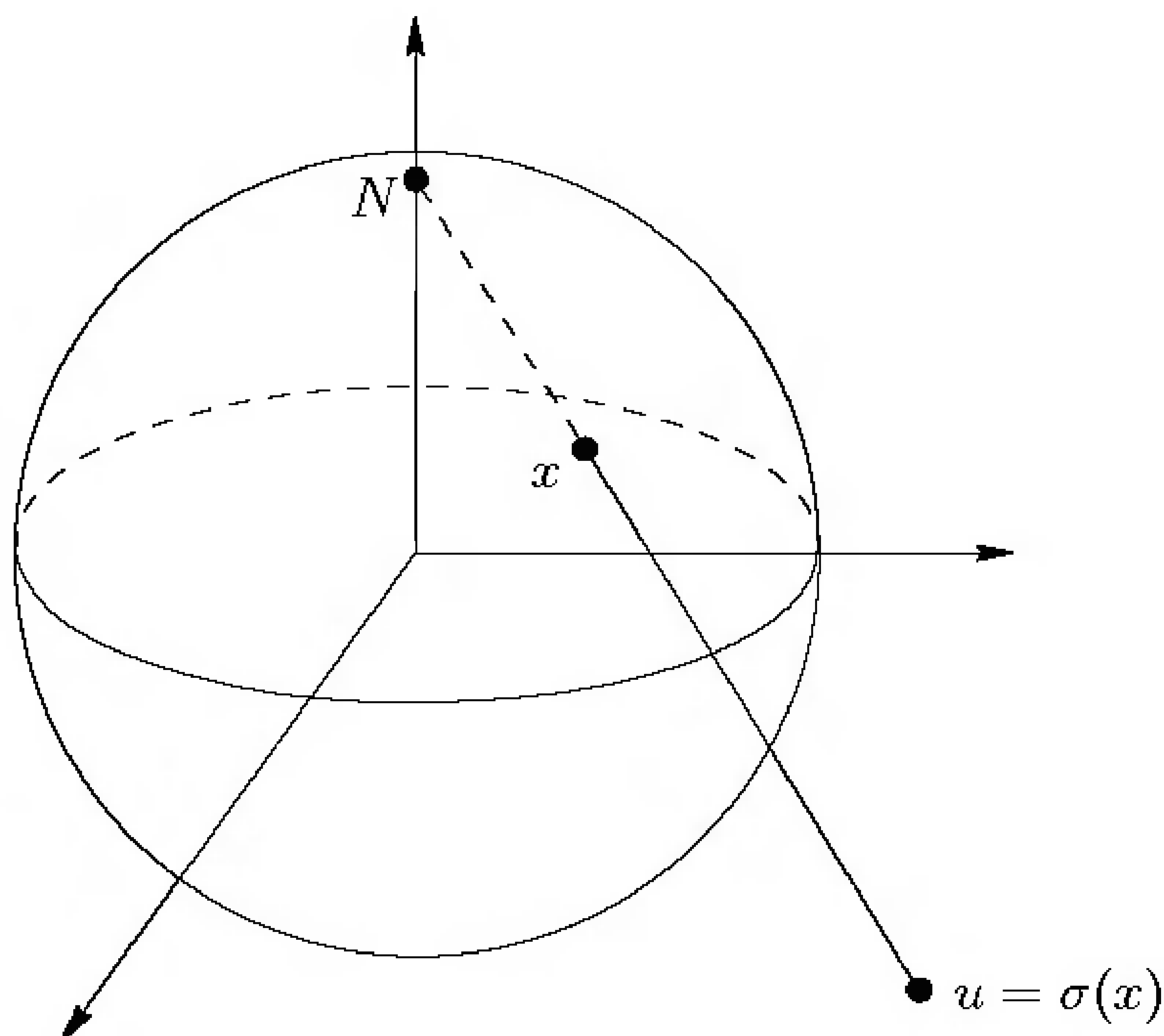
FIGURE 3.6. Stereographic projection.
