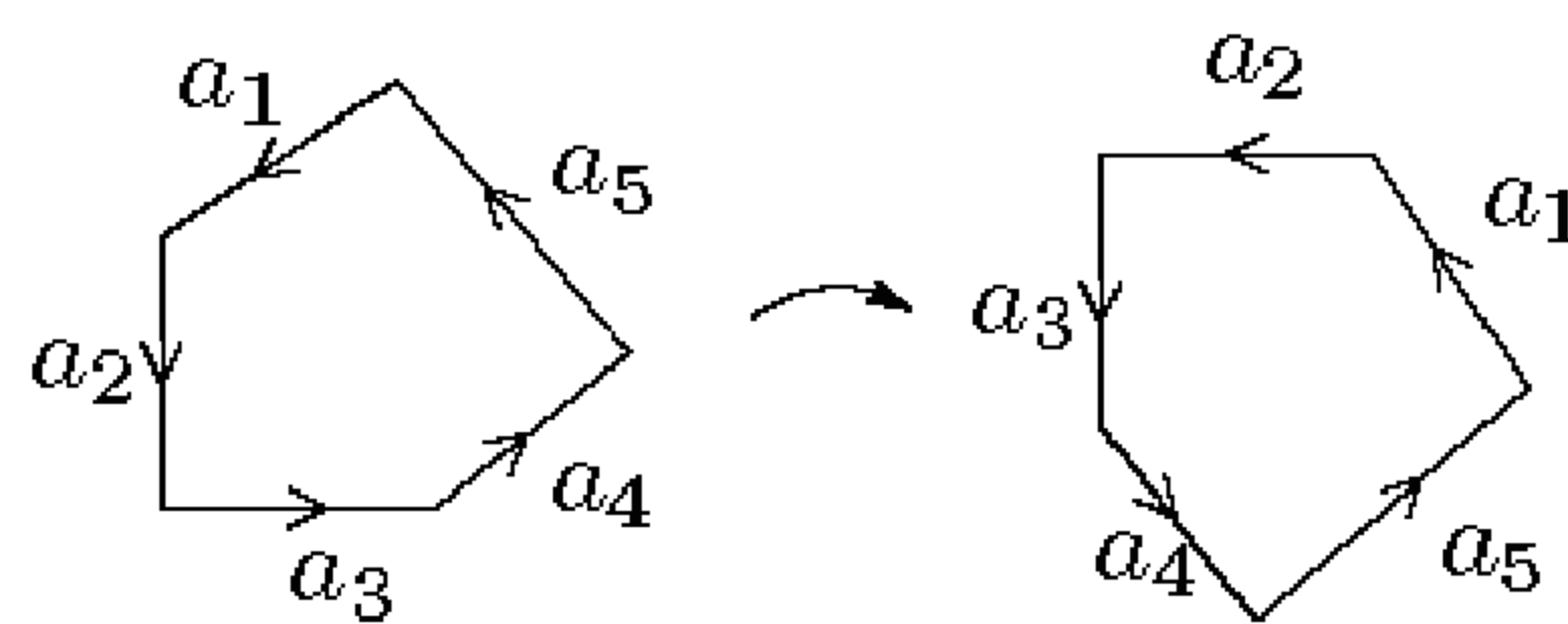
FIGURE 6.19. Rotating.
