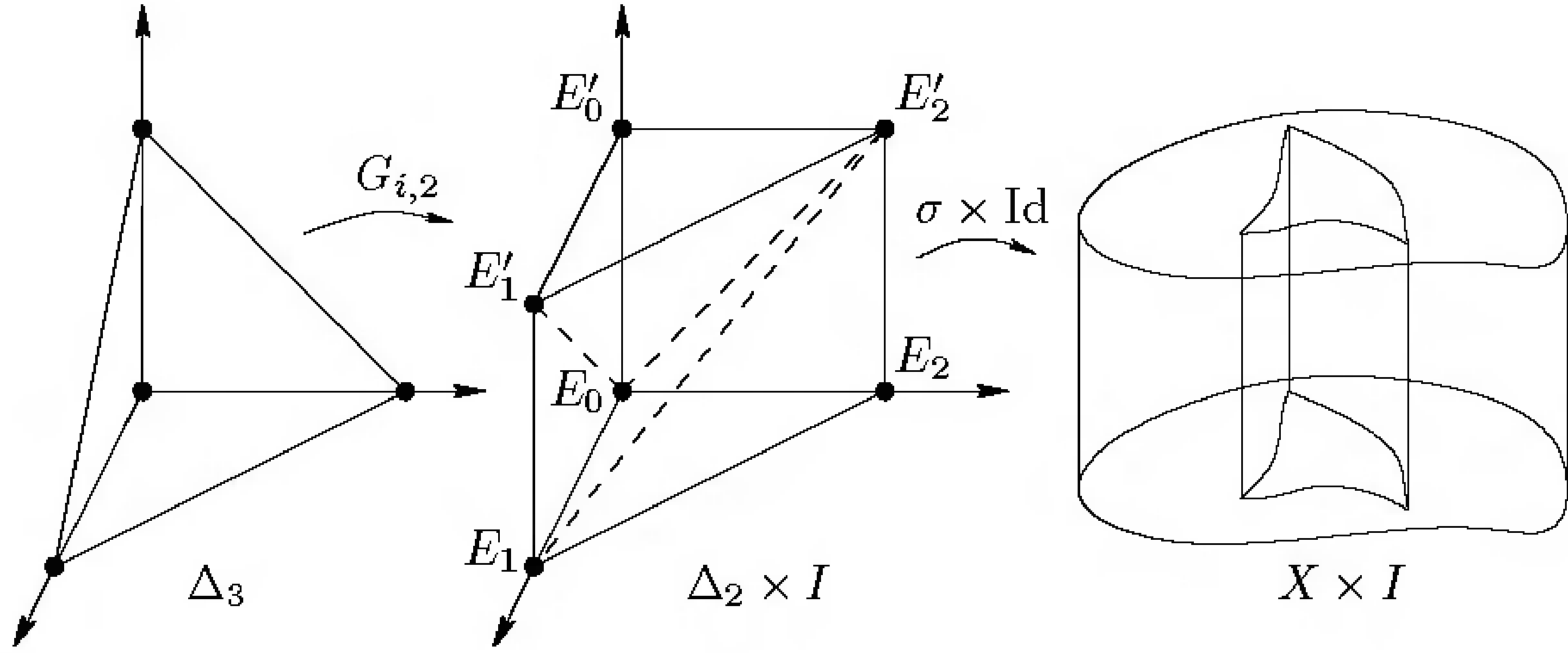
FIGURE 13.4. The operator h in dimension 2.
