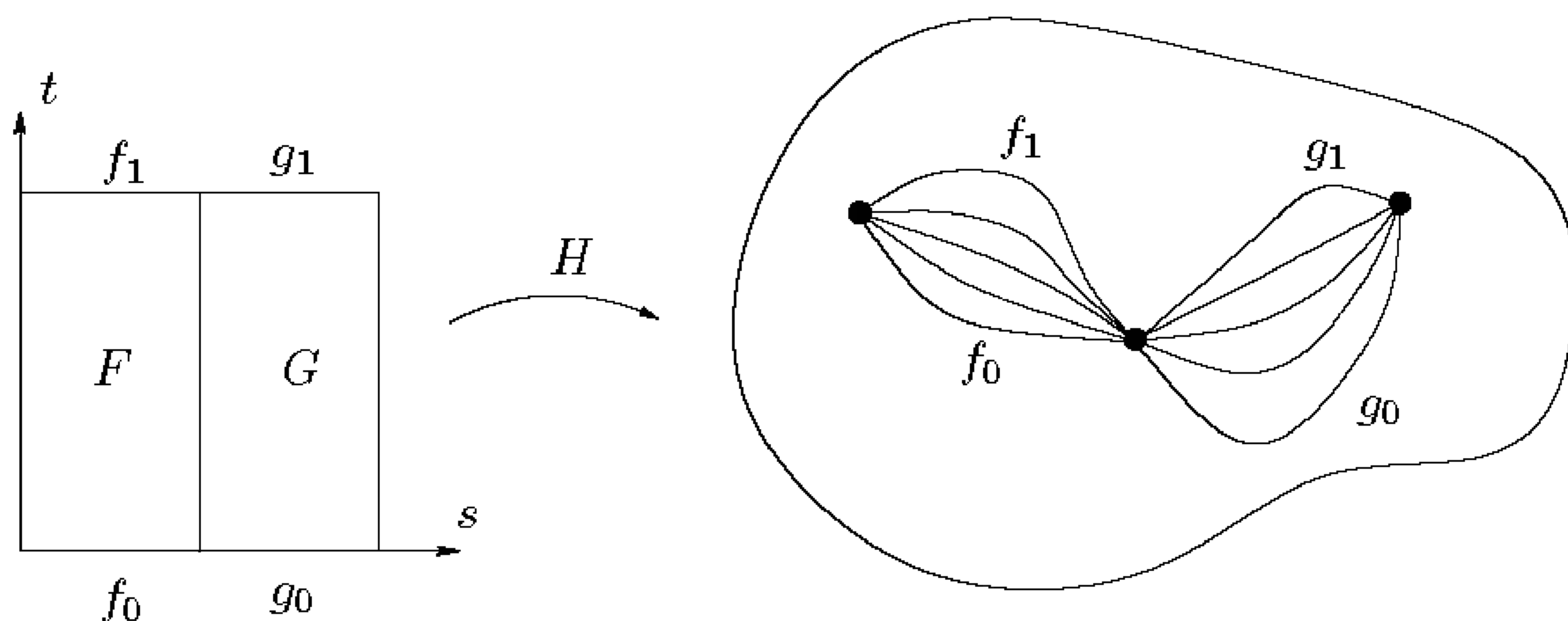
FIGURE 7.3. Homotopy invariance of path multiplication.
