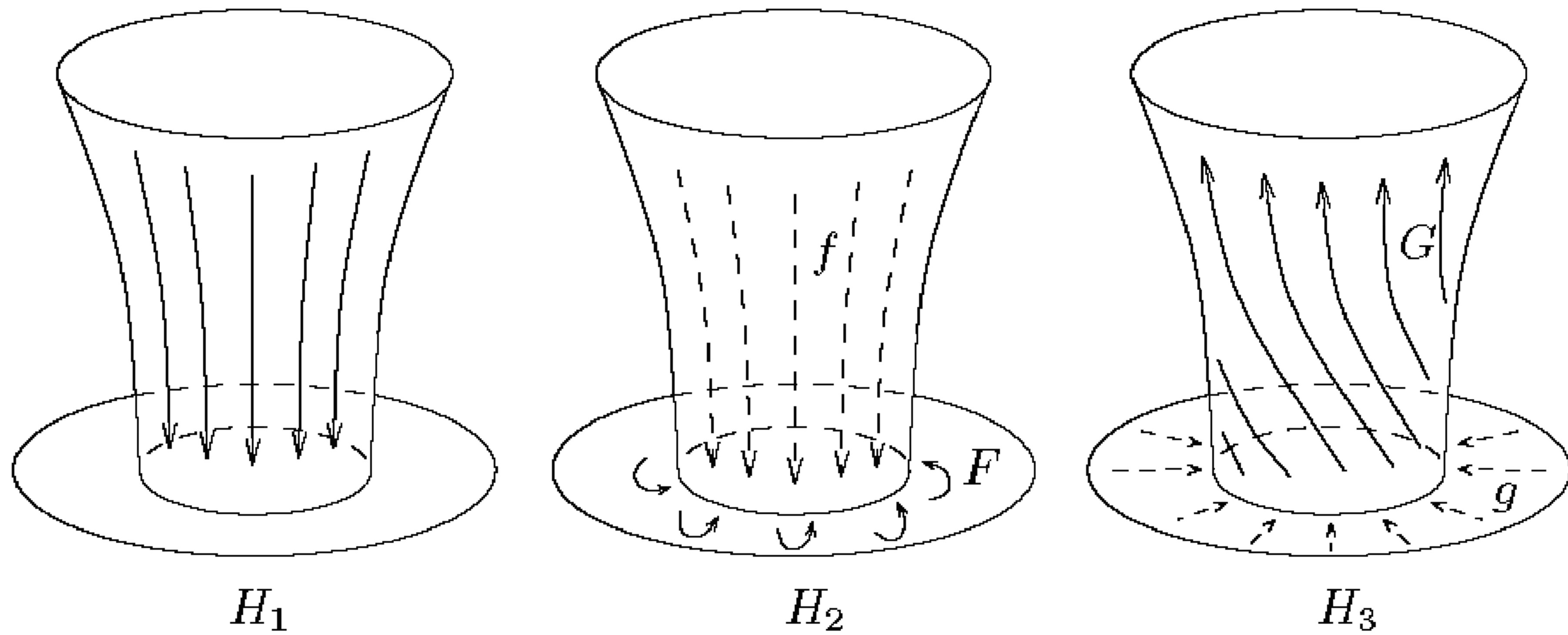
FIGURE 7.19. Homotopies of the mapping cylinder.
