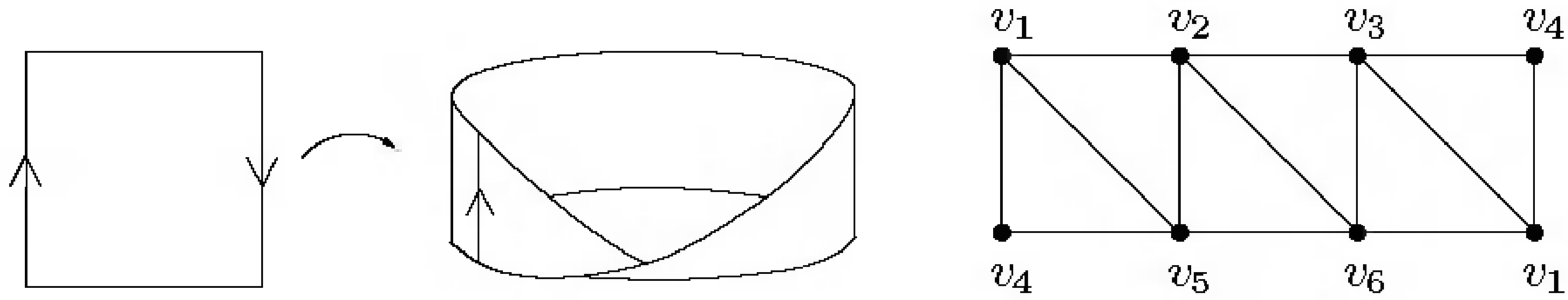
FIGURE 5.7. The Möbius band.
