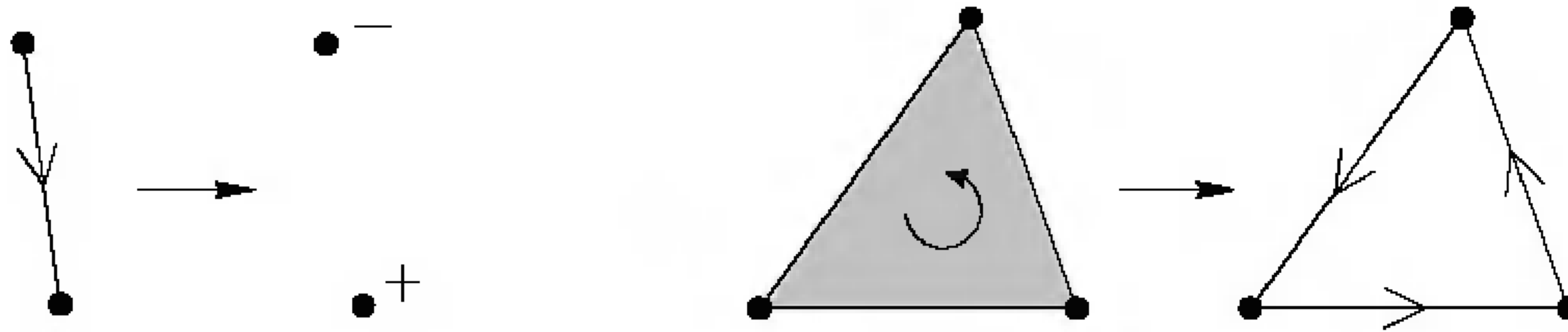
FIGURE 5.9. Induced orientations of boundary faces.
