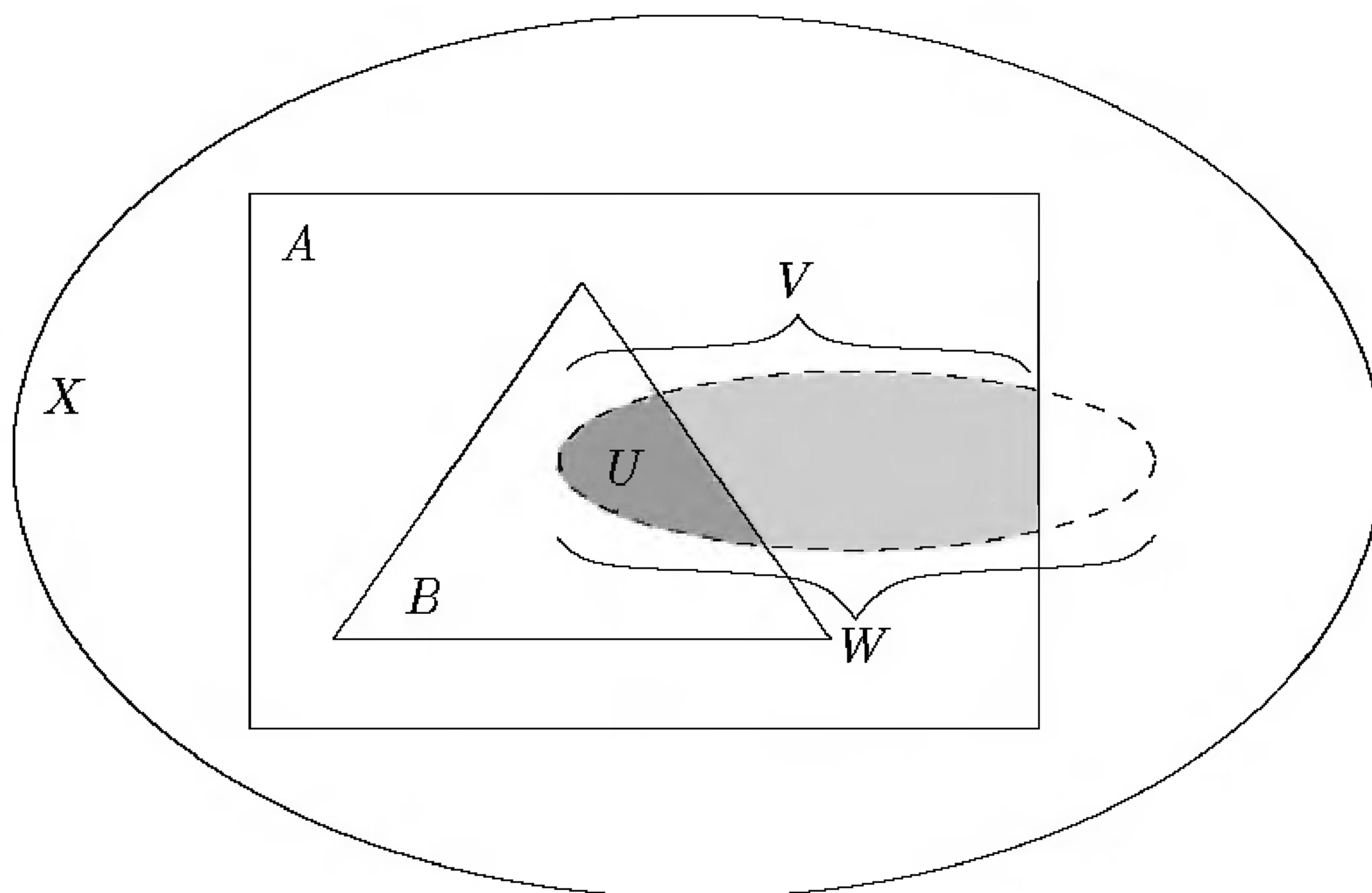
FIGURE 3.3. A subspace of a subspace.
