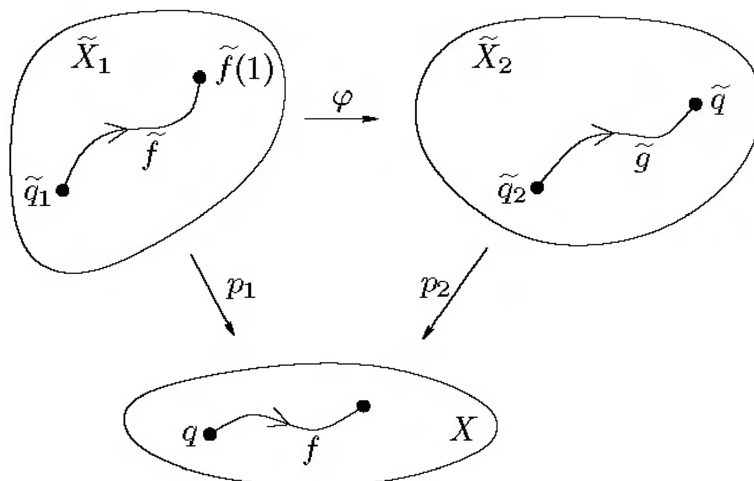
FIGURE 12.1. Proof that a covering homomorphism is surjective.
