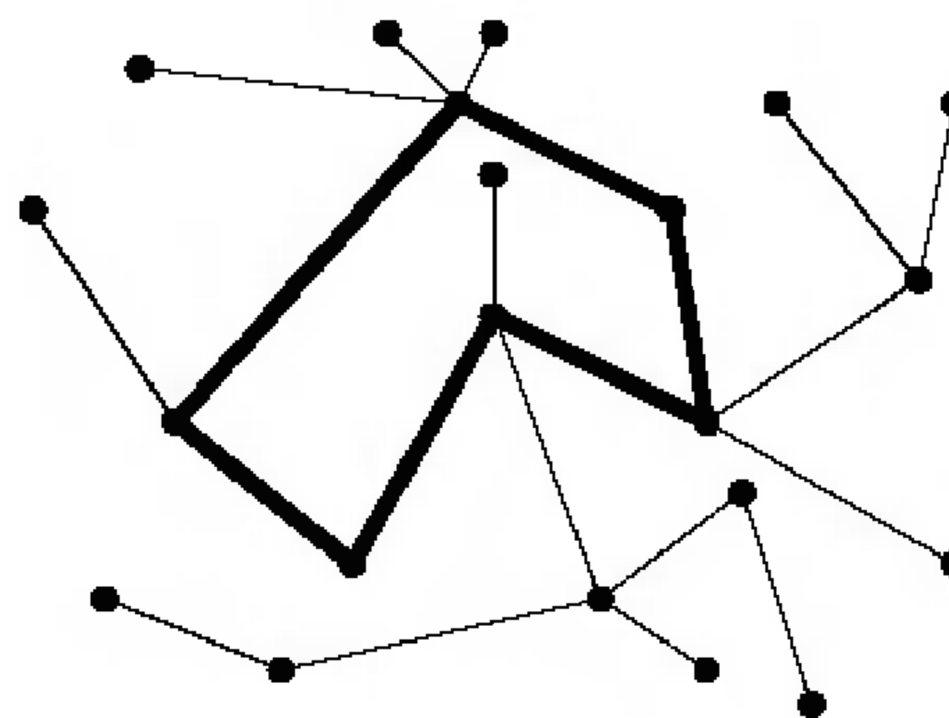
FIGURE 7.15. Not a tree.
