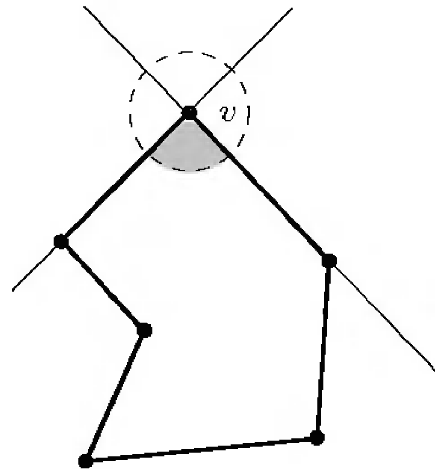
FIGURE 6.6. A vertex.
