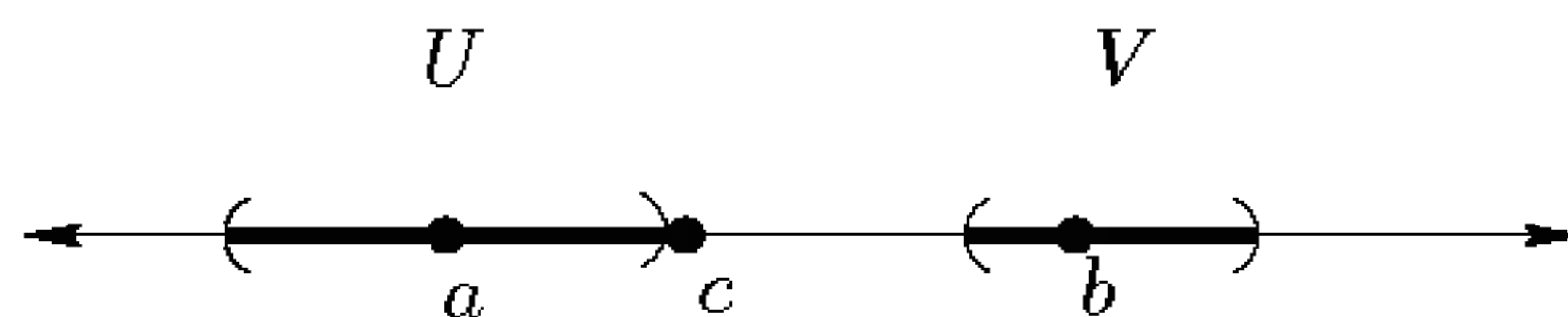
FIGURE 4.3. Proof that an interval is connected.
