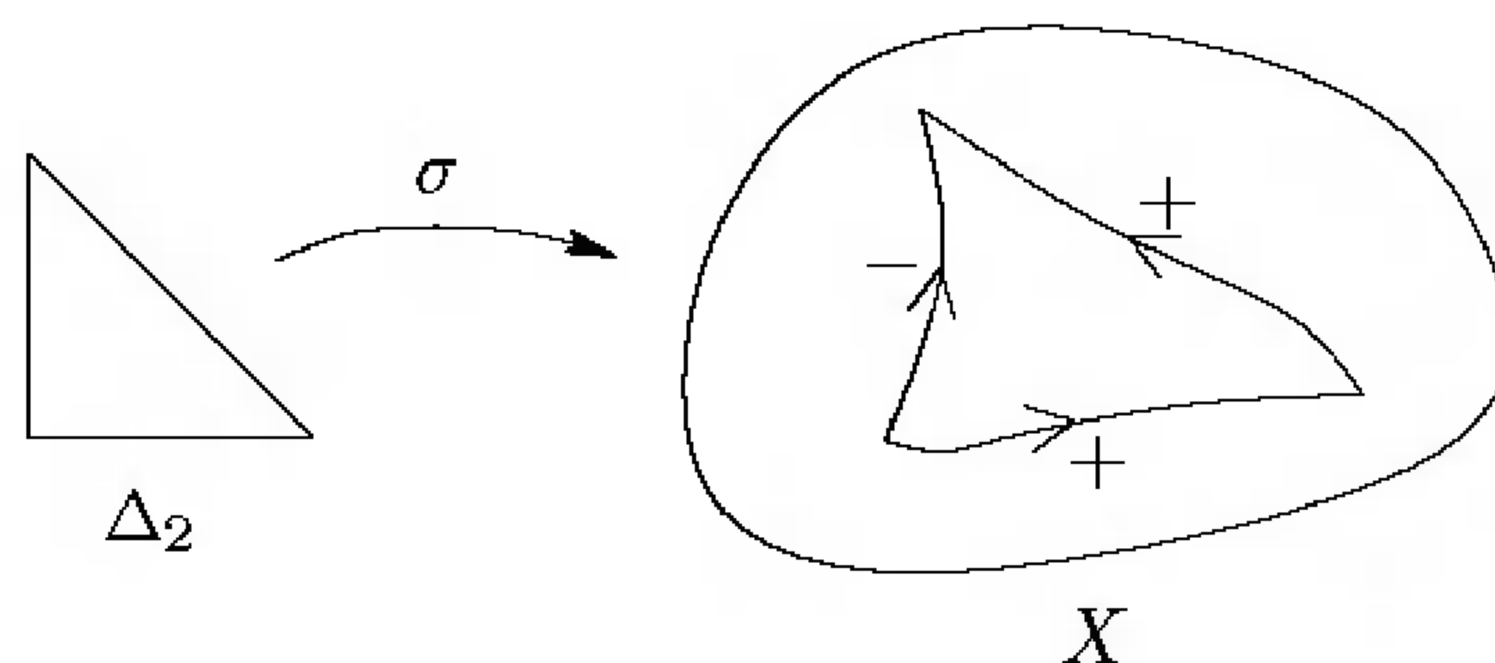
FIGURE 13.2. The boundary of a singular 2-simplex.
