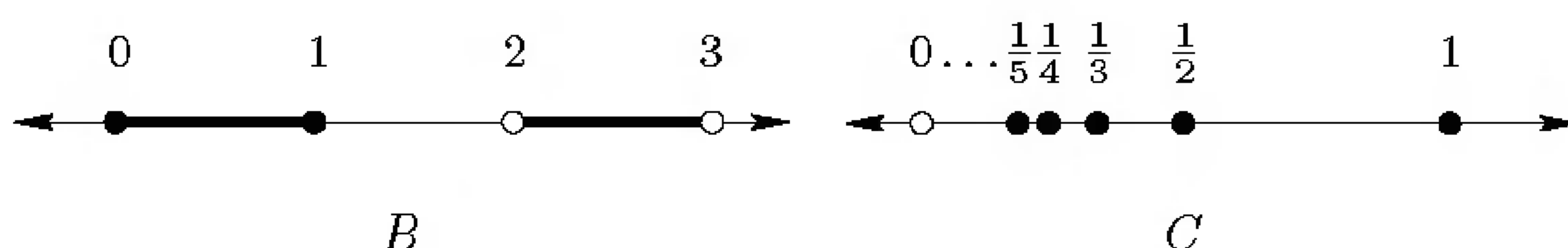
FIGURE 3.2. Subspaces of \mathbb{R} .
