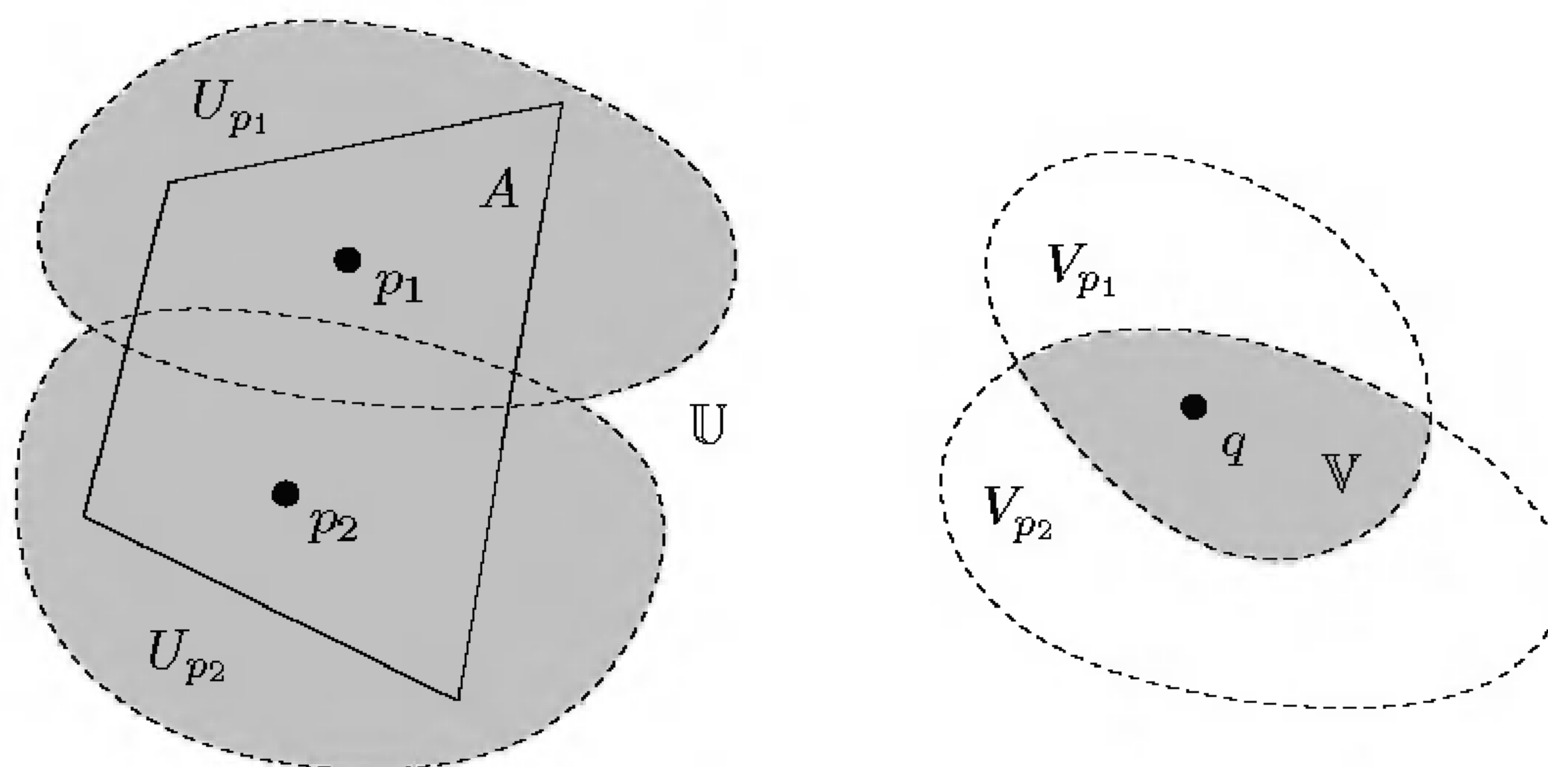
FIGURE 4.5. The case B = \{q\} .
