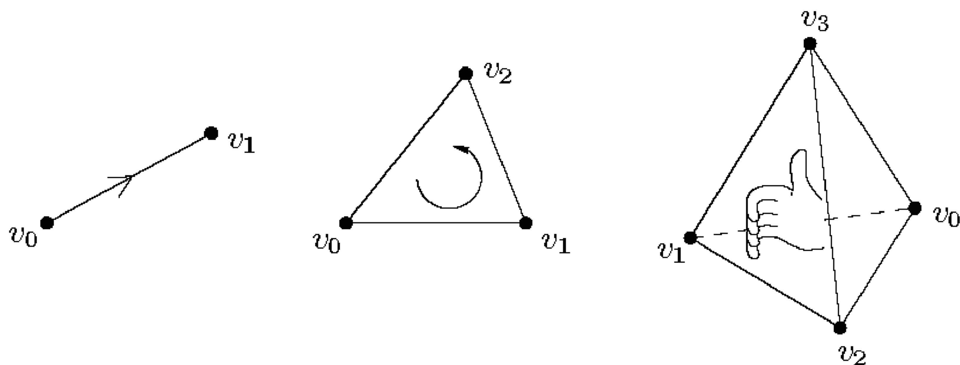
FIGURE 5.8. Orientations of simplices.
