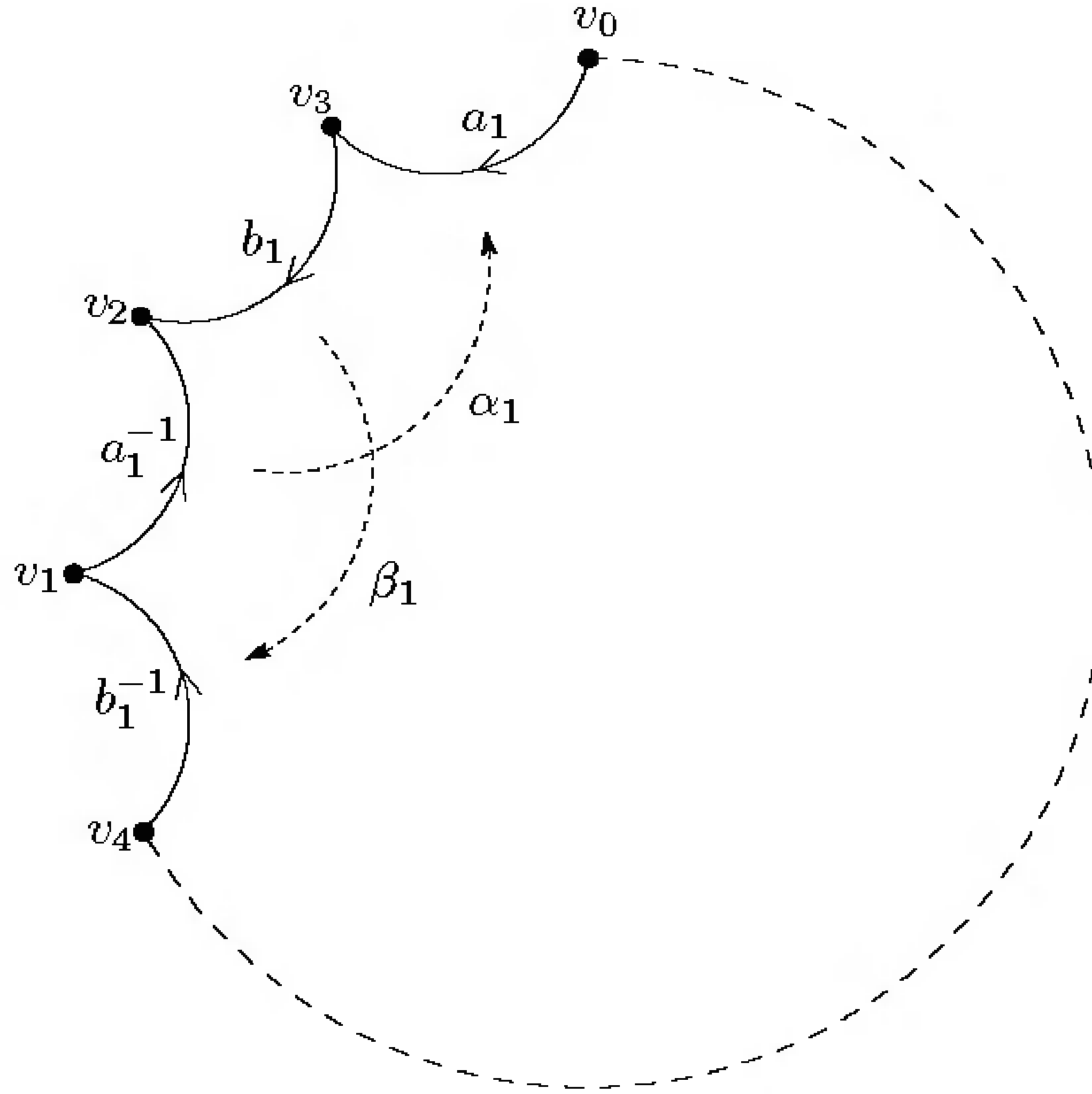
FIGURE 12.8. Edge pairing transformations.
