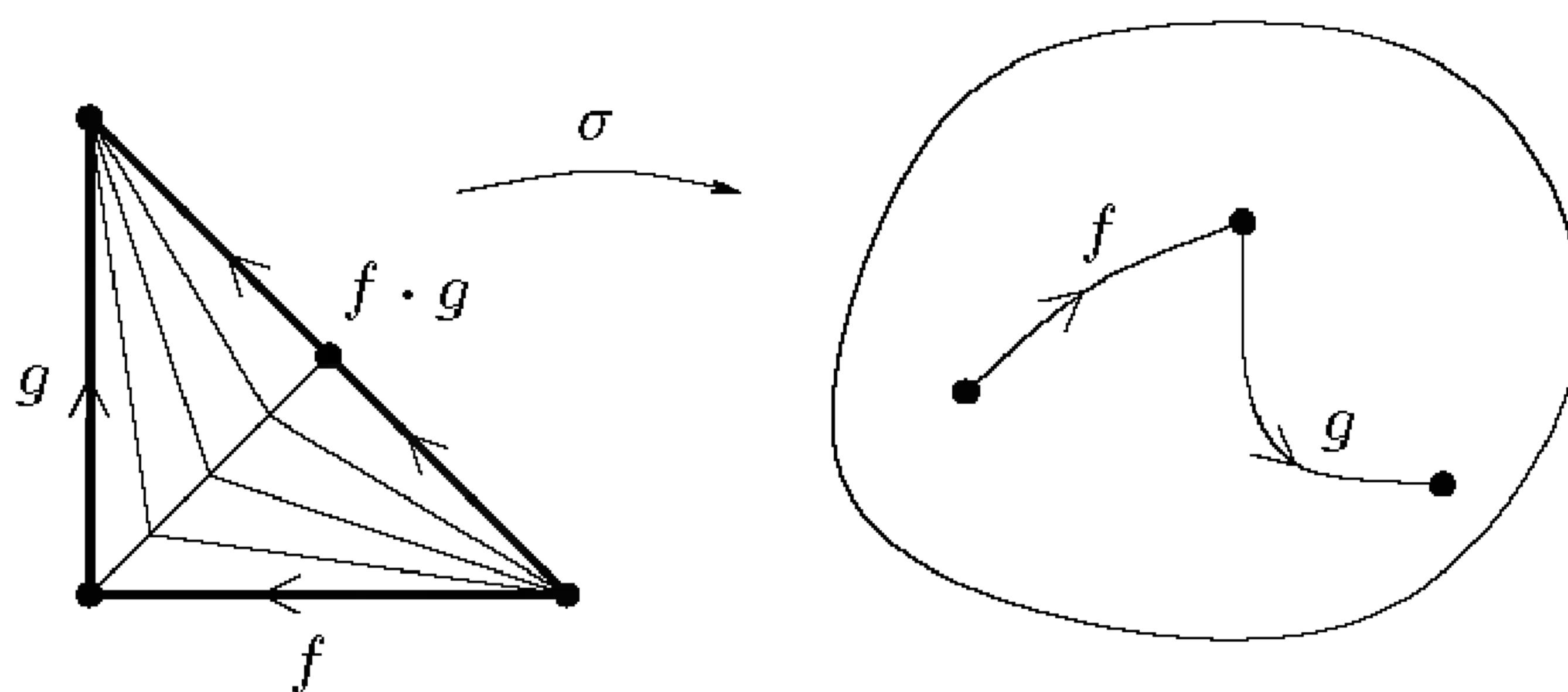
FIGURE 13.7. Proof that \gamma is a homomorphism.
