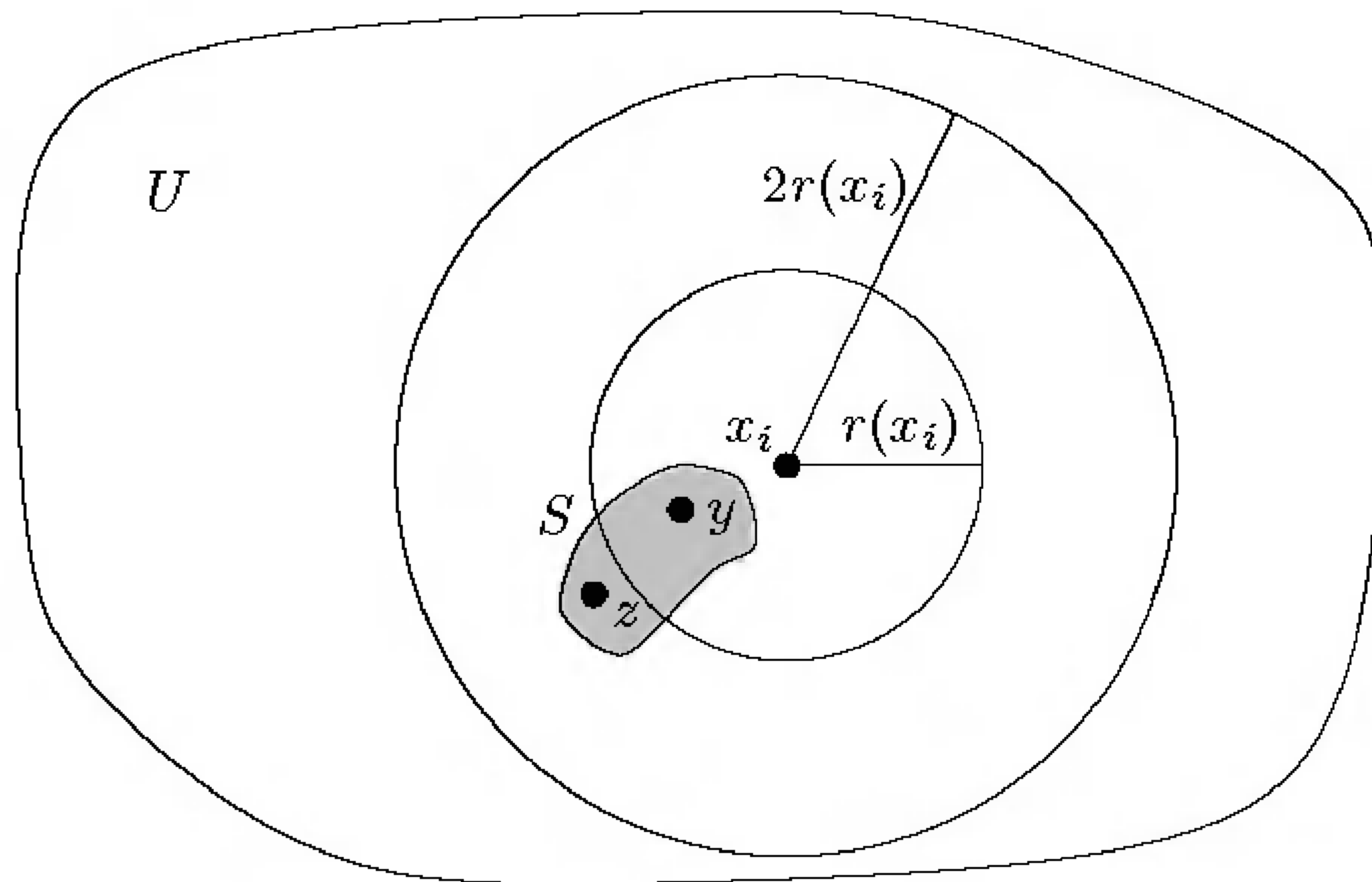
FIGURE 4.7. Proof of the Lebesgue number lemma.
