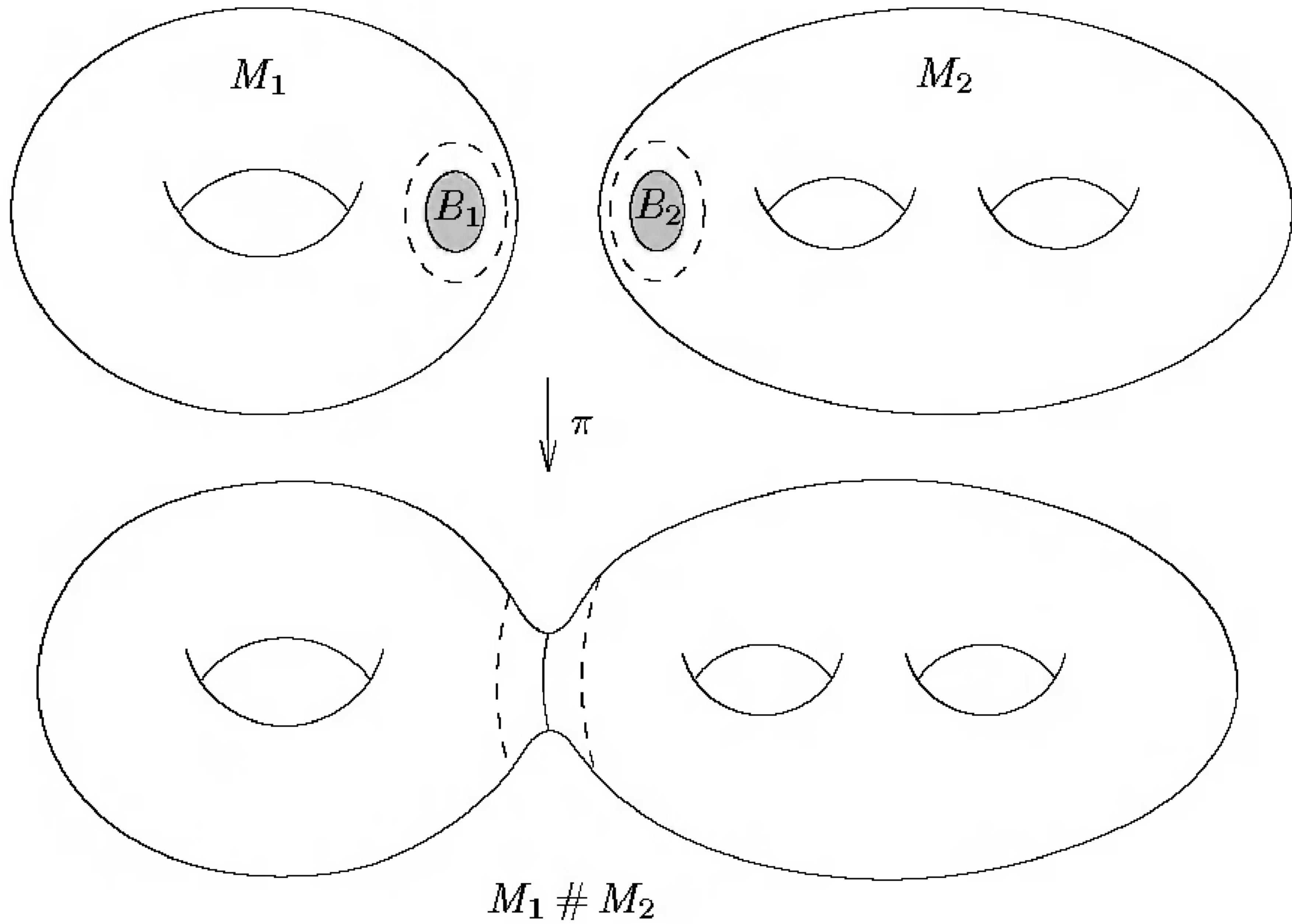
FIGURE 6.10. A connected sum.
