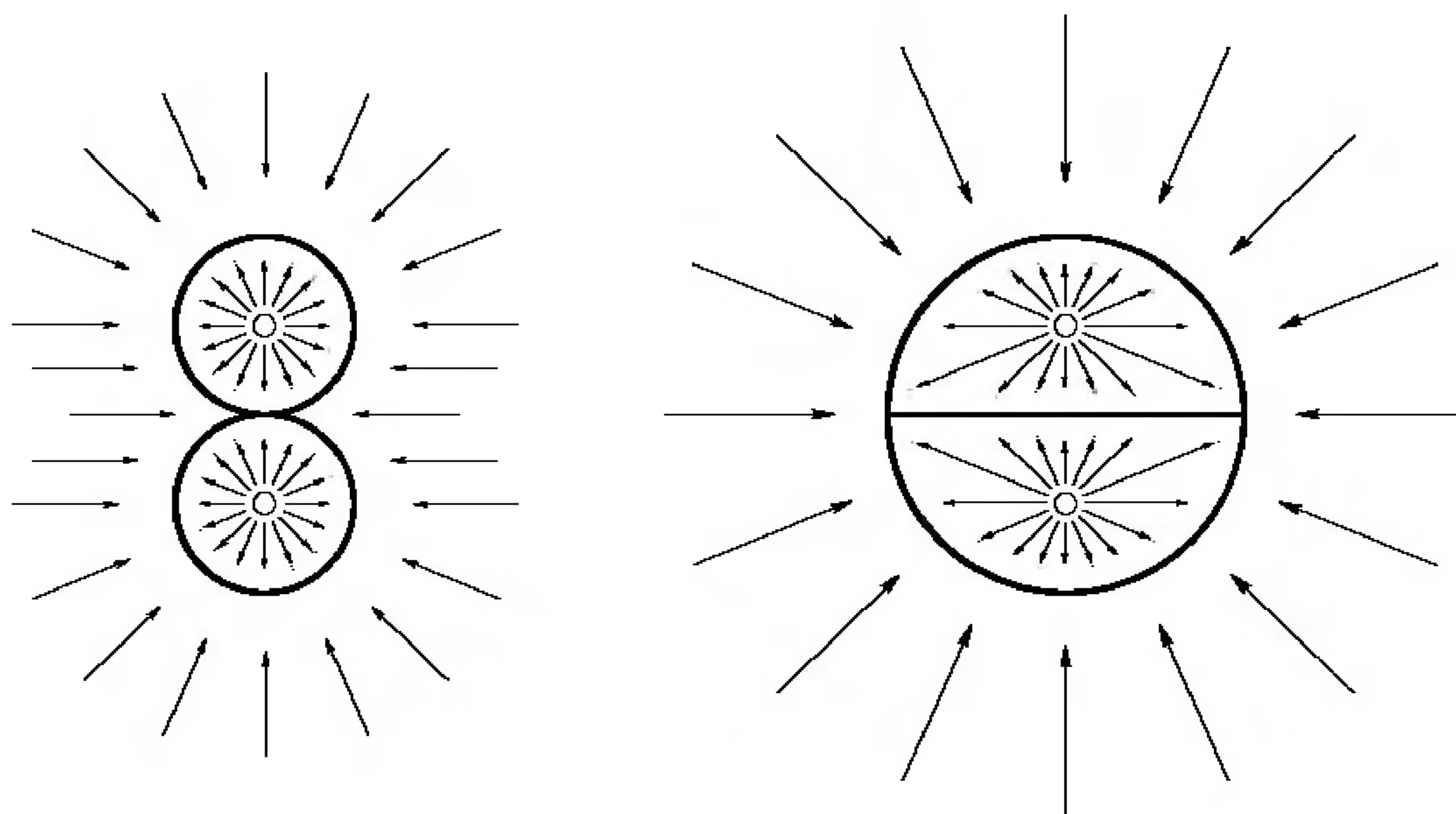
FIGURE 7.13. Deformation retractions onto \mathcal{E} and \Theta .
