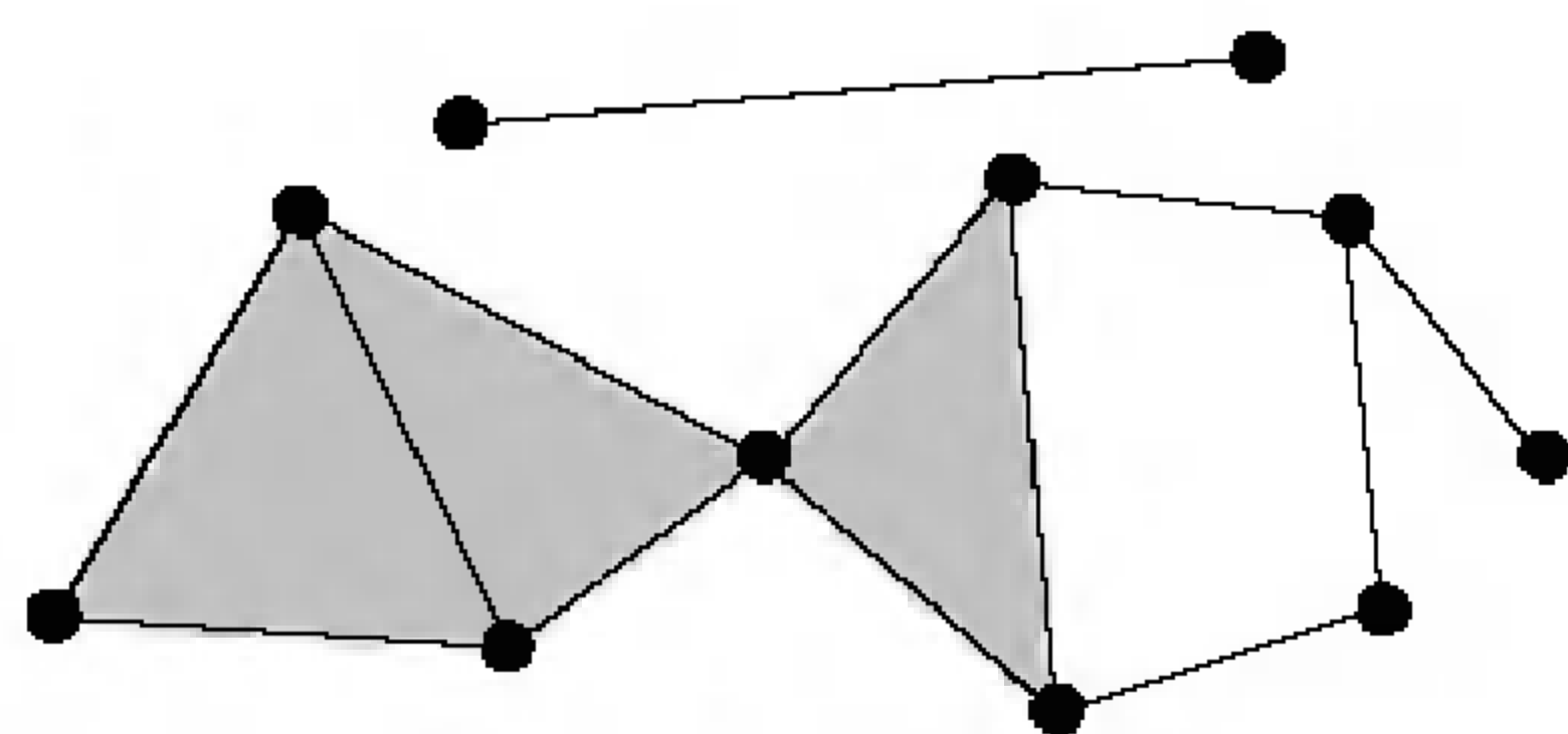
FIGURE 5.2. A complex in \mathbb{R}^2 .
