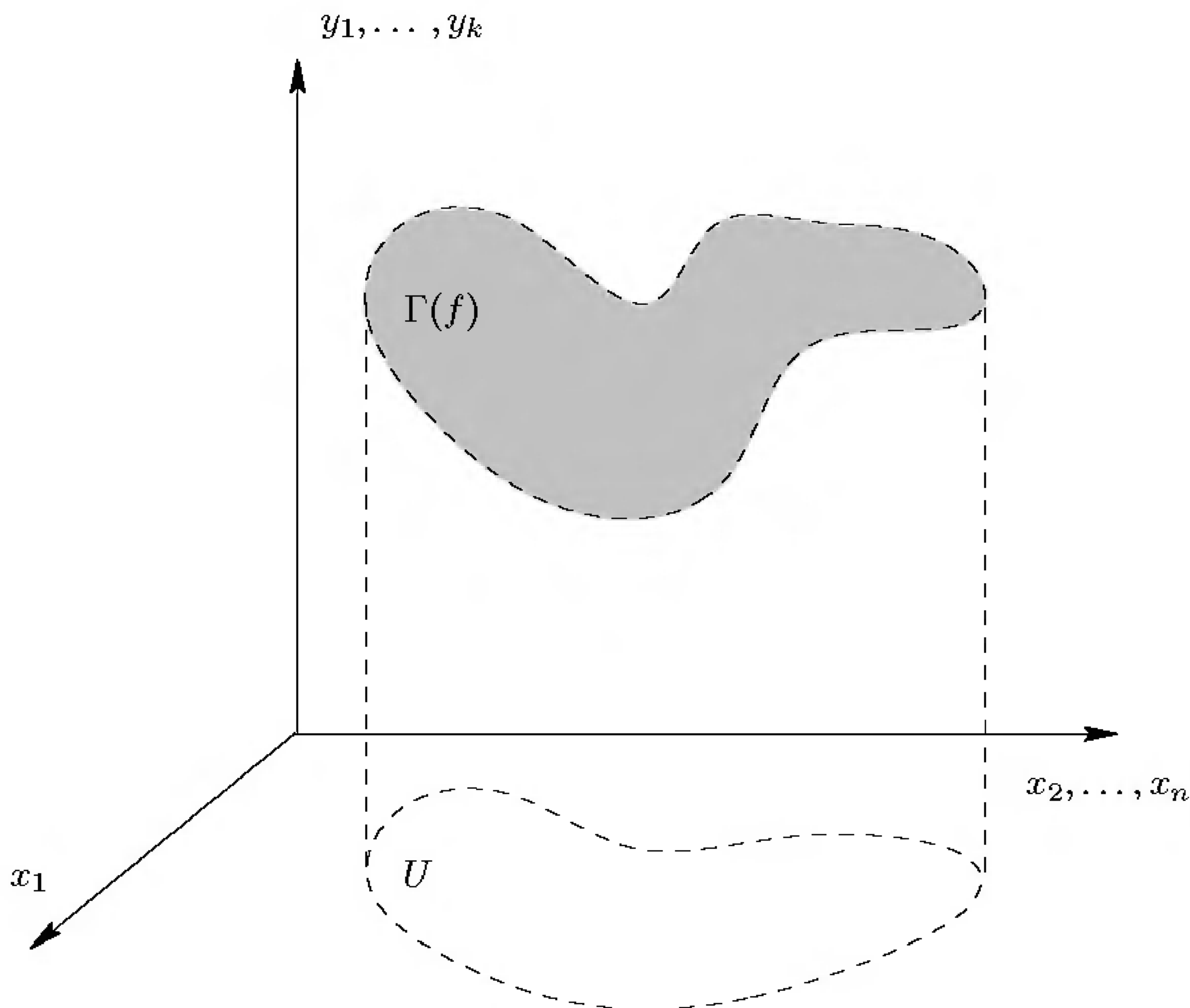
FIGURE 3.5. The graph of a continuous function.
