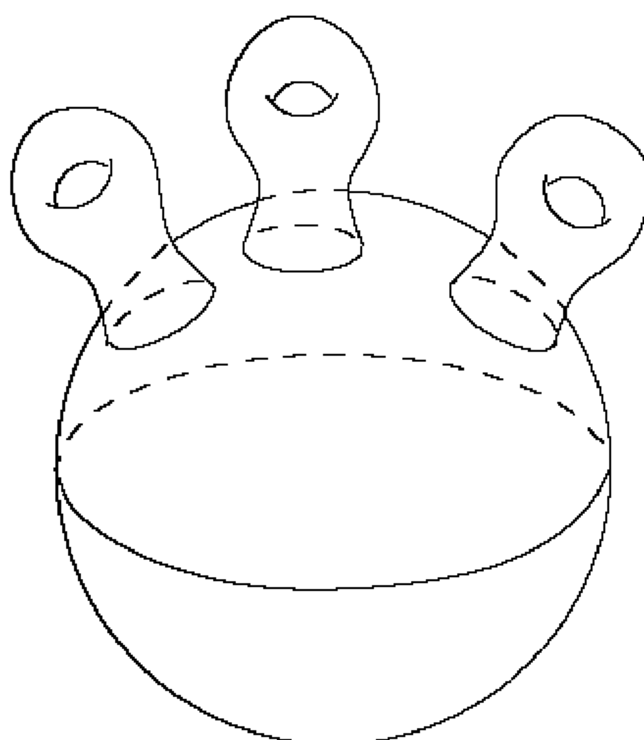
FIGURE 6.14. A sphere with handles.
