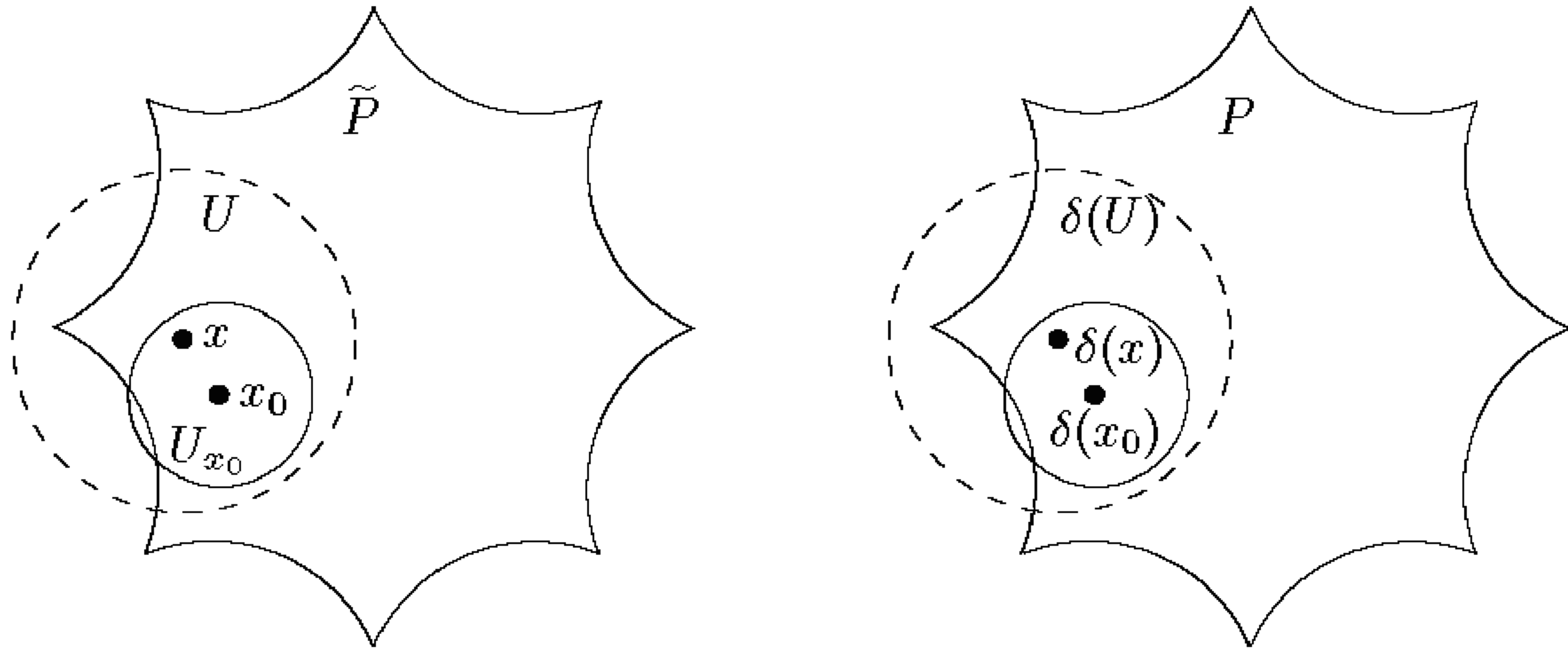
FIGURE 12.12. Finding regular hyperbolic balls of fixed radius.
