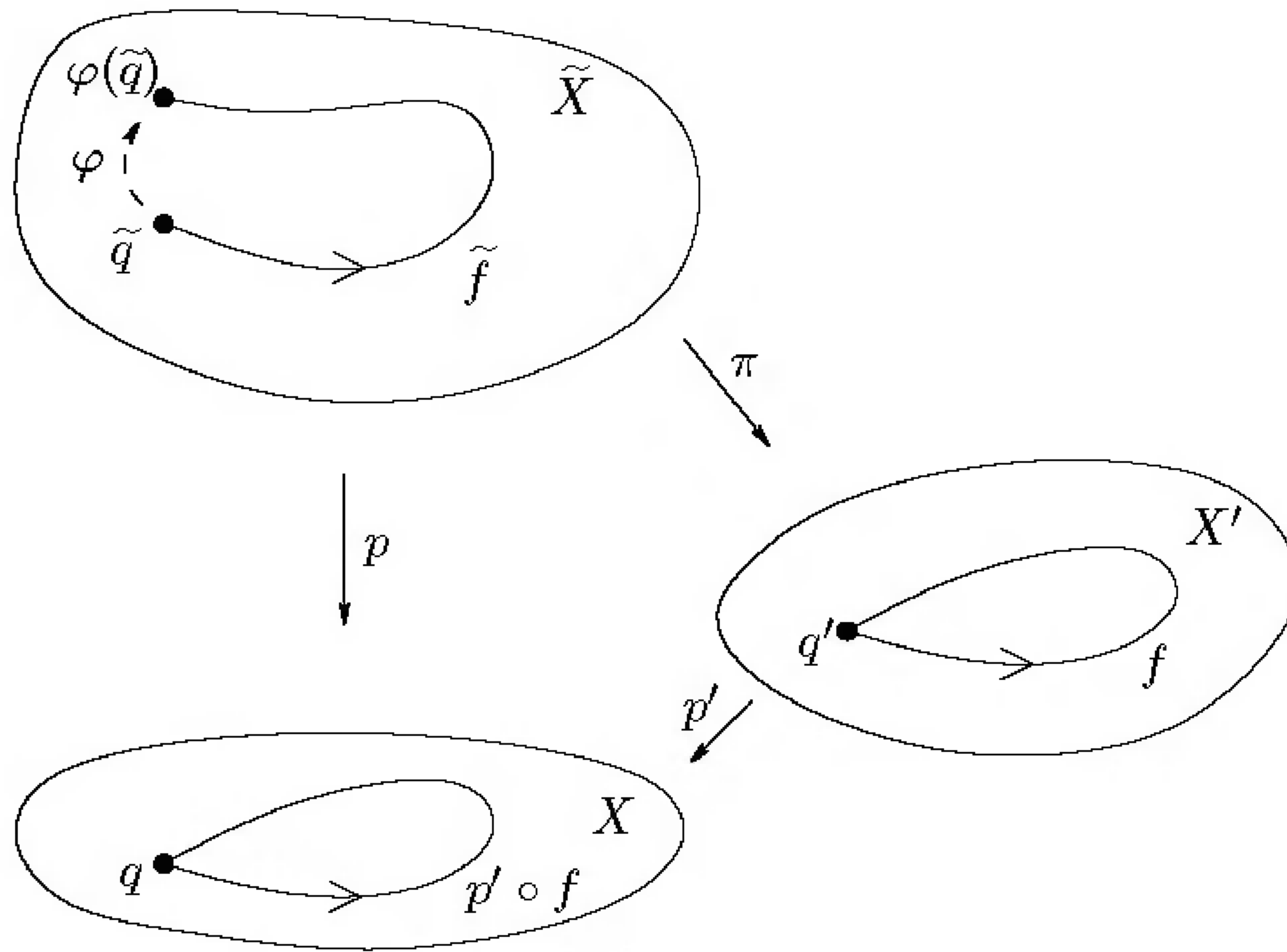
FIGURE 12.13. Proof of the classification theorem.
