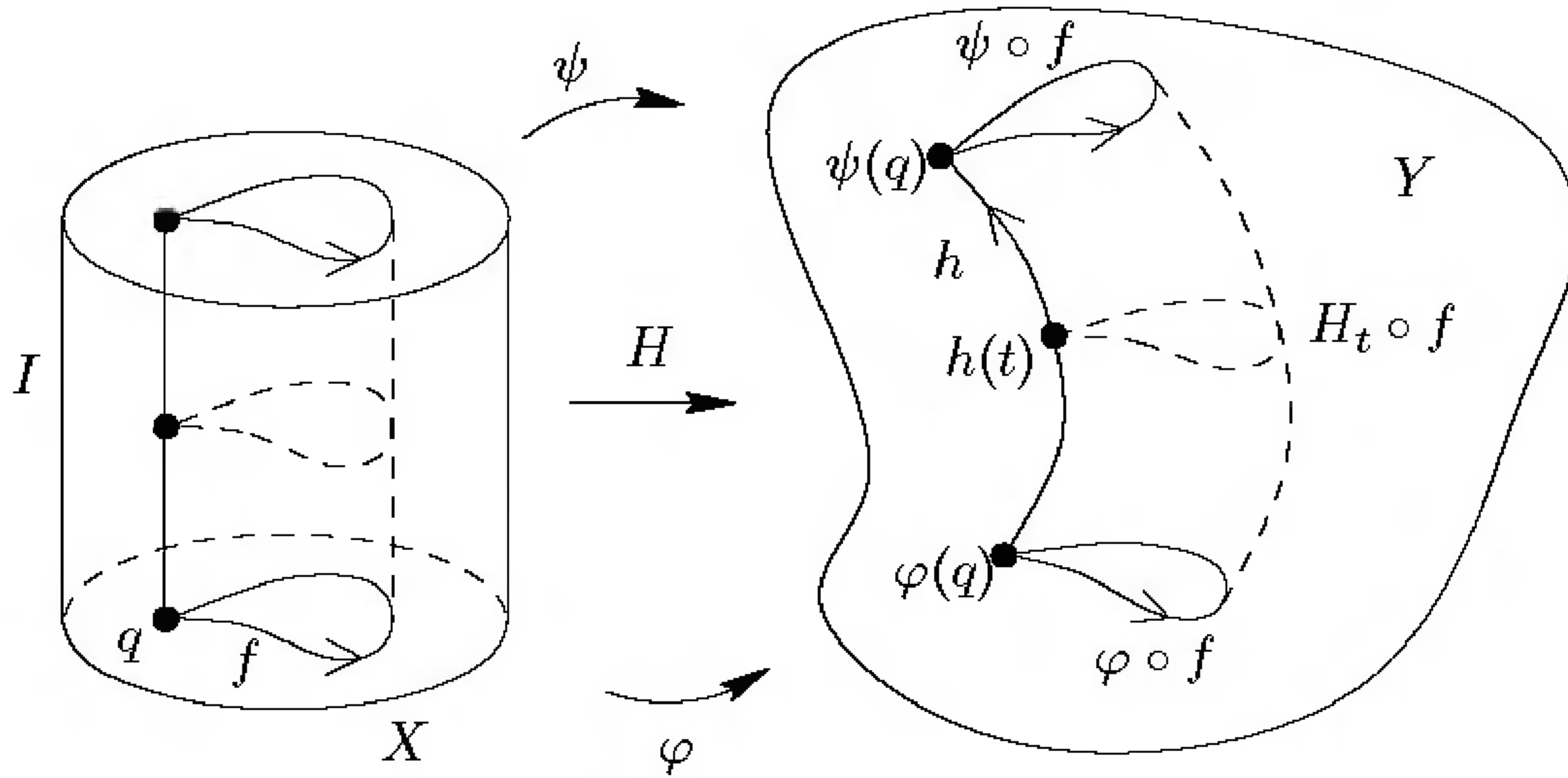
FIGURE 7.17. Induced homomorphisms of homotopic maps.
