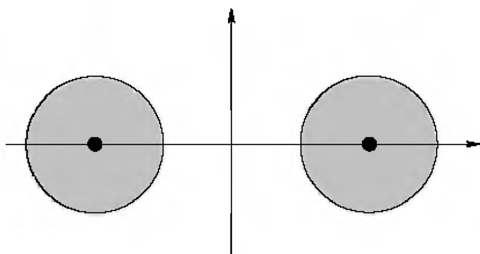
FIGURE 4.1. Union of two disks.
