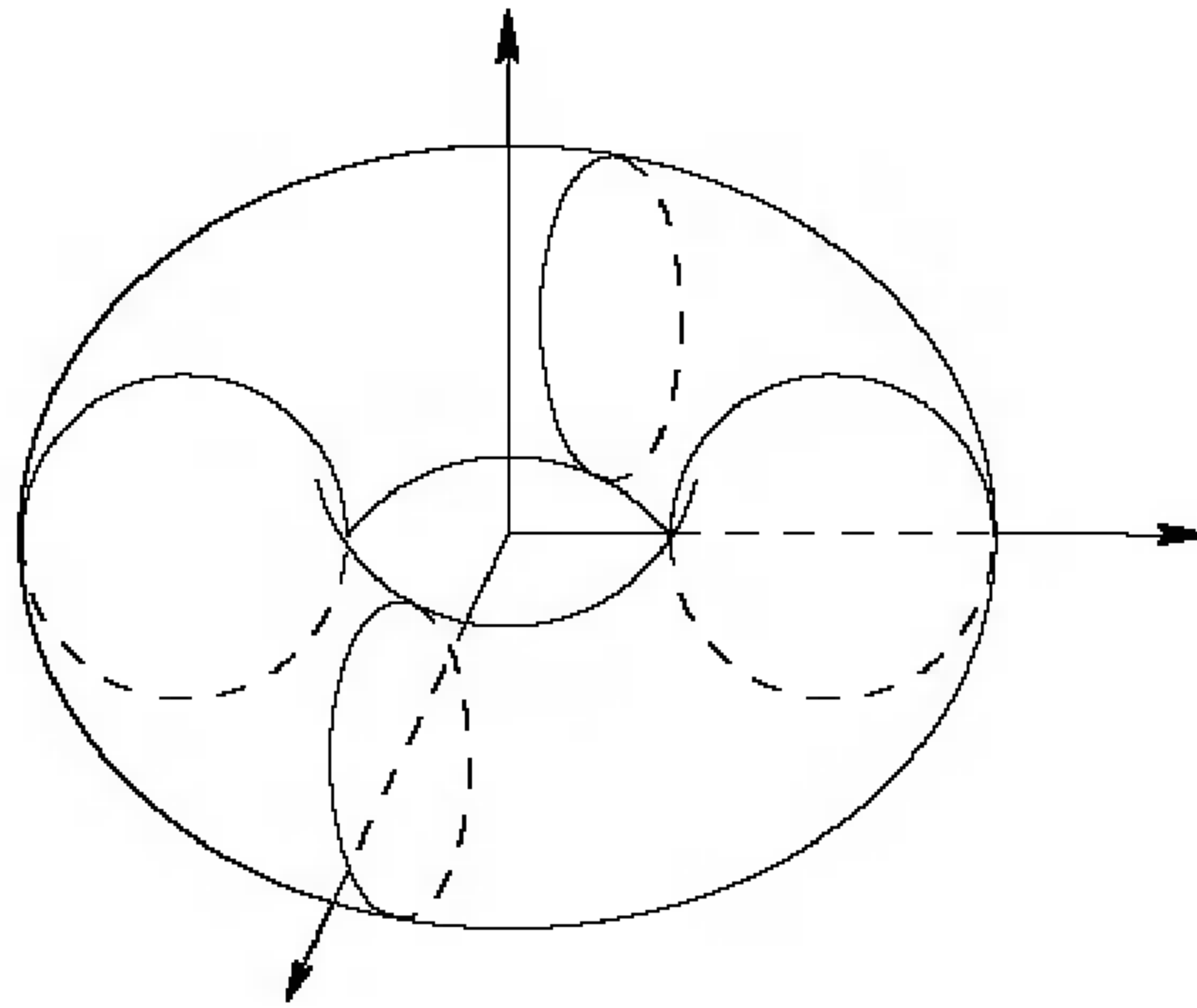
FIGURE 1.3. Doughnut surface.
