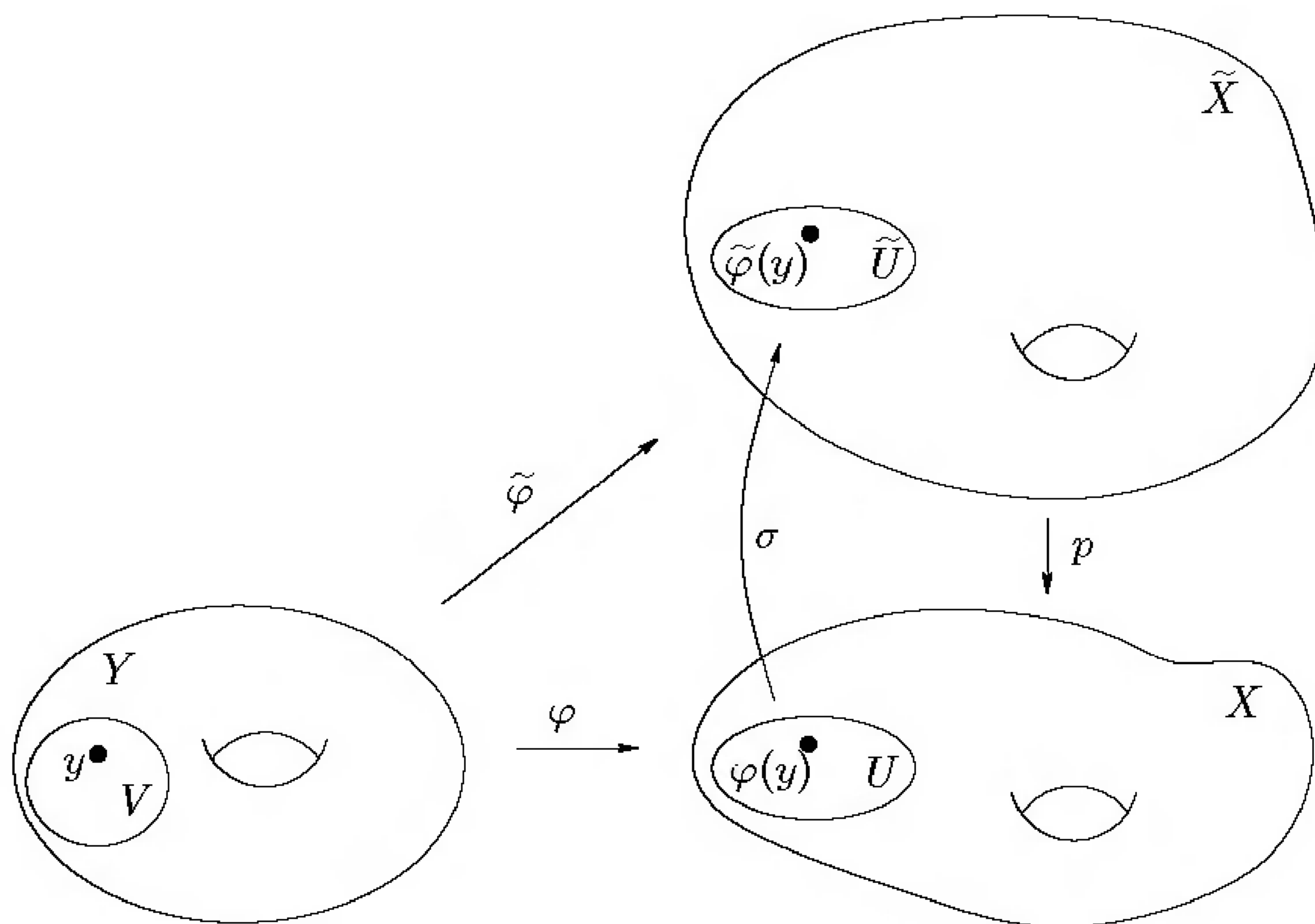
FIGURE 11.6. Proof that \tilde{\varphi} is continuous.
