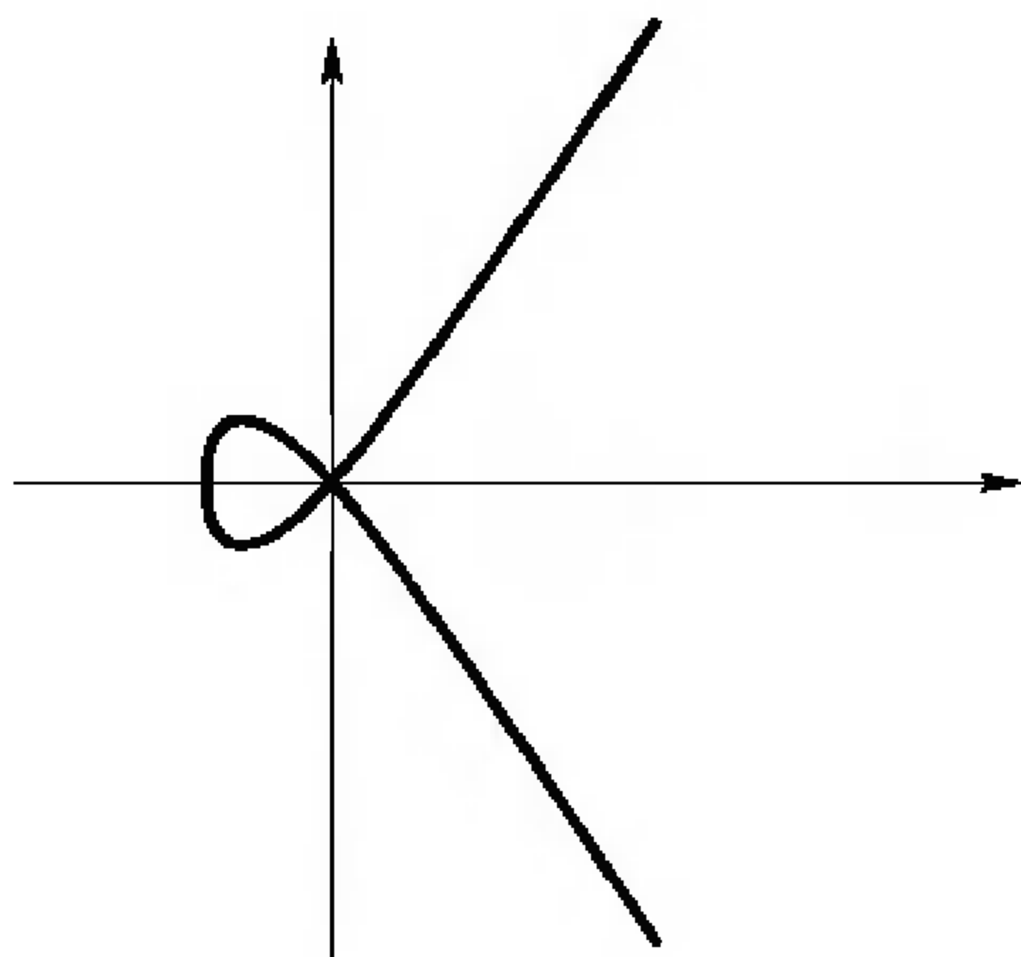
FIGURE 1.9. A self crossing.
