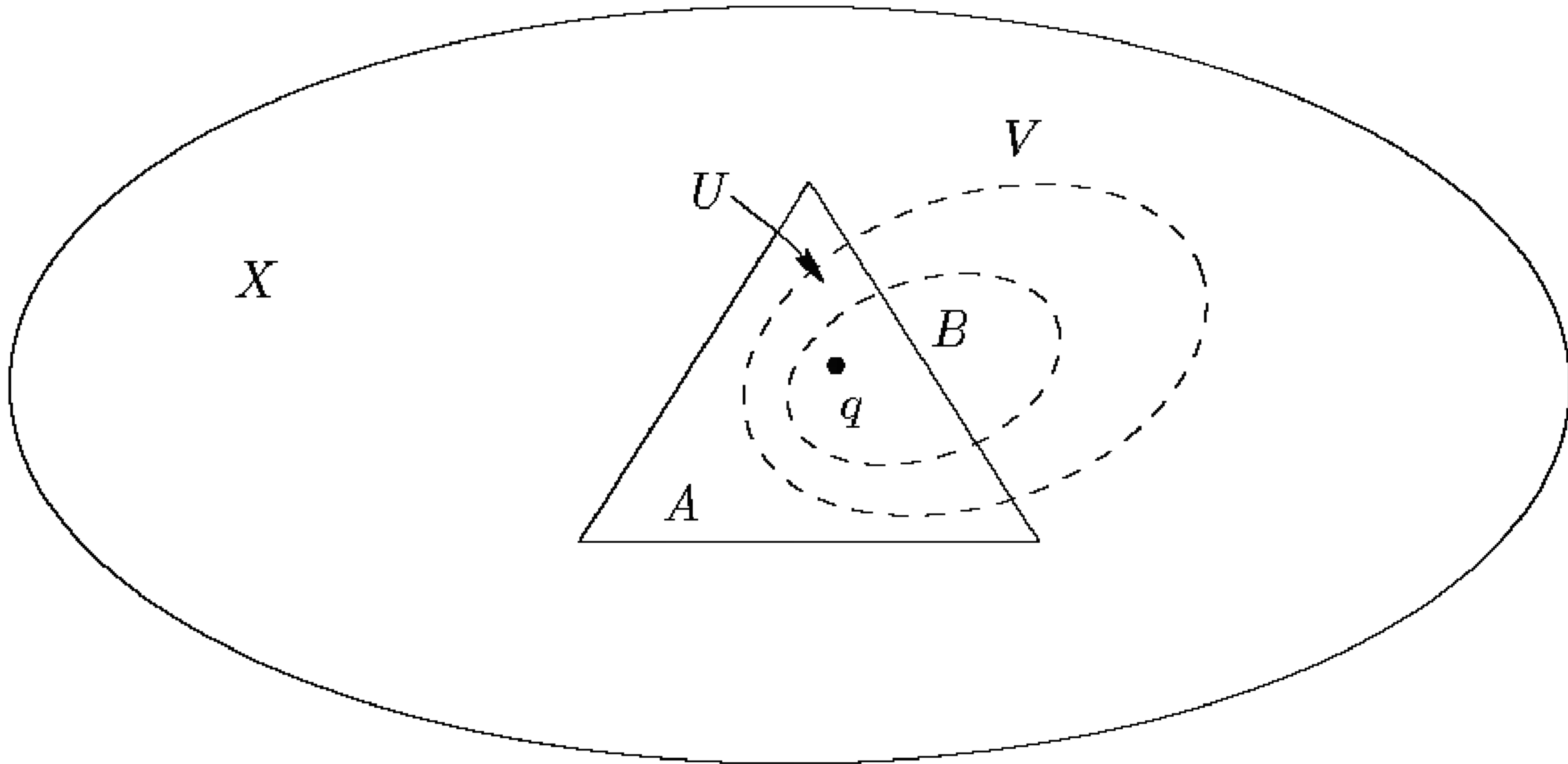
FIGURE 3.4. A basis open set for a subspace.
