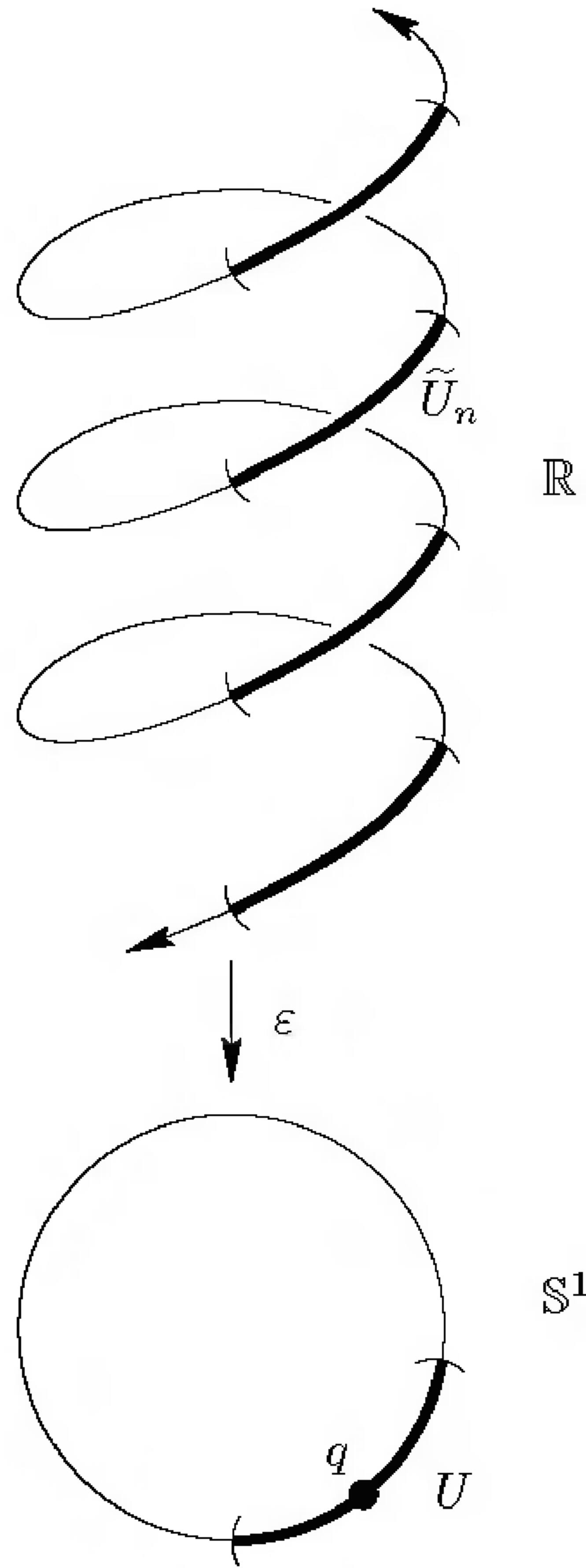
FIGURE 8.2. Evenly covered neighborhood in S^1 .
