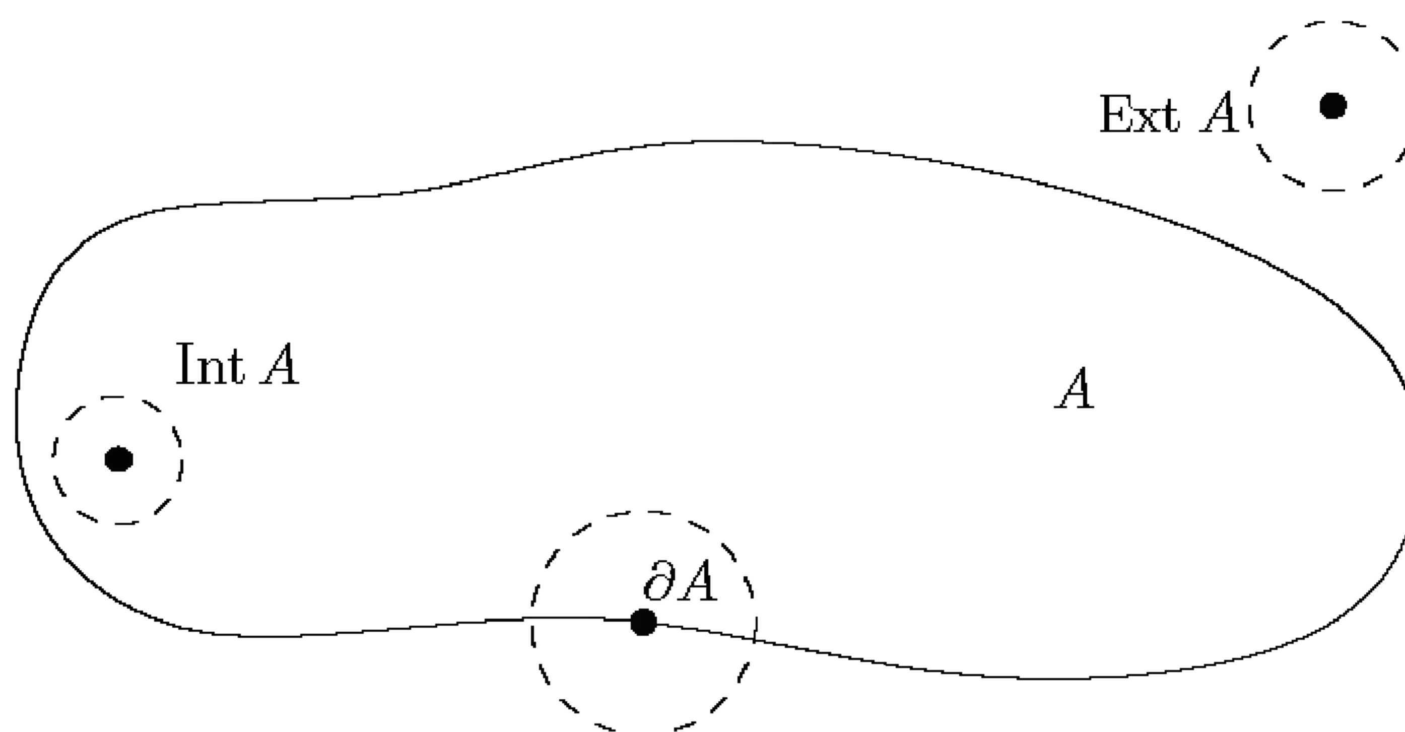
FIGURE 2.5. Interior, exterior, and boundary points.
