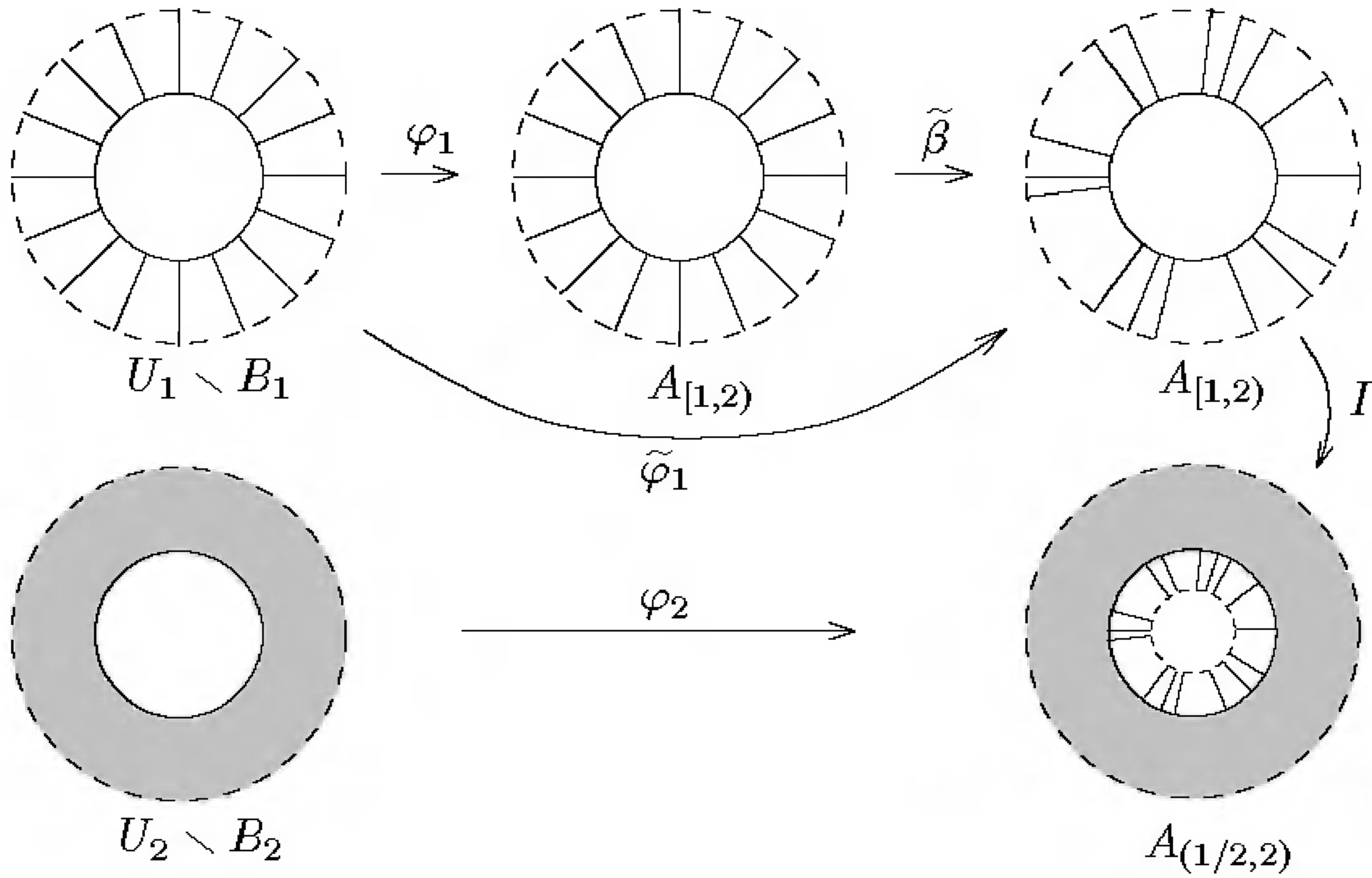
FIGURE 6.11. Euclidean neighborhood of points in S .
