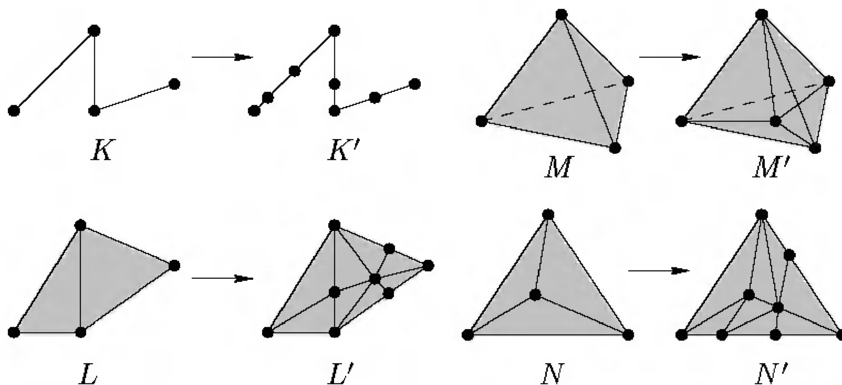
FIGURE 5.11. Subdivisions.
