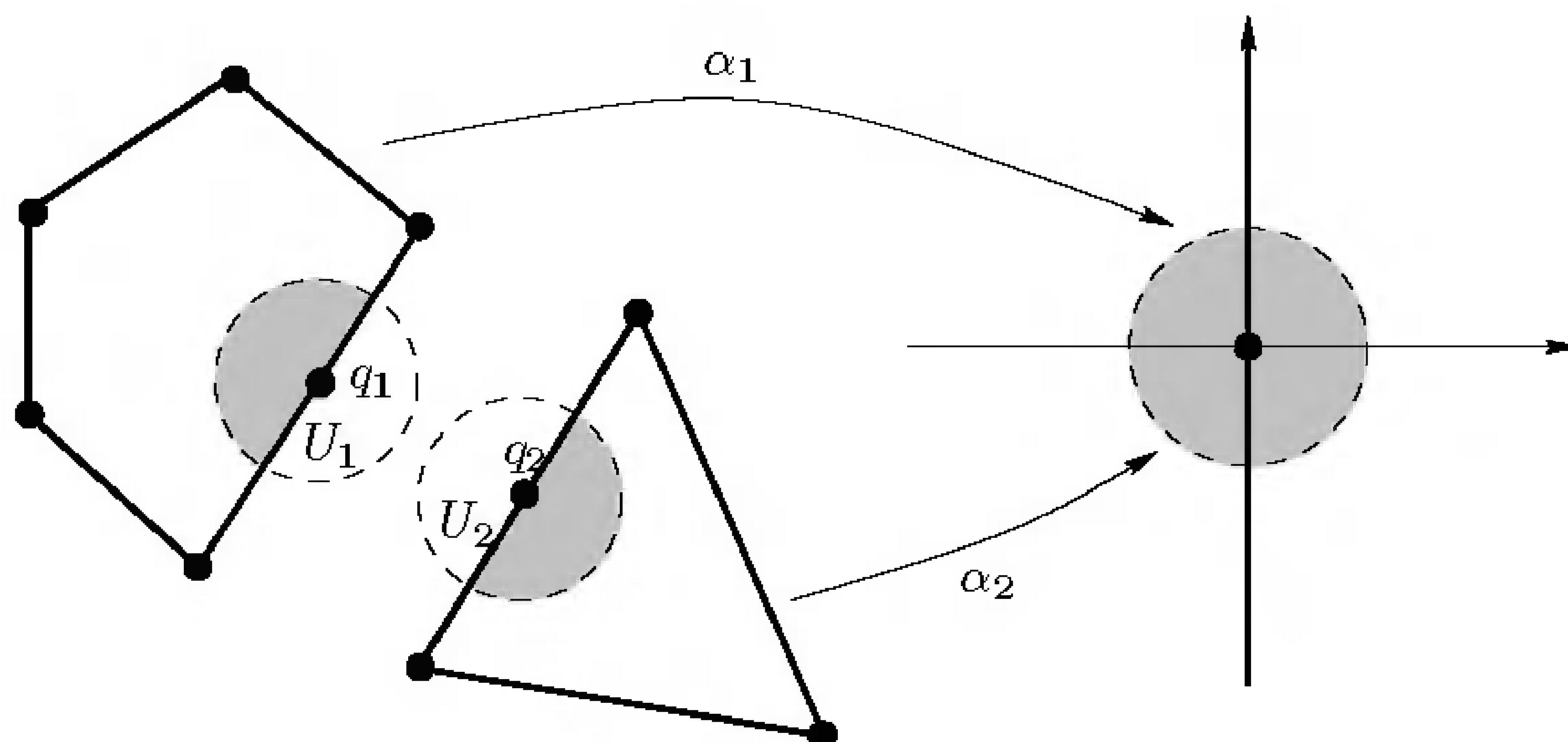
FIGURE 6.7. Euclidean neighborhood of an edge point.
