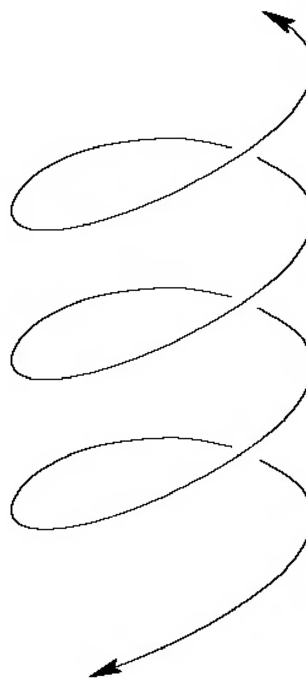
FIGURE 1.2. Space curve.
