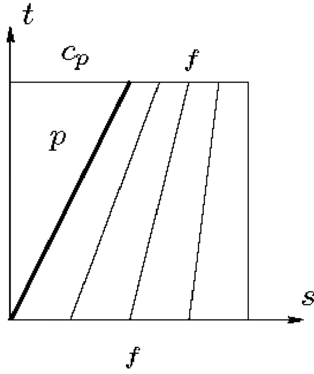
FIGURE 7.4. f \sim c_p \cdot f .
