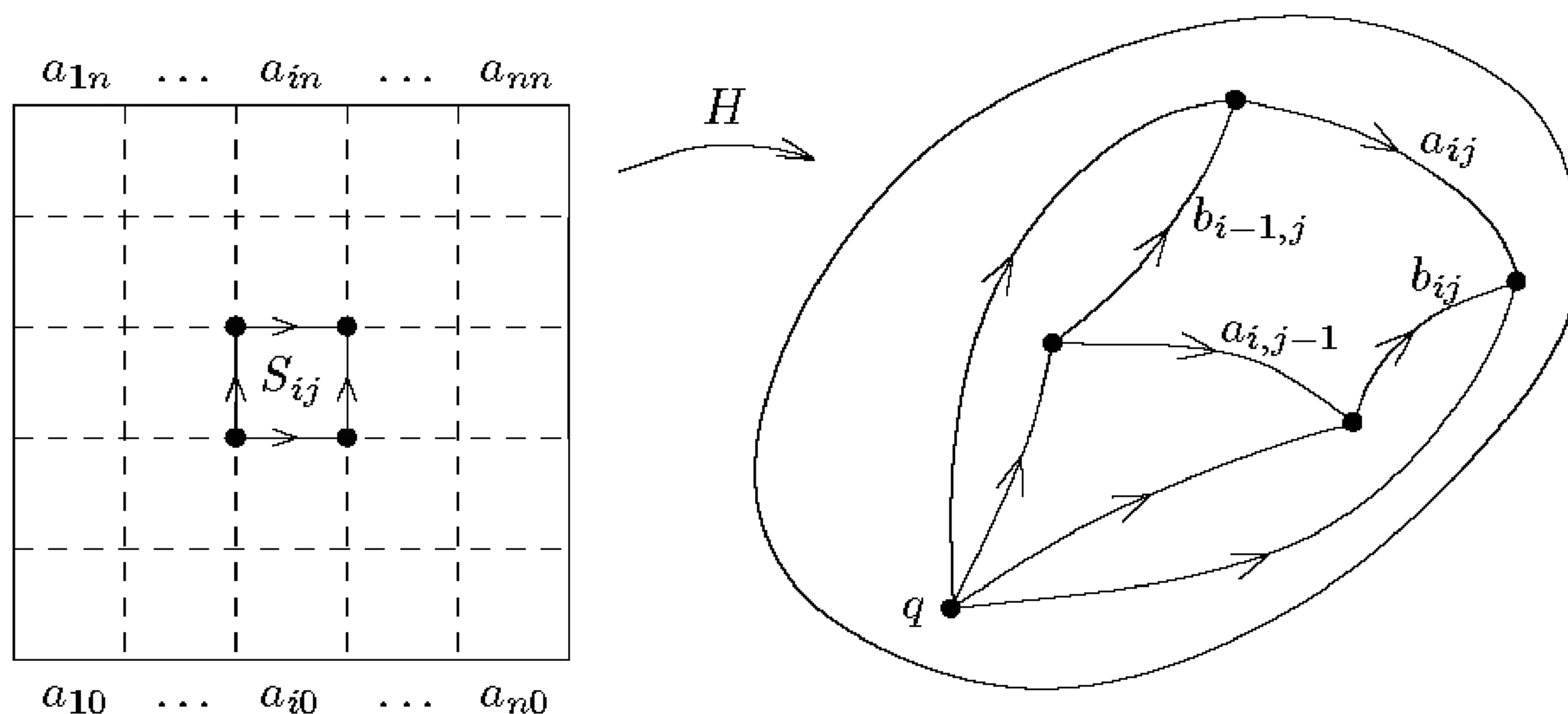
FIGURE 10.6. Proof that \text{Ker } \Phi \subset N .
