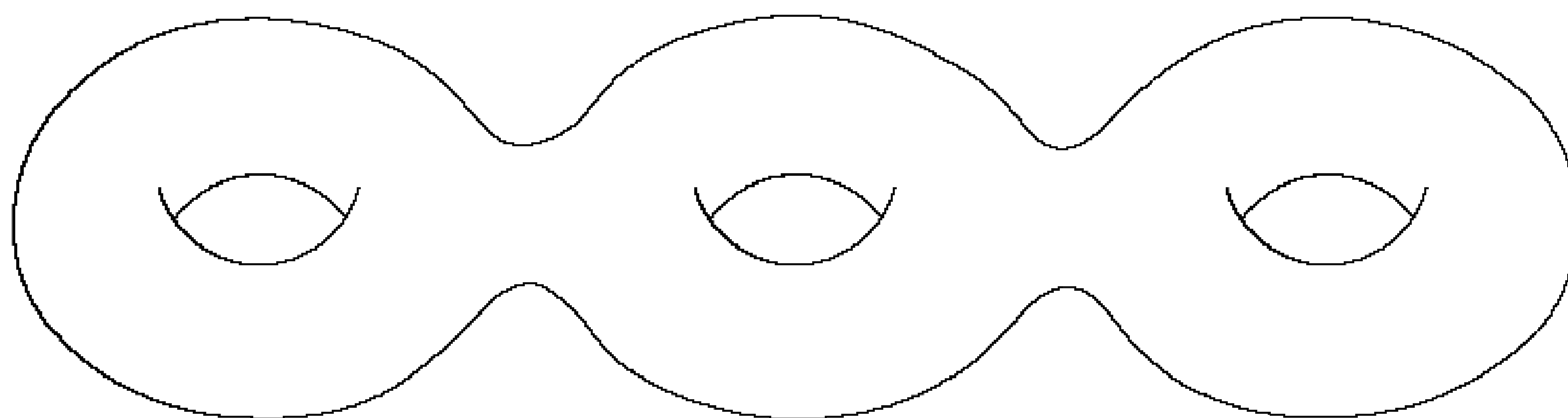
FIGURE 6.13. A connected sum of tori.
