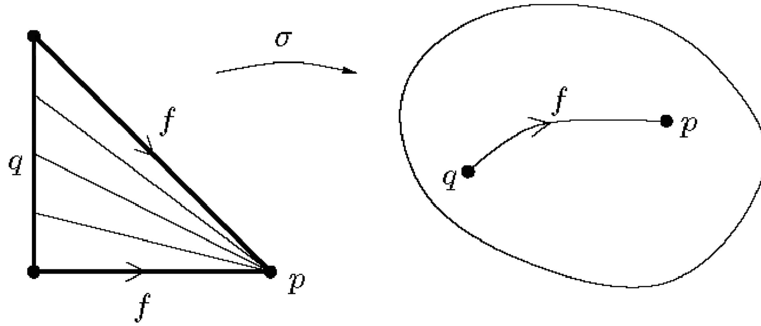
FIGURE 13.6. Proof that [f^{-1}]_H = -[f]_H .
