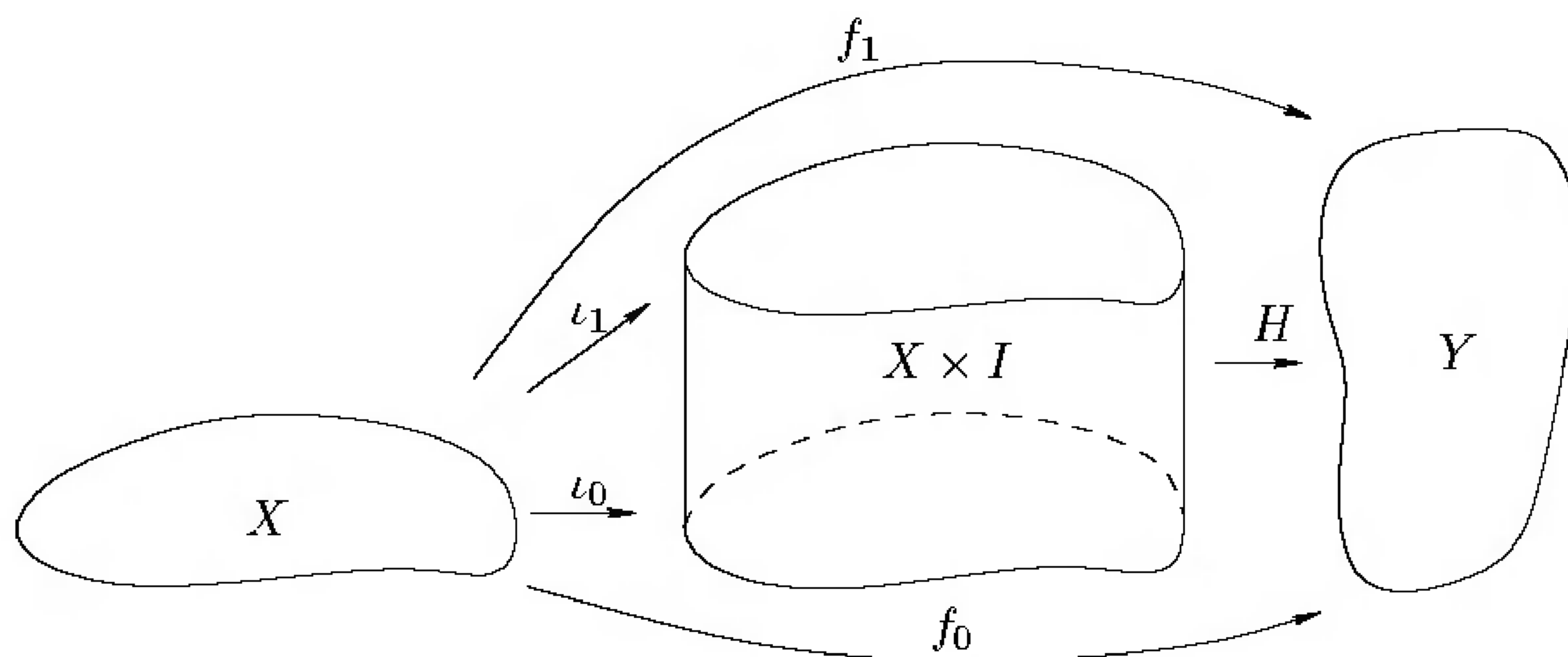
FIGURE 13.3. The setup for Theorem 13.7.
