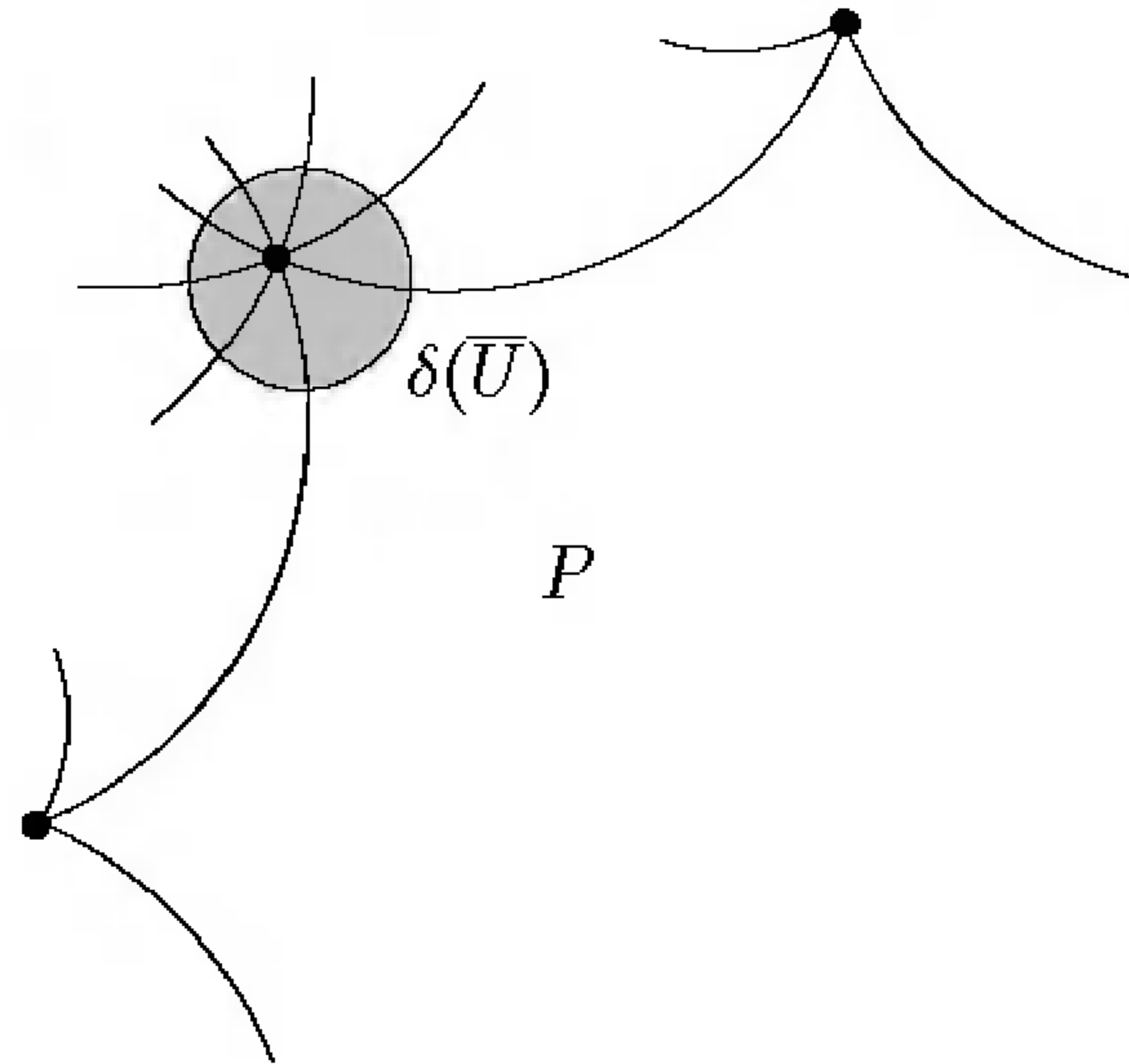
FIGURE 12.11. Hyperbolic neighborhood of a vertex point.
