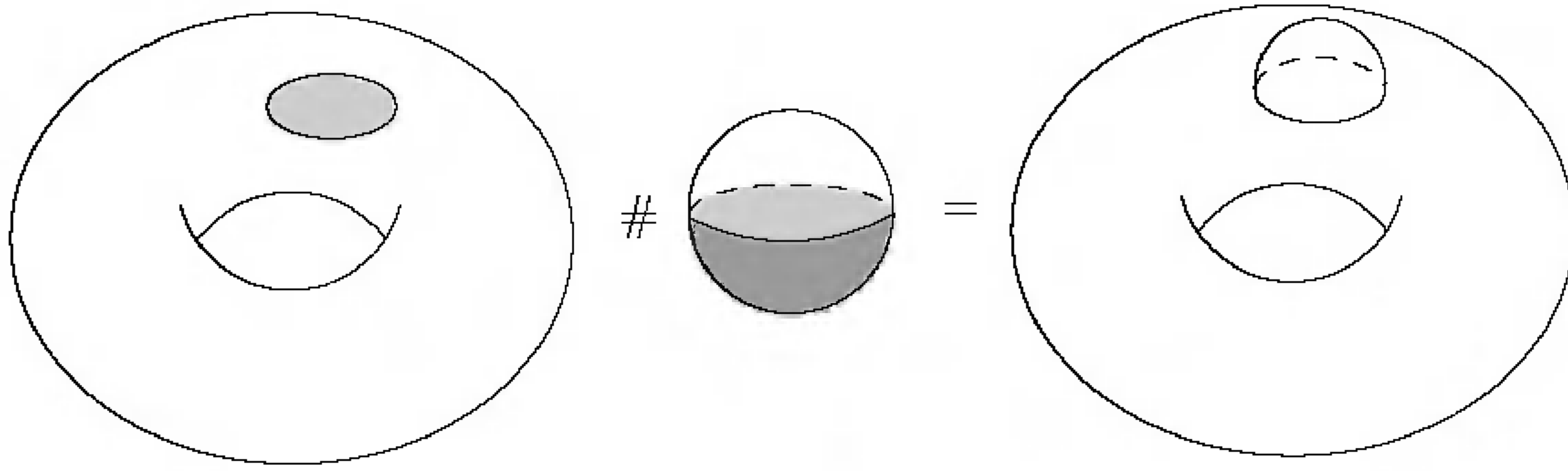
FIGURE 6.12. Connected sum with a sphere.
