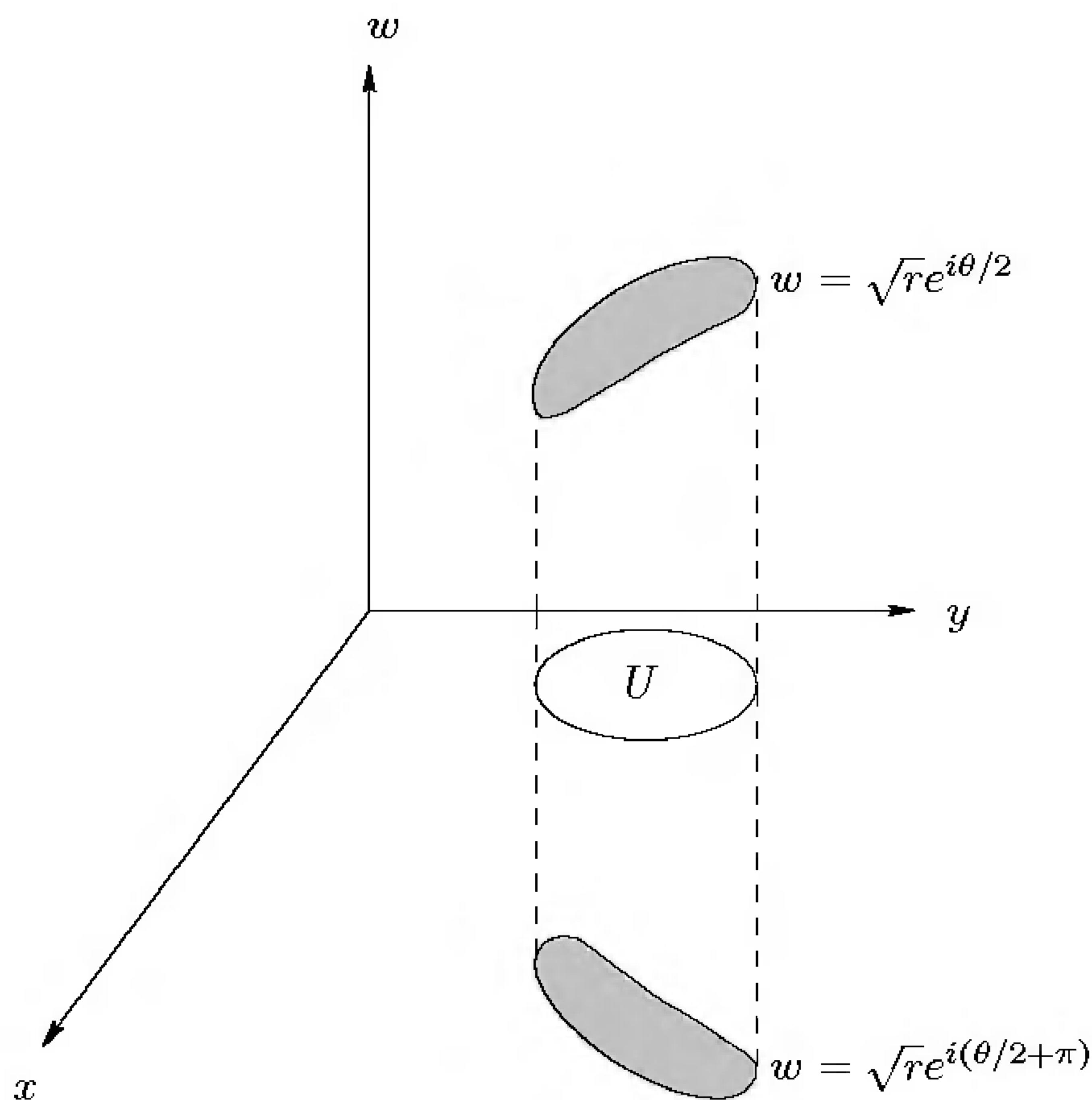
FIGURE 1.7. Two branches of the complex square root.
