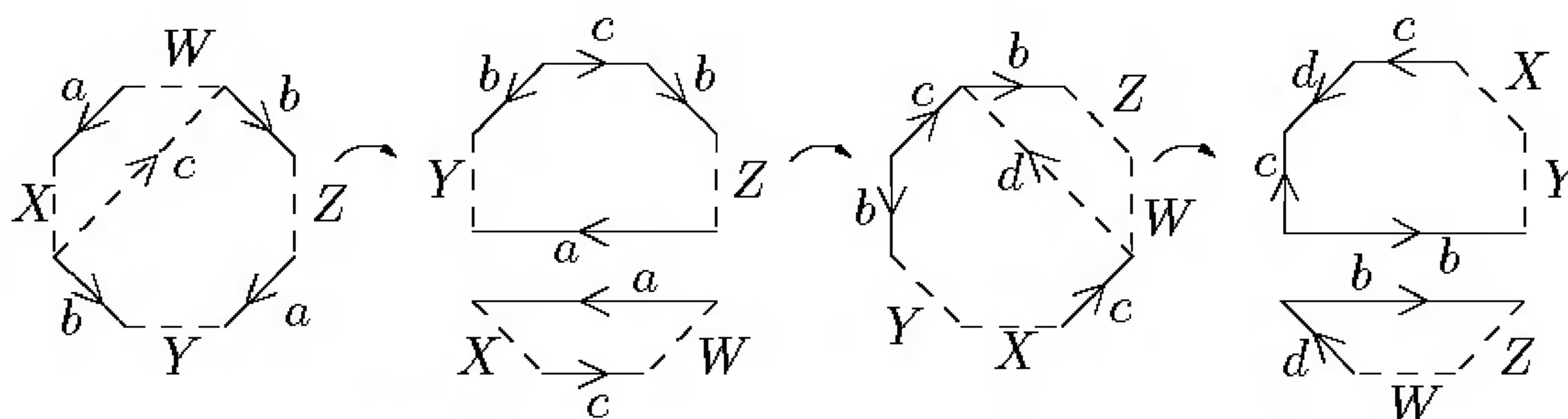
FIGURE 6.28. Bringing intertwined complementary pairs together.
