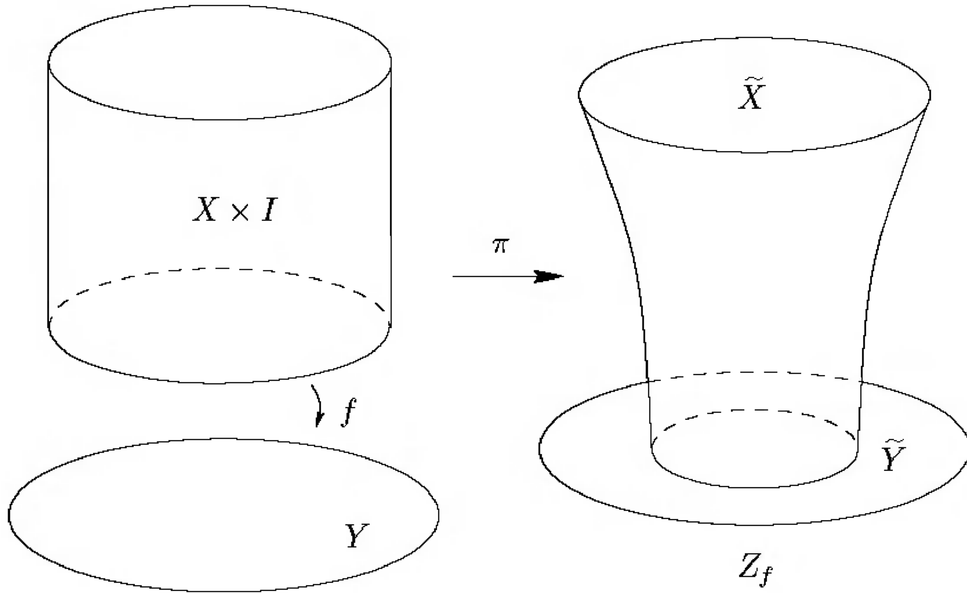
FIGURE 7.18. The mapping cylinder.
