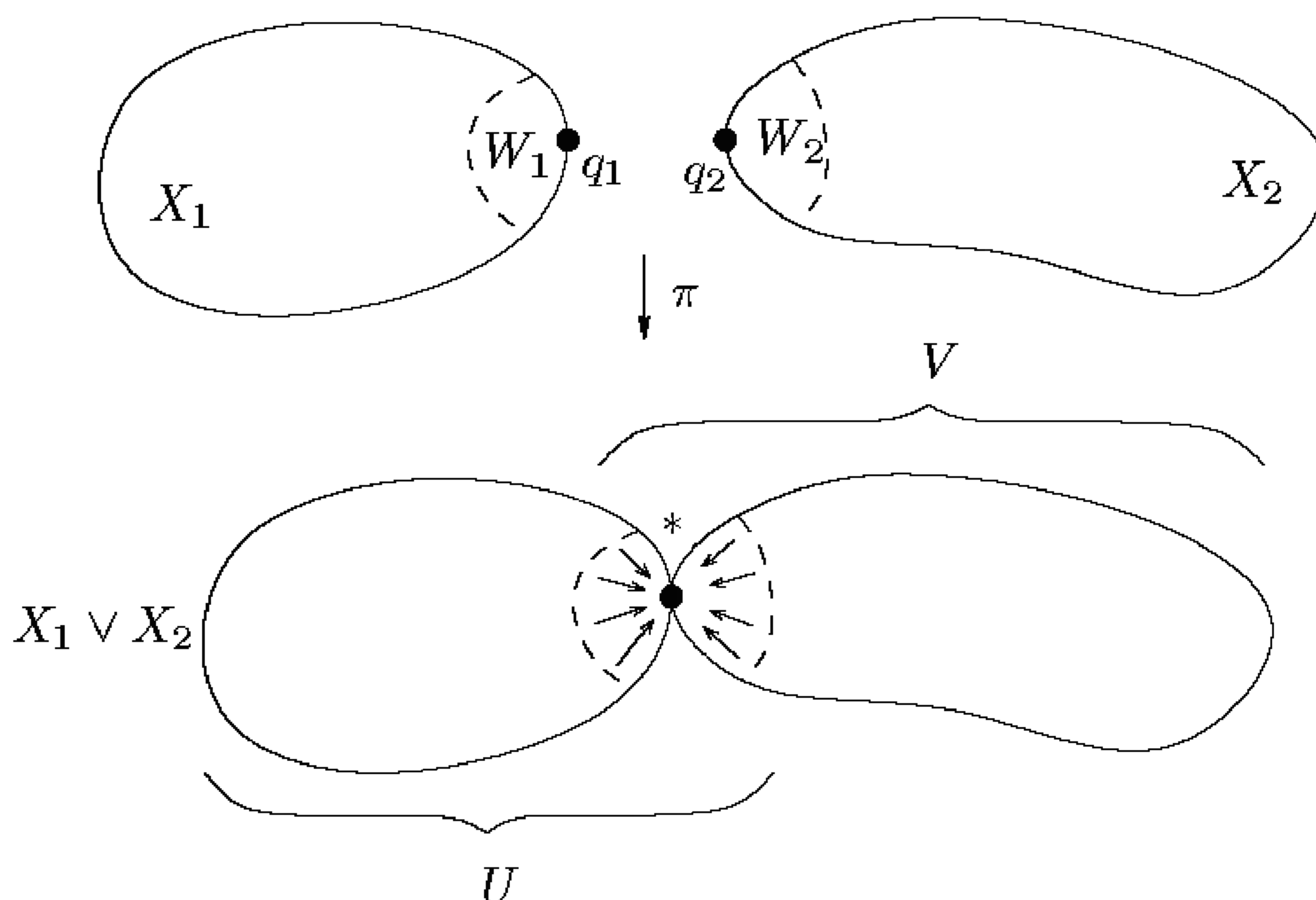
FIGURE 10.1. Computing the fundamental group of a wedge.
