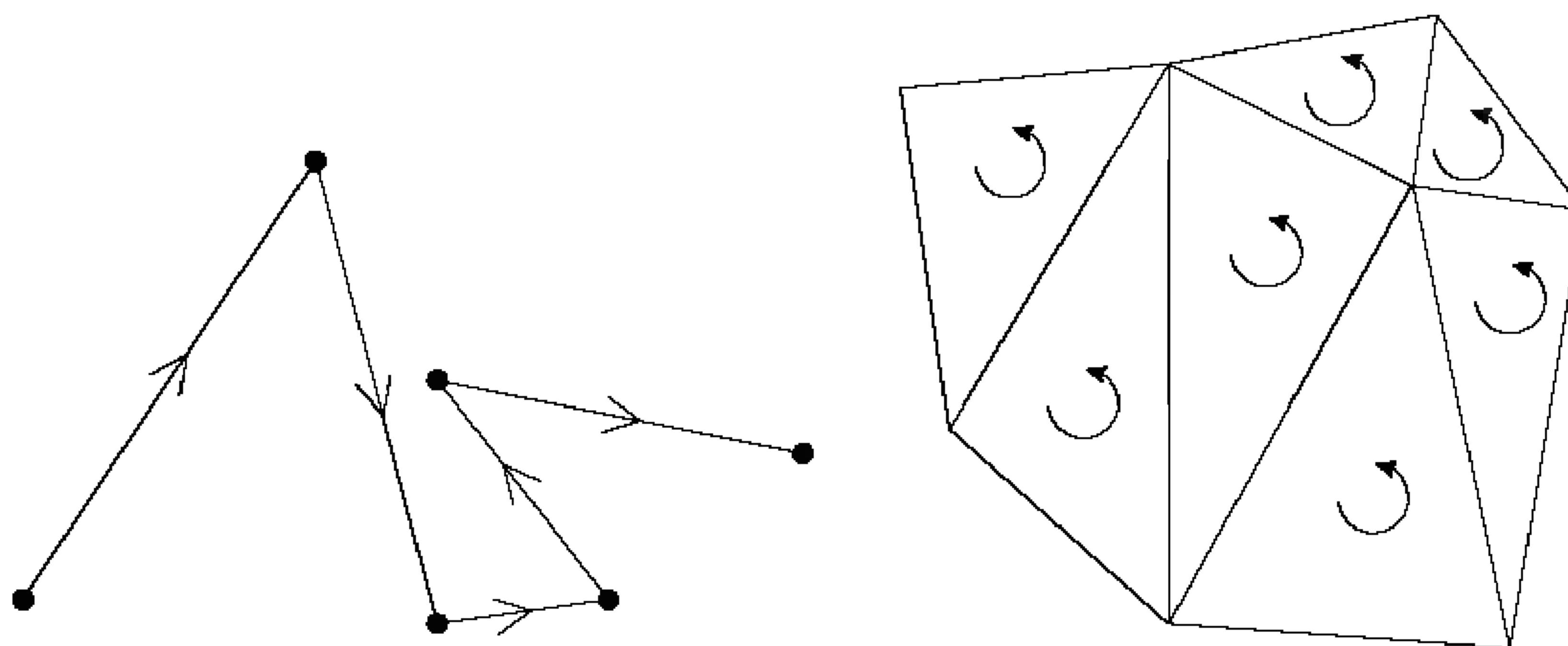
FIGURE 5.10. Orientations of simplicial complexes.
