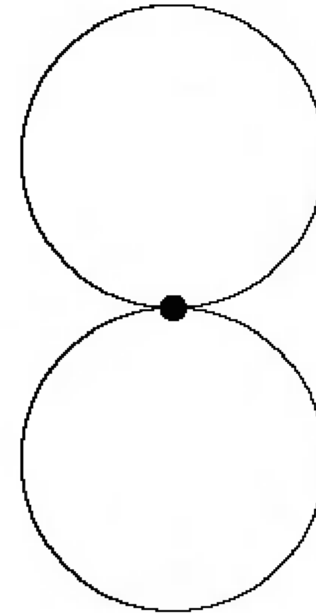
FIGURE 3.11. Wedge of two circles.
