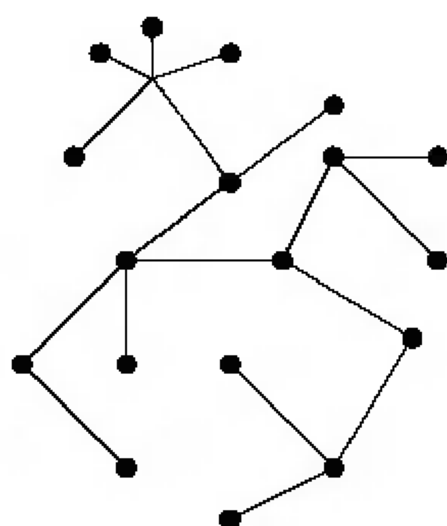
FIGURE 7.14. A tree.
