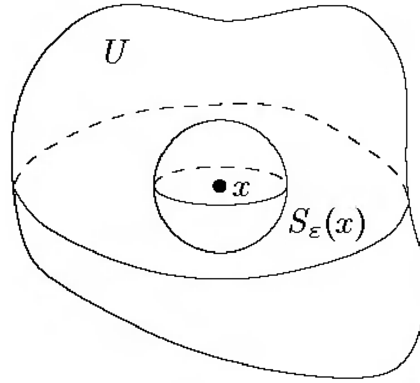
FIGURE 13.10. Proof of Lemma 13.21.
