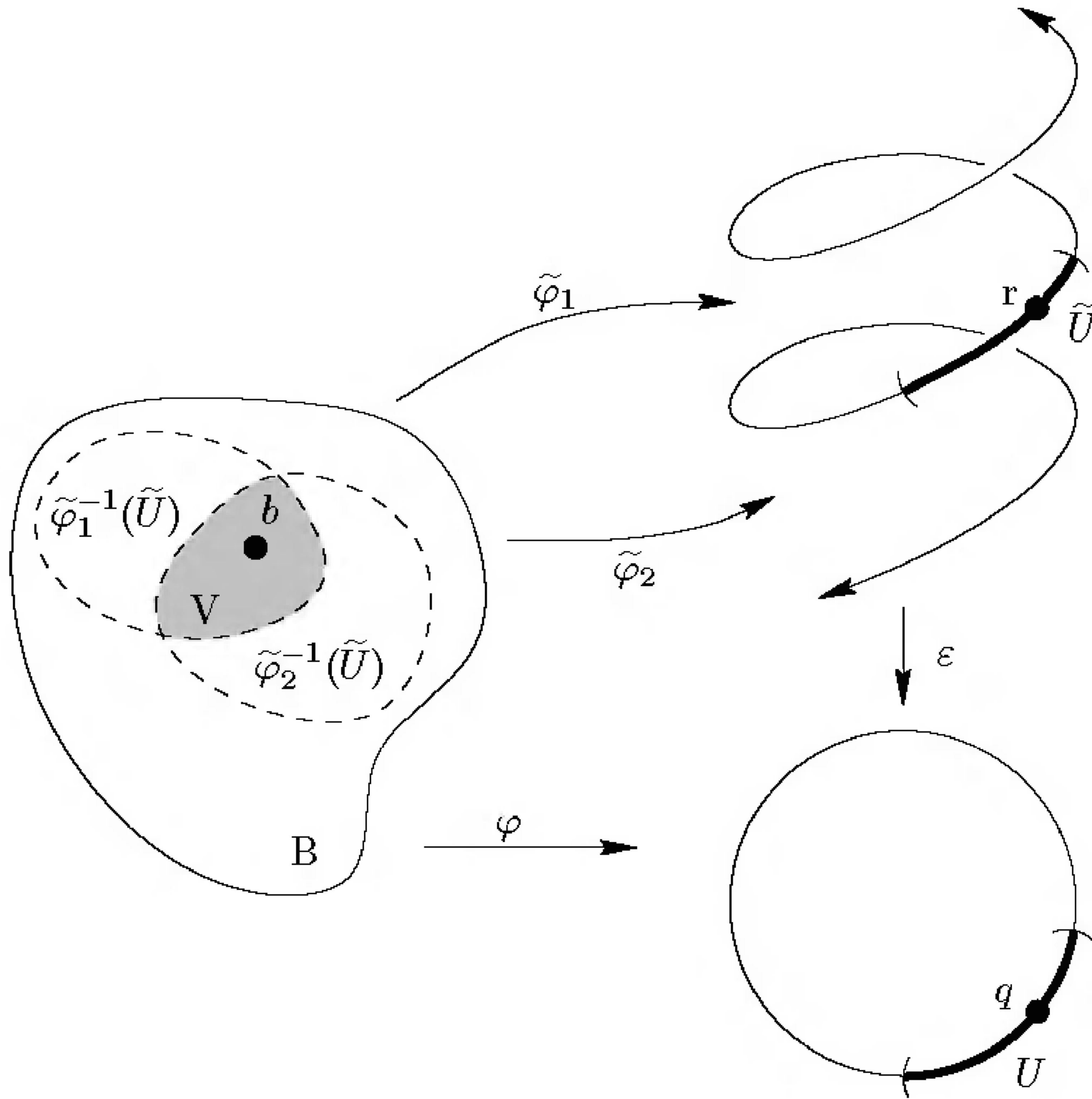
FIGURE 8.3. Proof of the unique lifting property.
