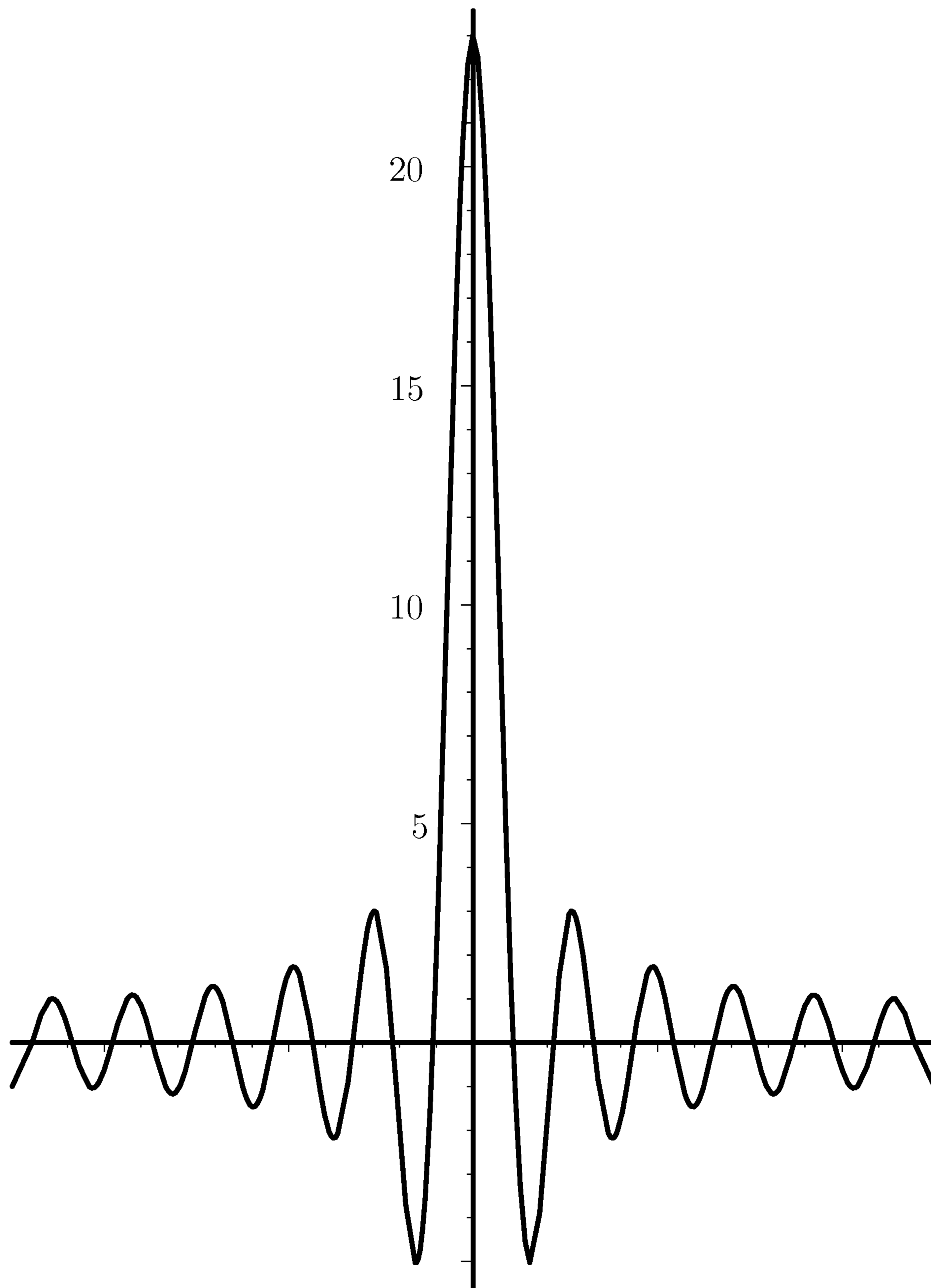
Figure 9.2. The Dirichlet kernel D_{11}(x) for -\frac{1}{2} \leq x \leq \frac{1}{2} .
