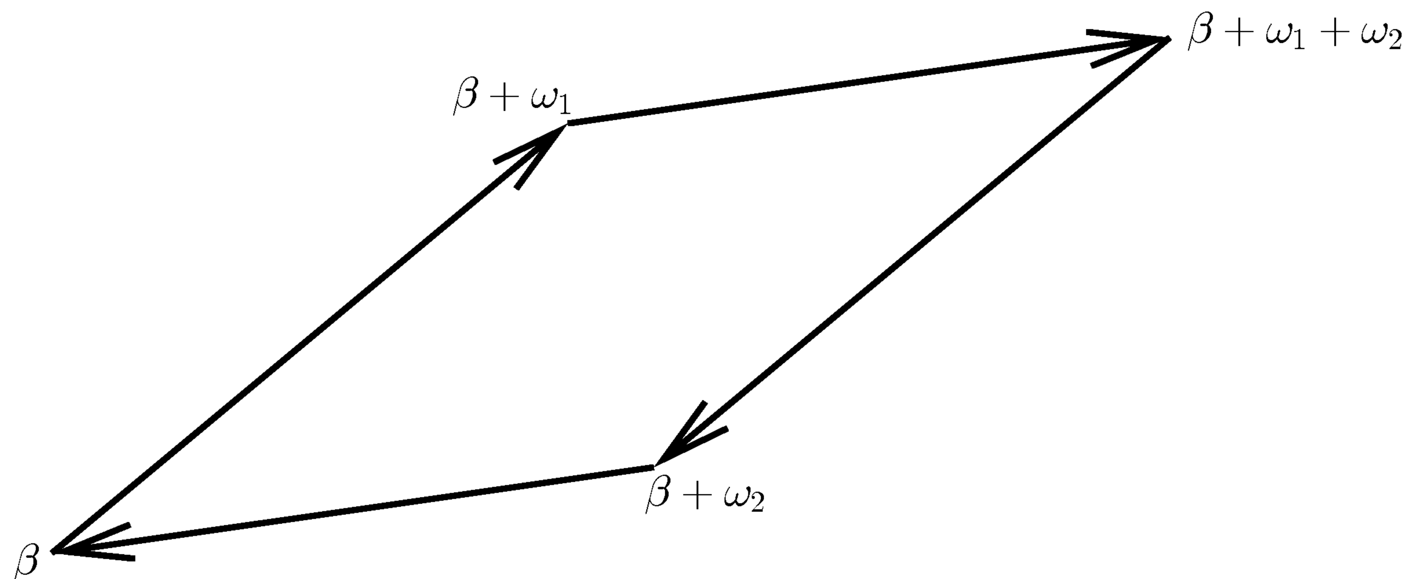
Figure 6.3. Integrating along the four sides of \Gamma_\beta .
