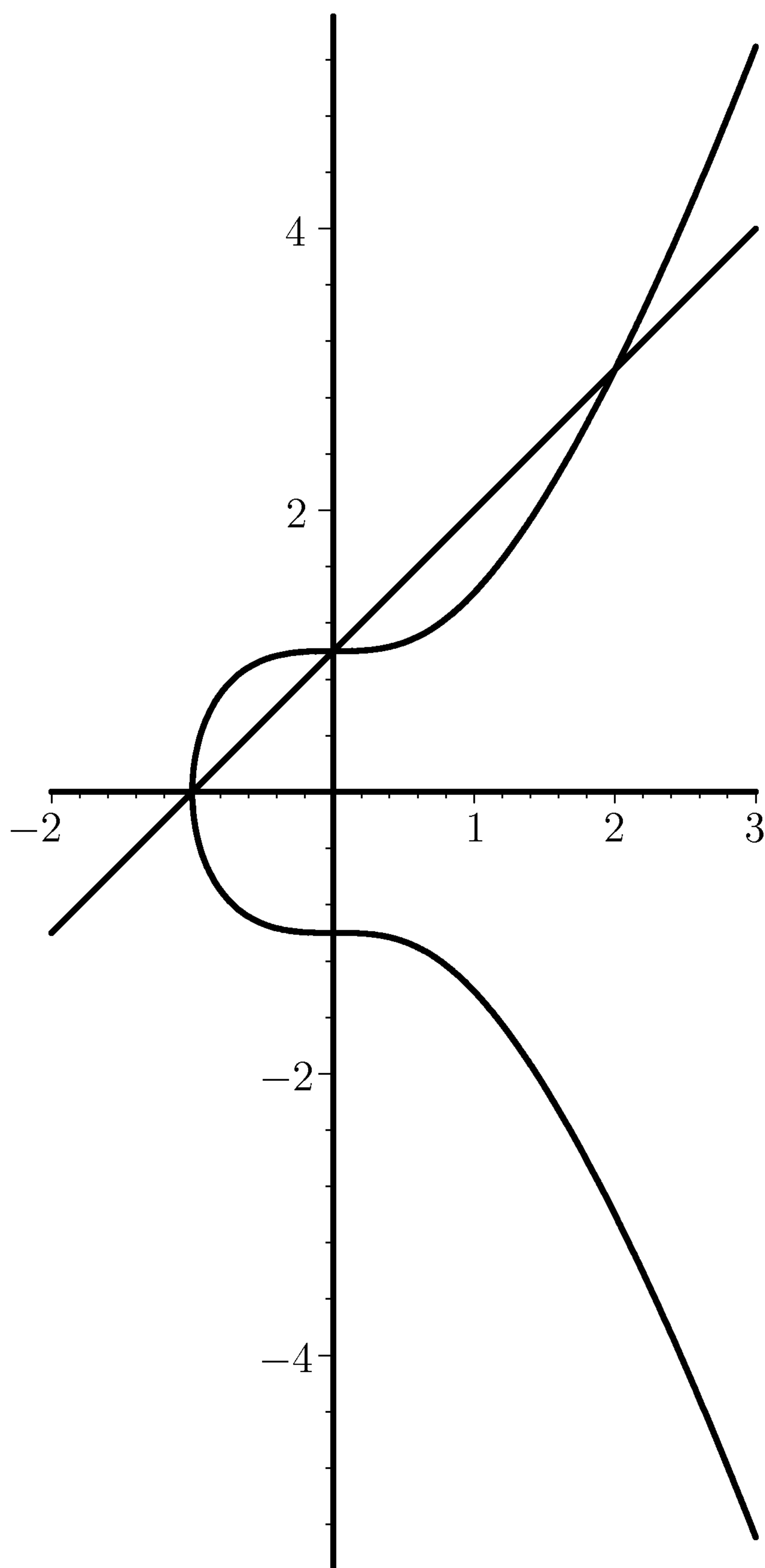
Figure 5.1. The binary operation on y^2 = x^3 + 1 , showing (2, 3) + (0, 1) + (-1, 0) = 0 .
