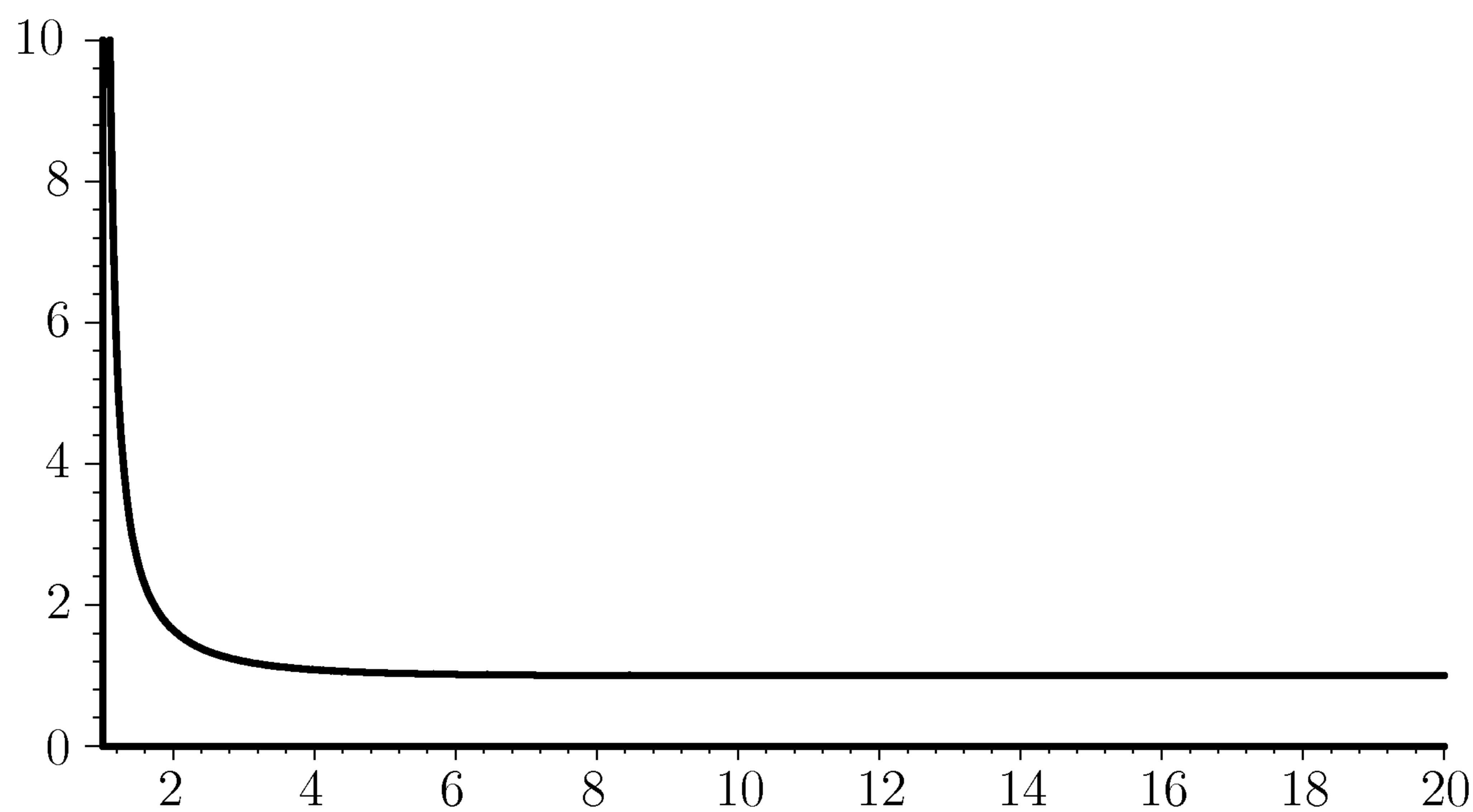
Figure 1.2. The graph of \zeta(\sigma) for 1 < \sigma \leq 20 .
