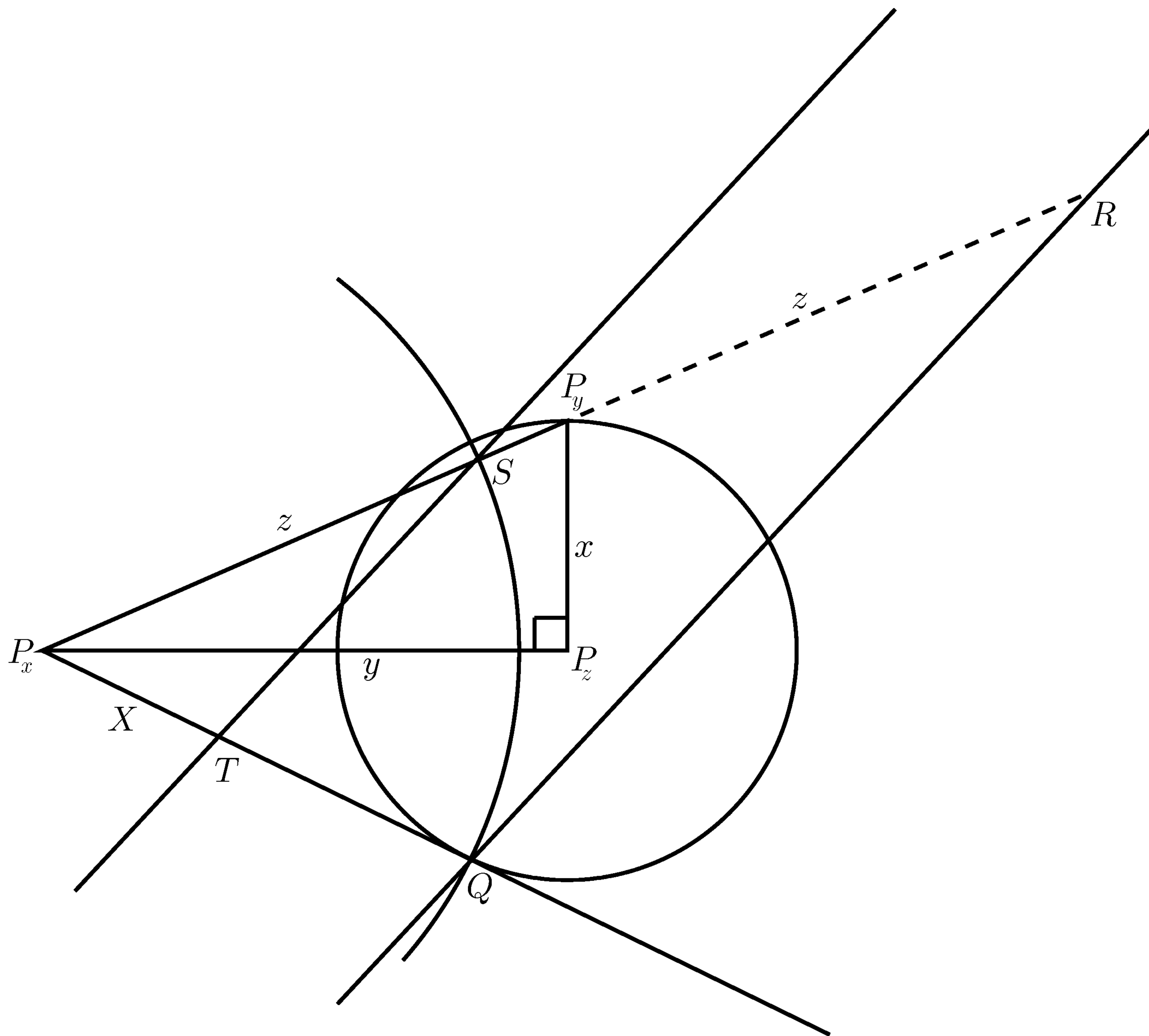
Figure 5.4. Constructing a new Pythagorean triple.
