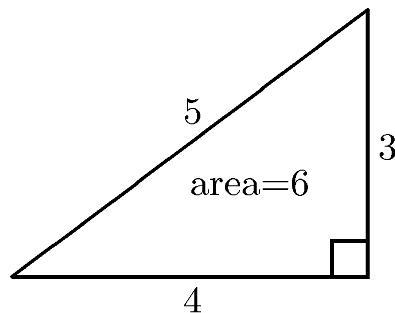
Figure 5.3. Six is a congruent number.
