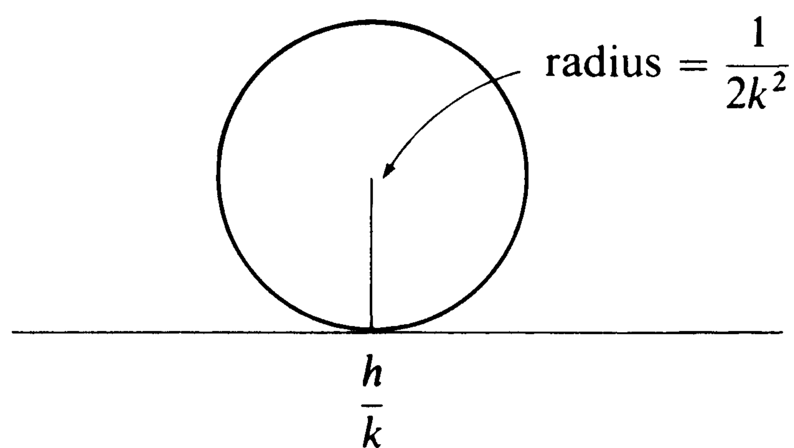
Figure 5.1 The Ford circle C(h, k)
