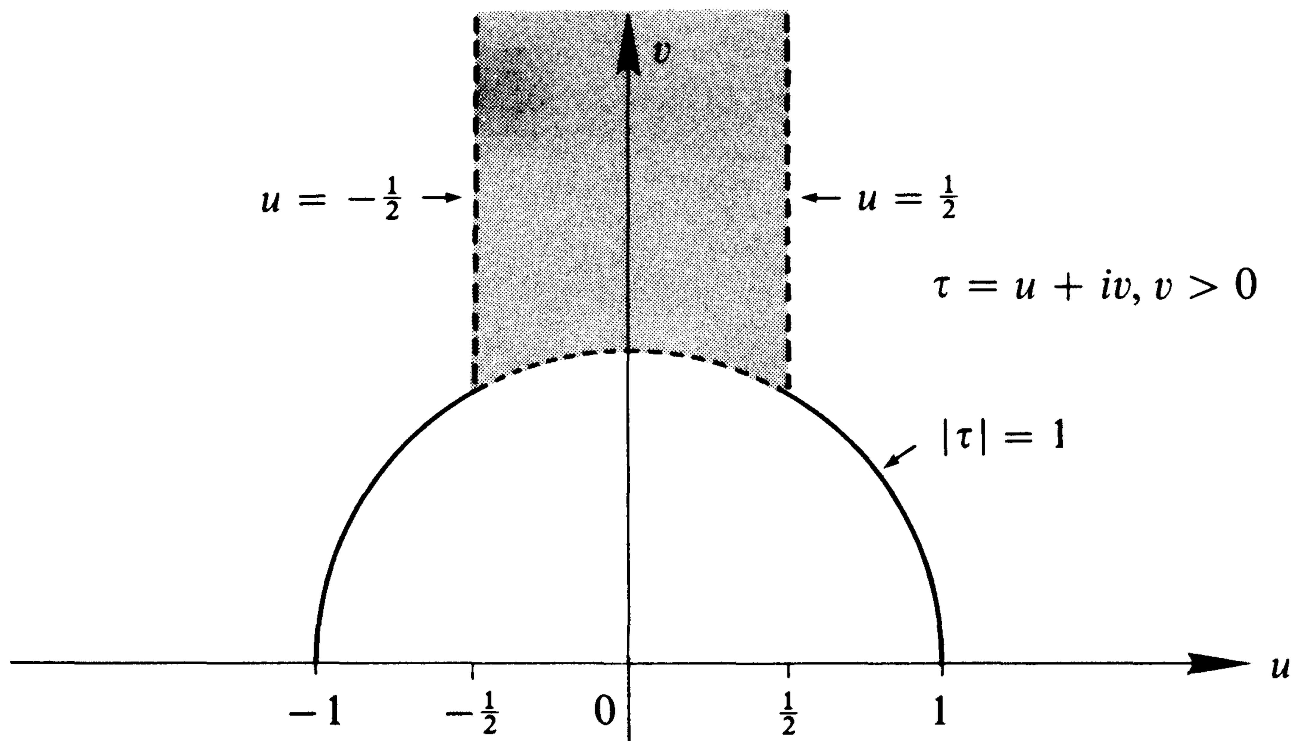
Figure 2.1 Fundamental region of the modular group
