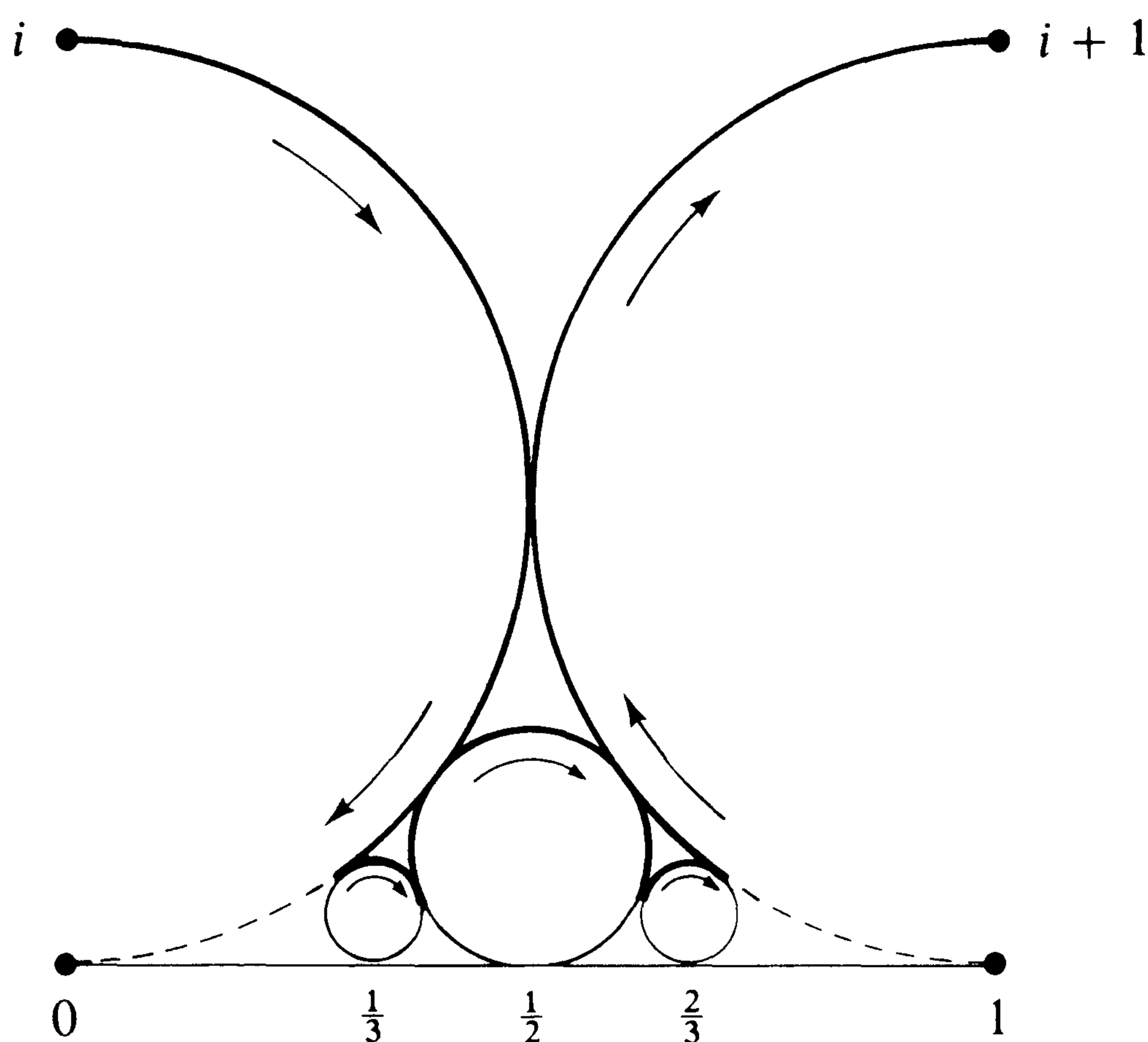
Figure 5.5 The Rademacher path P(3)
