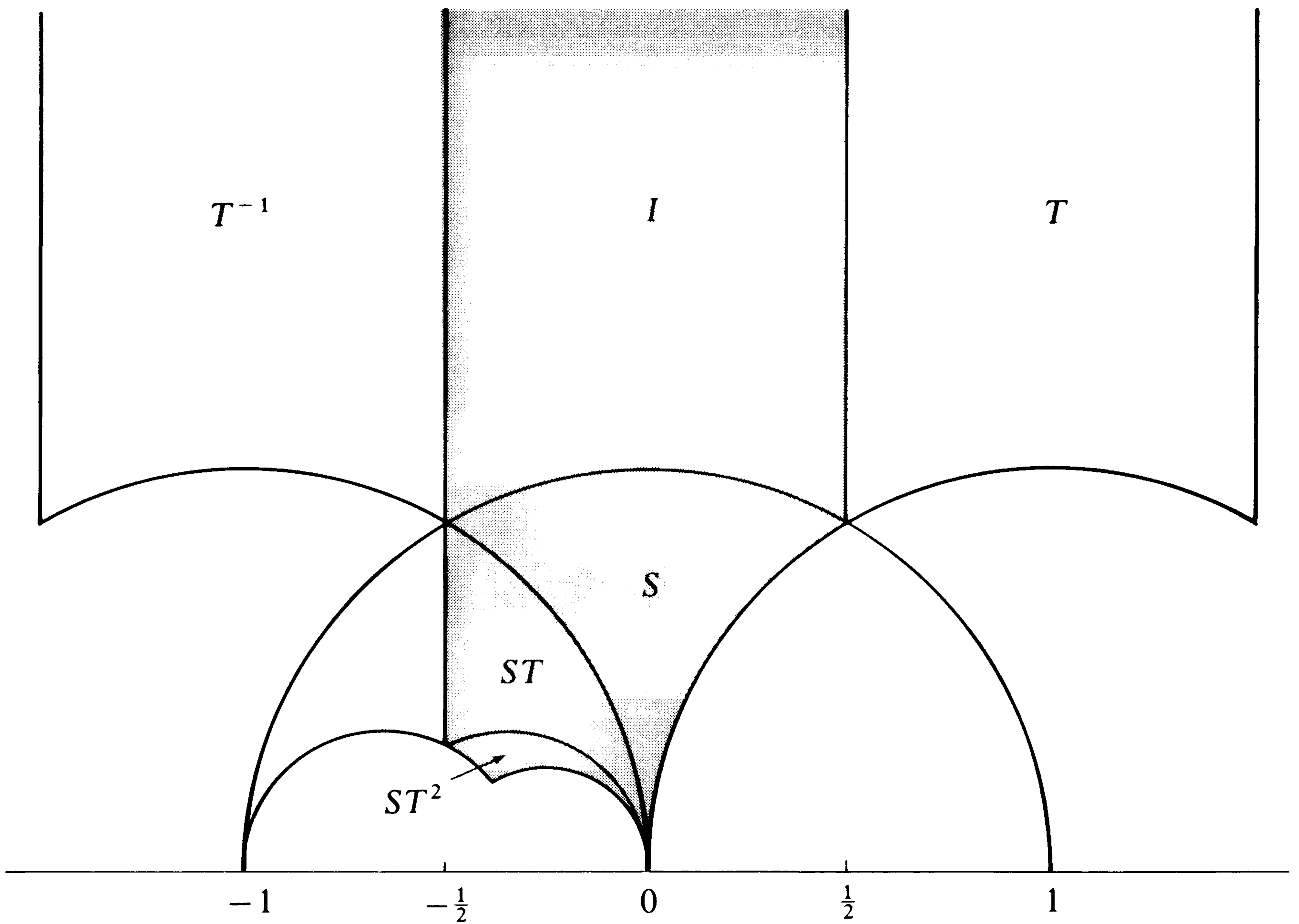
Figure 4.1 Fundamental region for \Gamma_0(3)
