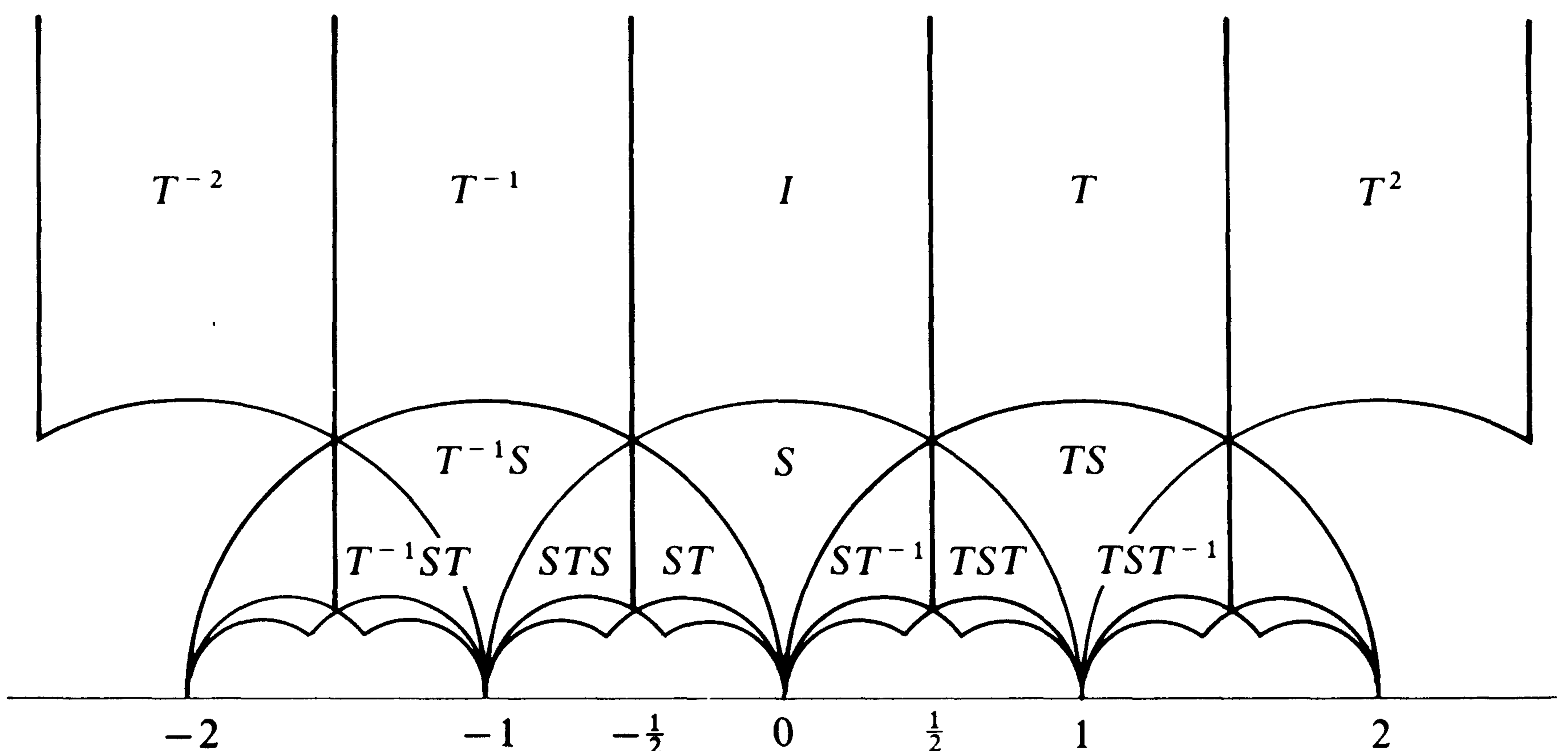
Figure 2.2 Images of the fundamental region R_\Gamma under elements of \Gamma
